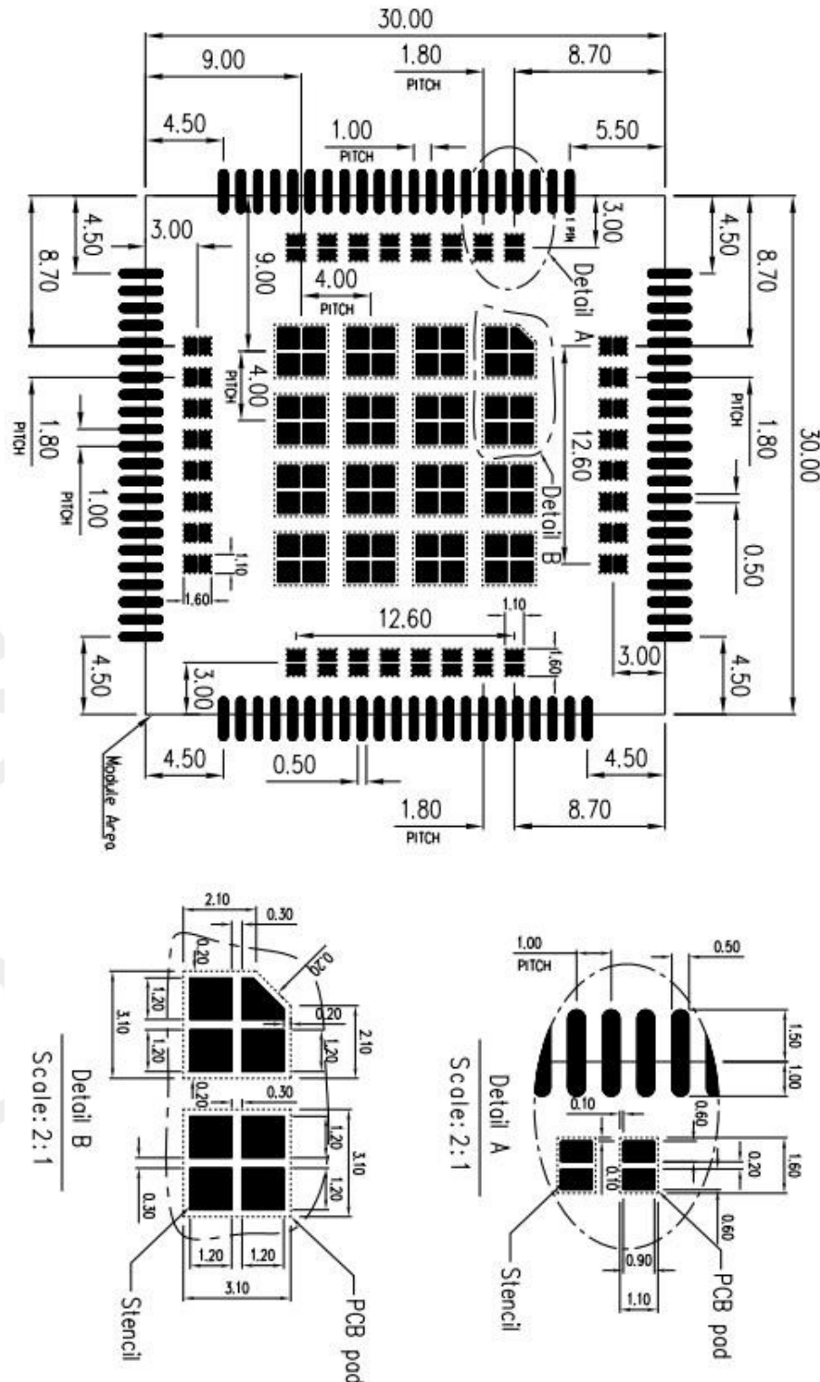
Figure 42 : Stencil Foil
