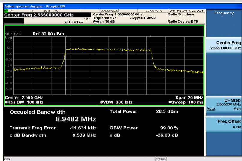
Band7-10MHz-16QAM-21400-50RB#0-8.9482
