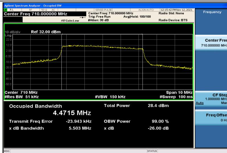
Band17-5MHz-16QAM-23790-25RB#0-4.4715
