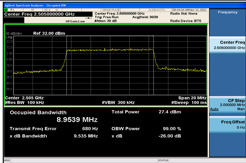
Band7-10MHz-16QAM-20800-50RB#0-8.9539
