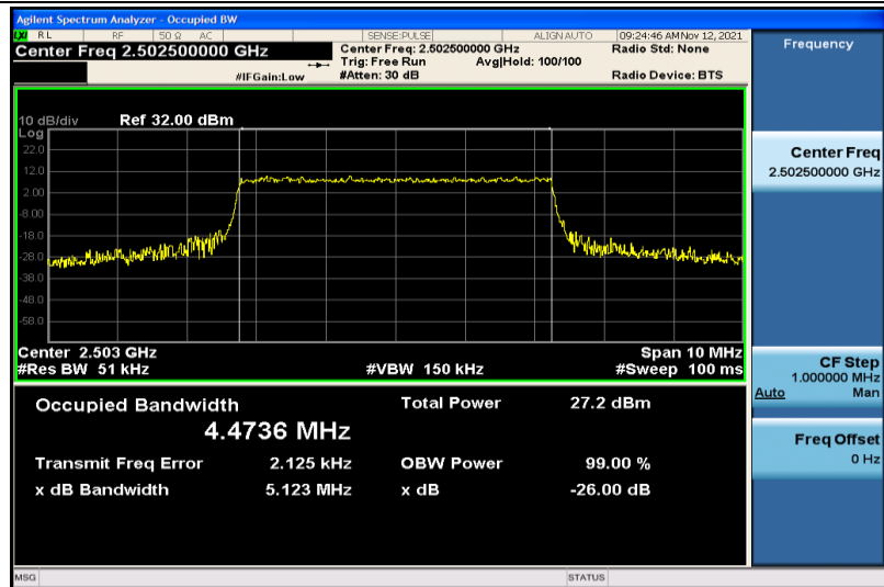
Band7-5MHz-16QAM-20775-25RB#0-4.4736
