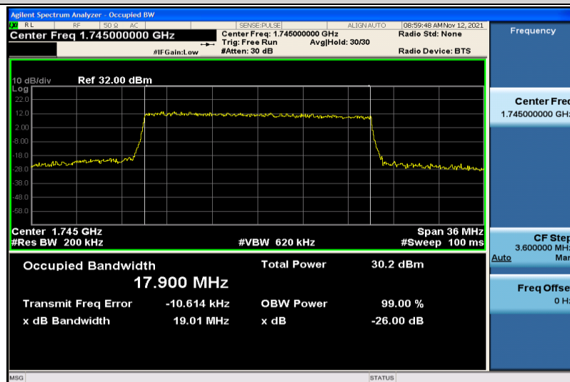
Band4-20MHz-16QAM-20300-100RB#0-17.900
