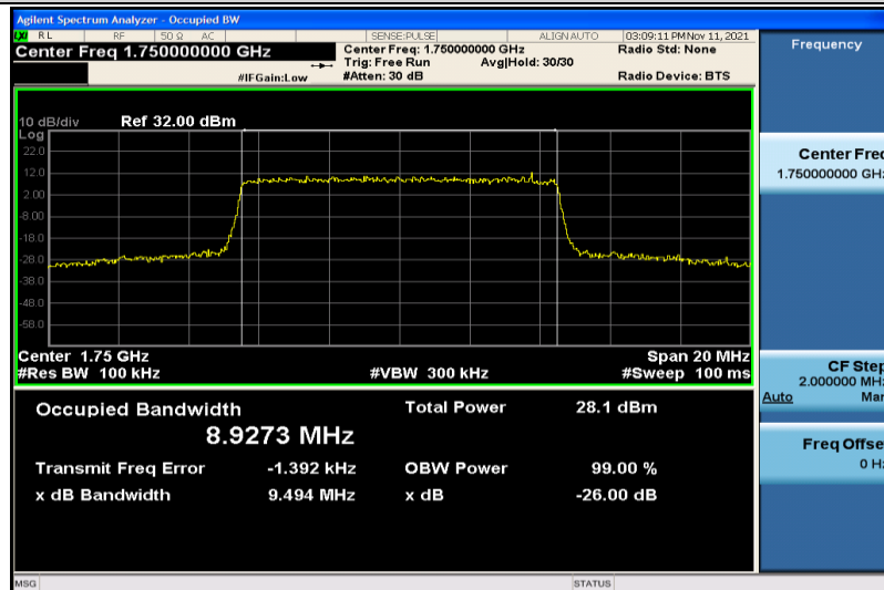
Band4-10MHz-16QAM-20350-50RB#0-8.9273
