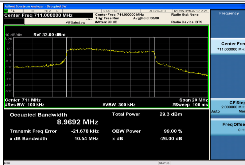
Band17-10MHz-QPSK-23800-50RB#0-8.9692
