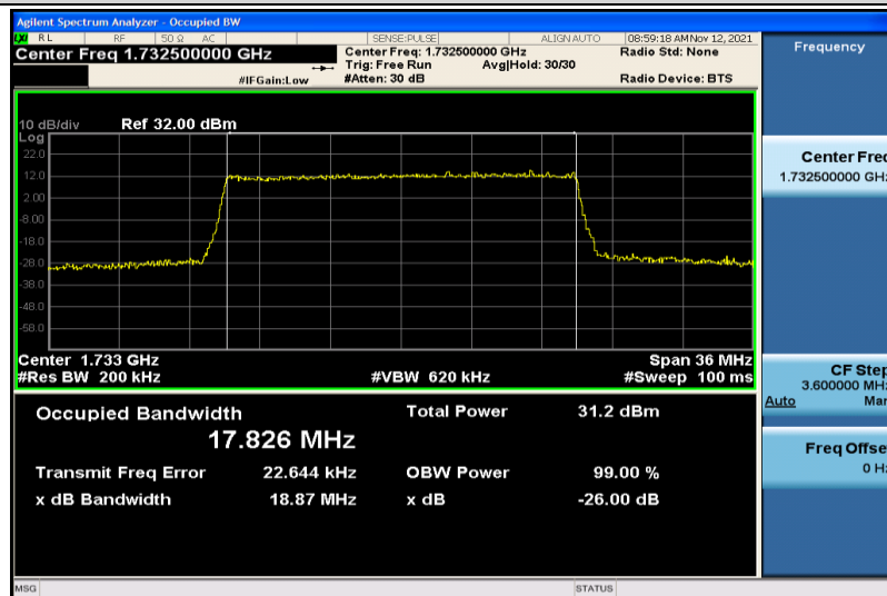
Band4-20MHz-QPSK-20175-100RB#0-17.826
