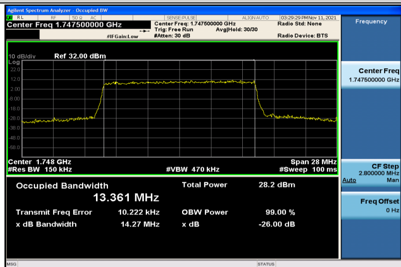
Band4-15MHz-16QAM-20325-75RB#0-13.361
