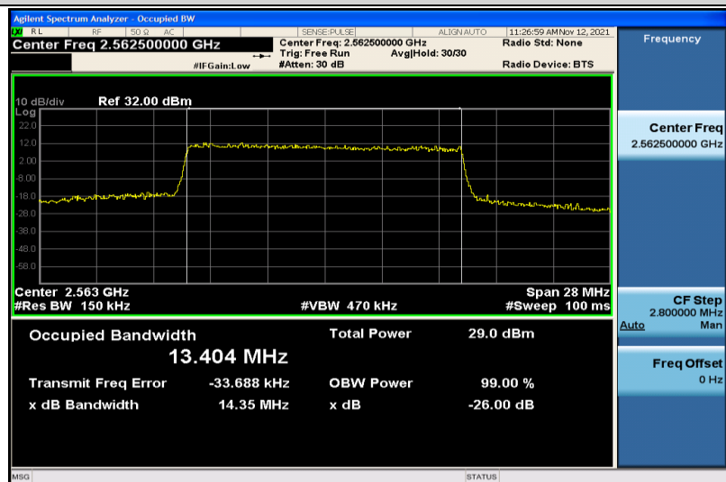
Band7-15MHz-QPSK-21375-75RB#0-13.404
