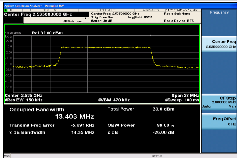
Band7-15MHz-QPSK-21100-75RB#0-13.403
