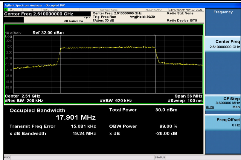
Band7-20MHz-QPSK-20850-100RB#0-17.901
