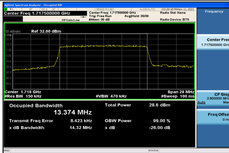
Band4-15MHz-QPSK-20025-75RB#0-13.374
