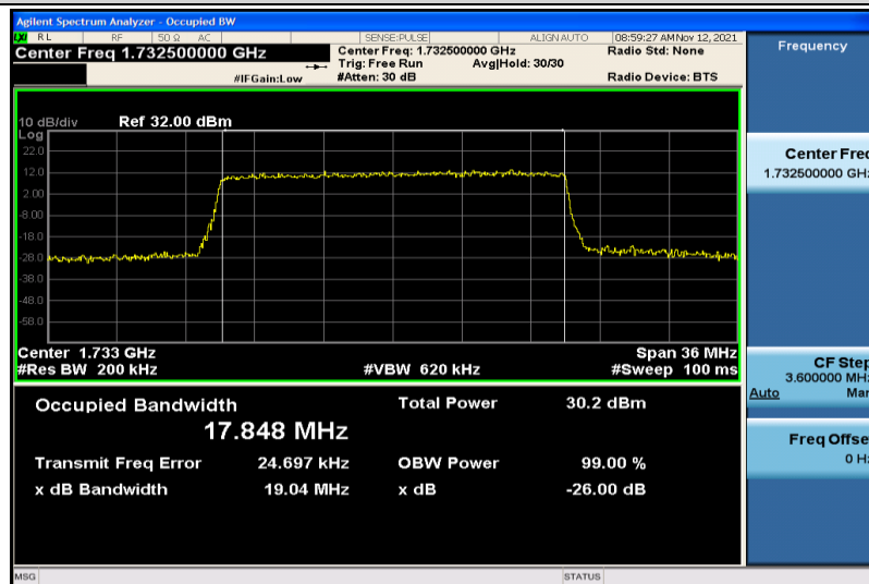
Band4-20MHz-16QAM-20175-100RB#0-17.848
