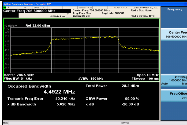
Band17-5MHz-16QAM-23755-25RB#0-4.4922
