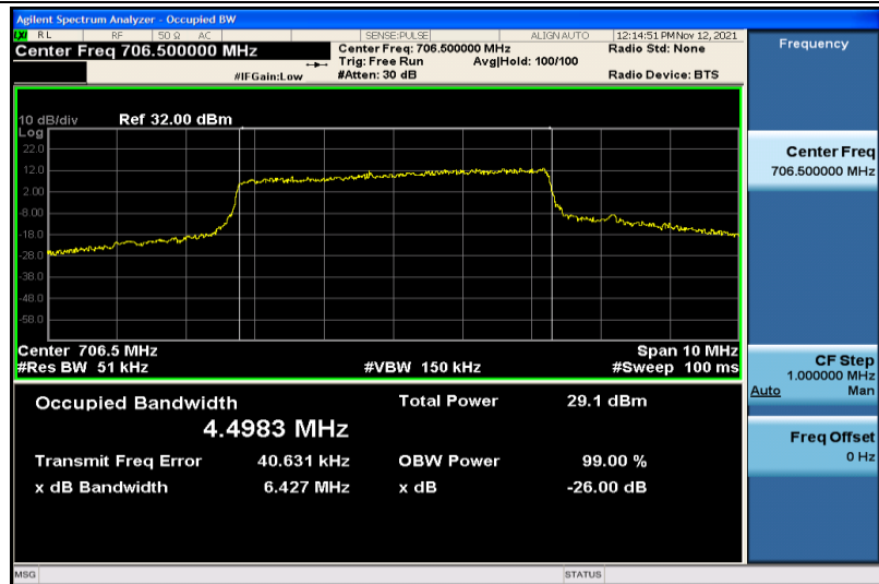
Band17-5MHz-QPSK-23755-25RB#0-4.4983
