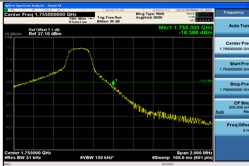
Band4-5MHz-16QAM-20375-1RB#24
