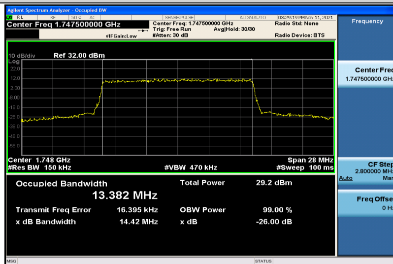
Band4-15MHz-QPSK-20325-75RB#0-13.382
