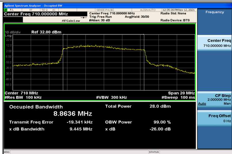
Band17-10MHz-16QAM-23790-50RB#0-8.8636
