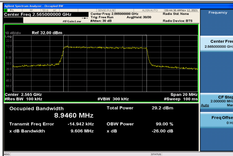
Band7-10MHz-QPSK-21400-50RB#0-8.9460
