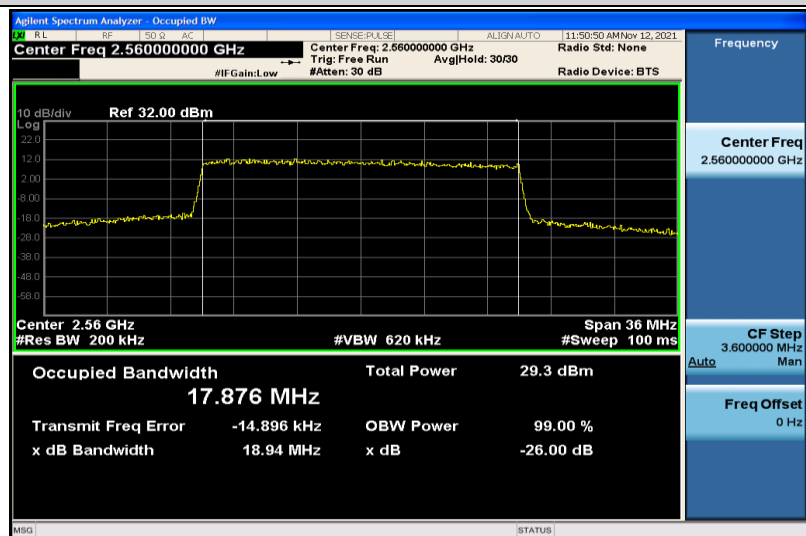
Band7-20MHz-16QAM-21350-100RB#0-17.876
