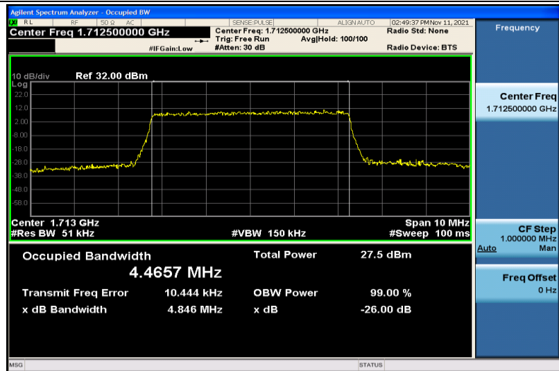
Band4-5MHz-16QAM-19975-25RB#0-4.4657
