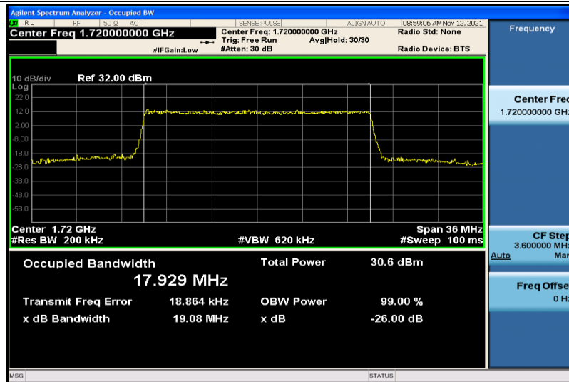
Band4-20MHz-16QAM-20050-100RB#0-17.929
