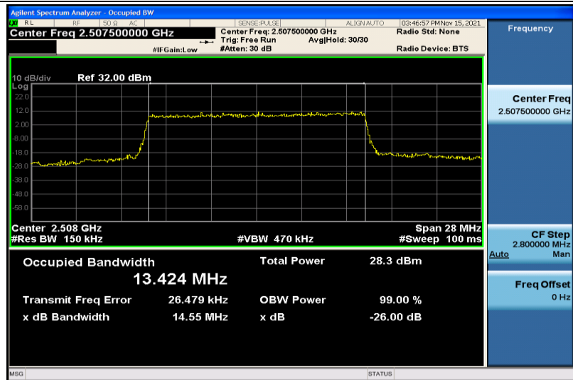
Band7-15MHz-QPSK-20825-75RB#0-13.424
