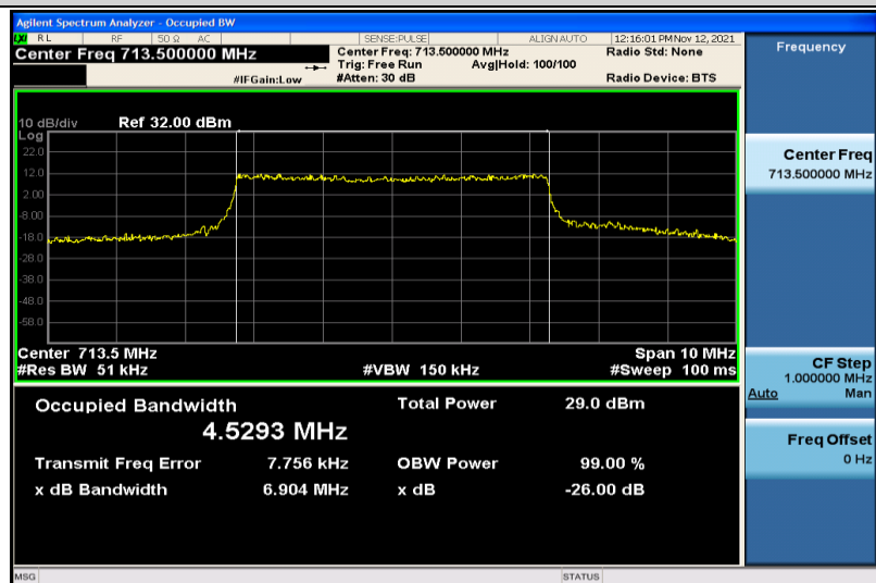
Band17-5MHz-QPSK-23825-25RB#0-4.5293
