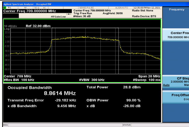
Band17-10MHz-QPSK-23780-50RB#0-8.8614
