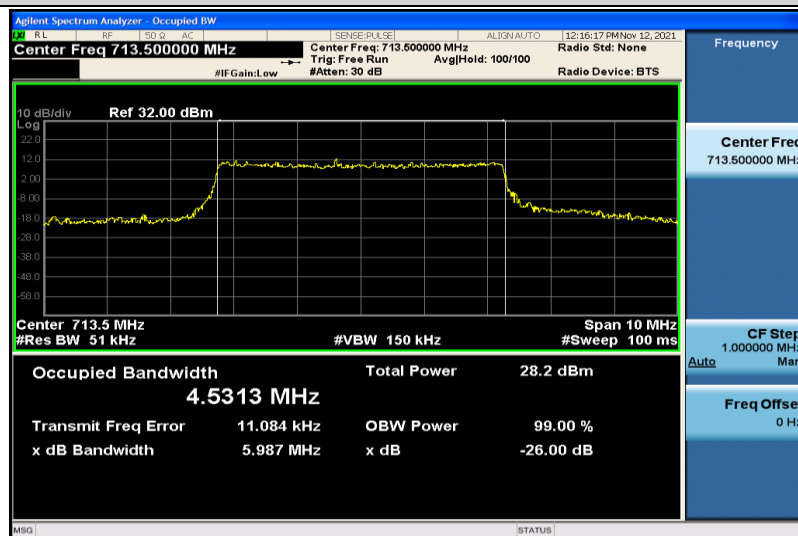
Band17-5MHz-16QAM-23825-25RB#0-4.5313
