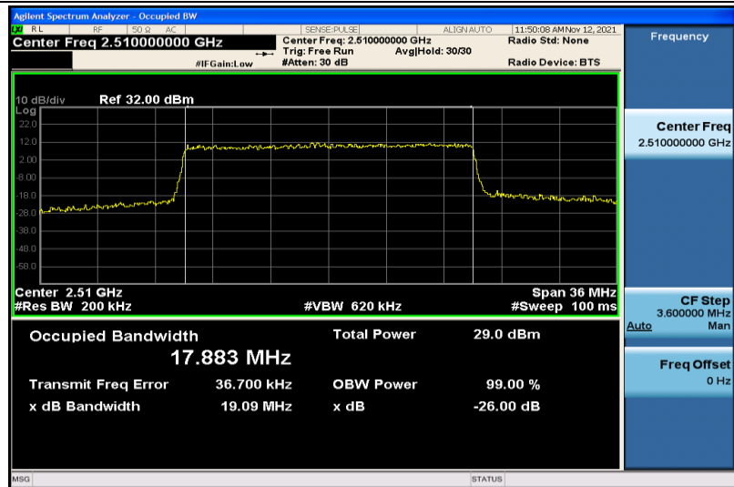
Band7-20MHz-16QAM-20850-100RB#0-17.883
