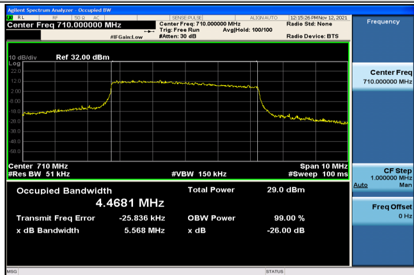
Band17-5MHz-QPSK-23790-25RB#0-4.4681
