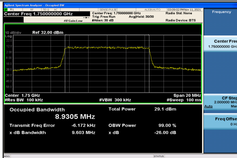
Band4-10MHz-QPSK-20350-50RB#0-8.9305
