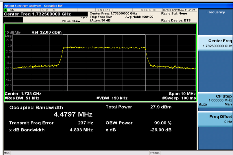
Band4-5MHz-16QAM-20175-25RB#0-4.4797
