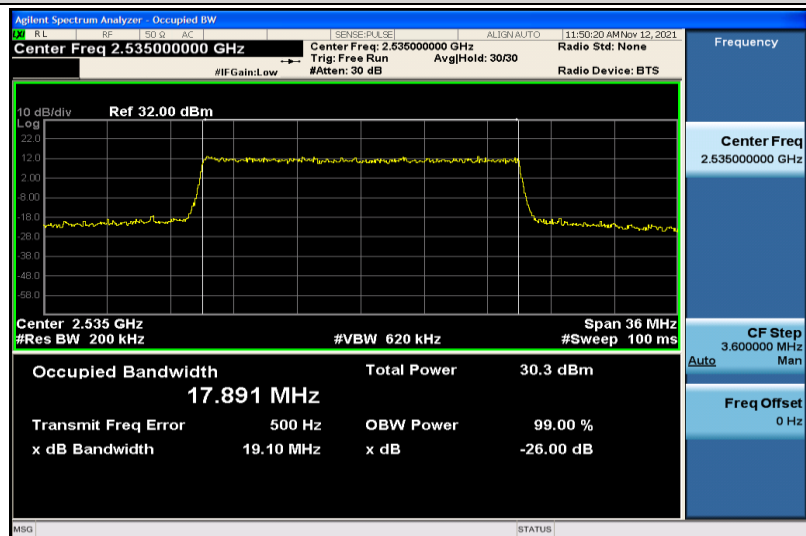
Band7-20MHz-QPSK-21100-100RB#0-17.891
