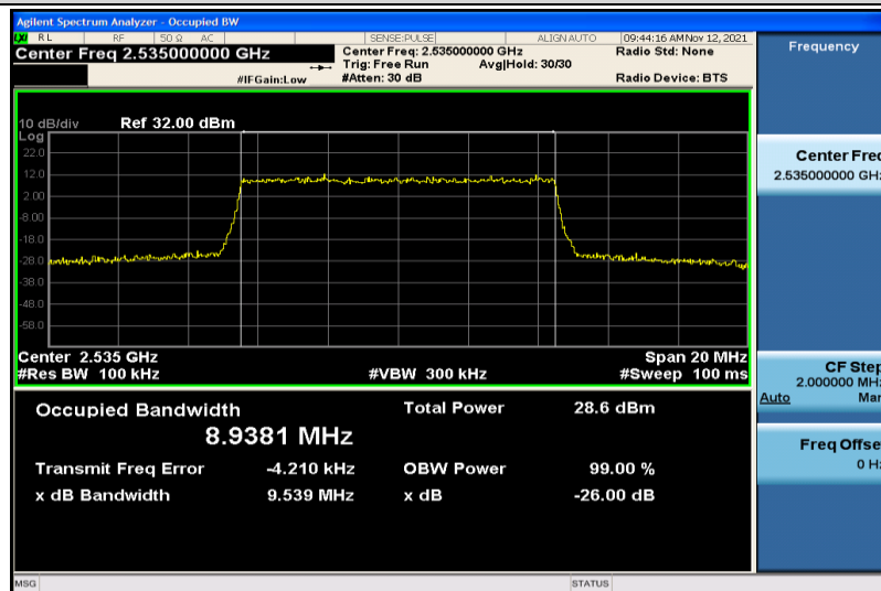
Band7-10MHz-QPSK-21100-50RB#0-8.9381
