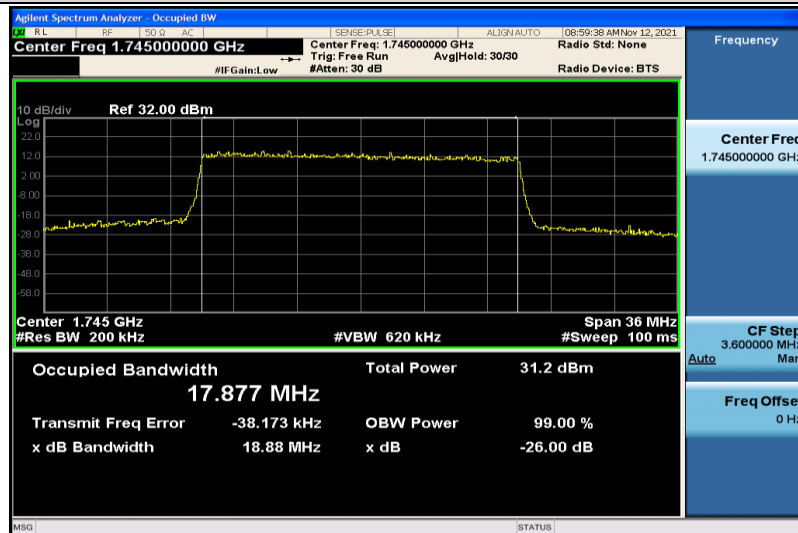
Band4-20MHz-QPSK-20300-100RB#0-17.877
