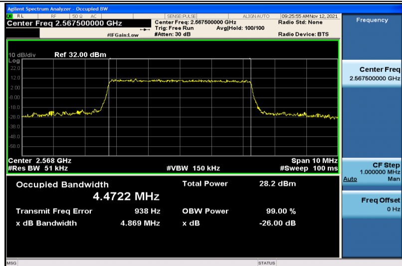
Band7-5MHz-16QAM-21425-25RB#0-4.4722
