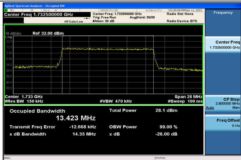
Band4-15MHz-16QAM-20175-75RB#0-13.423
