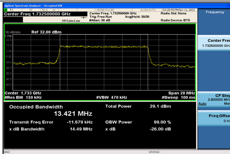
Band4-15MHz-QPSK-20175-75RB#0-13.421
