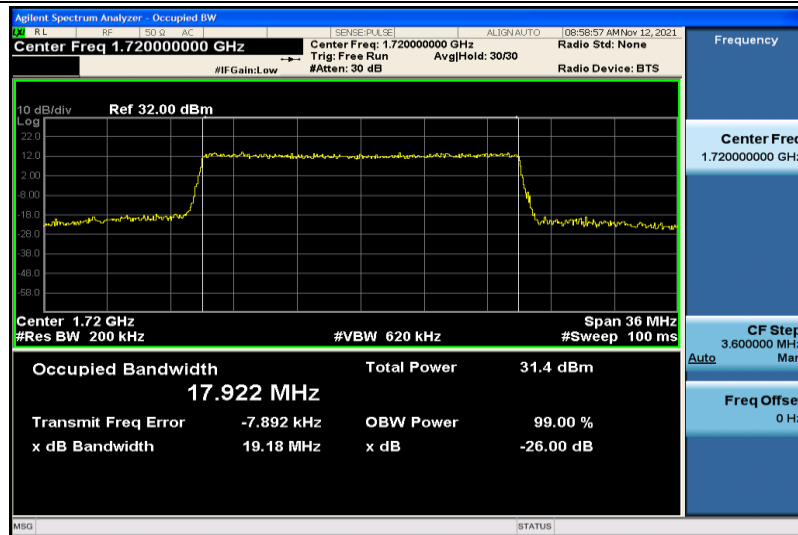
Band4-20MHz-QPSK-20050-100RB#0-17.922
