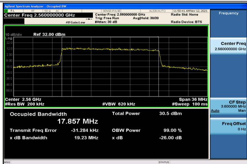
Band7-20MHz-QPSK-21350-100RB#0-17.857
