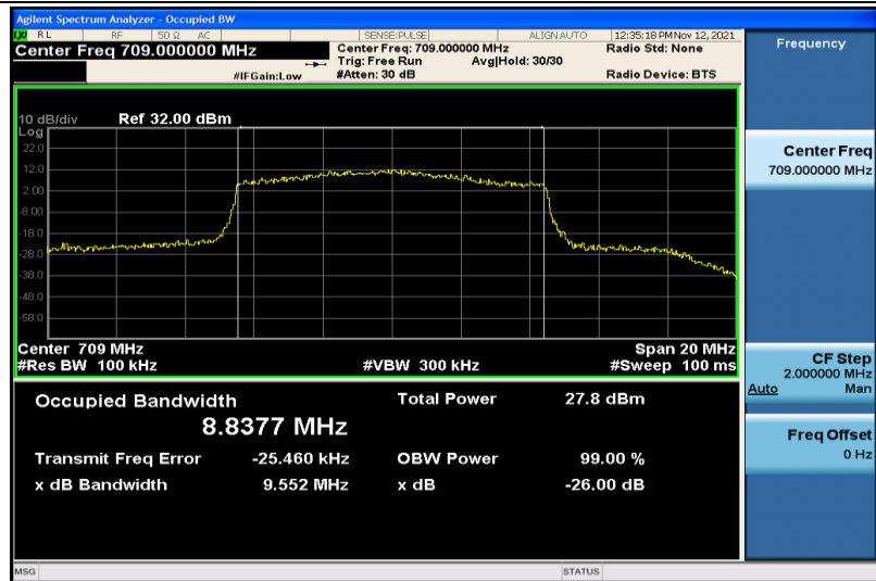
Band17-10MHz-16QAM-23780-50RB#0-8.8377
