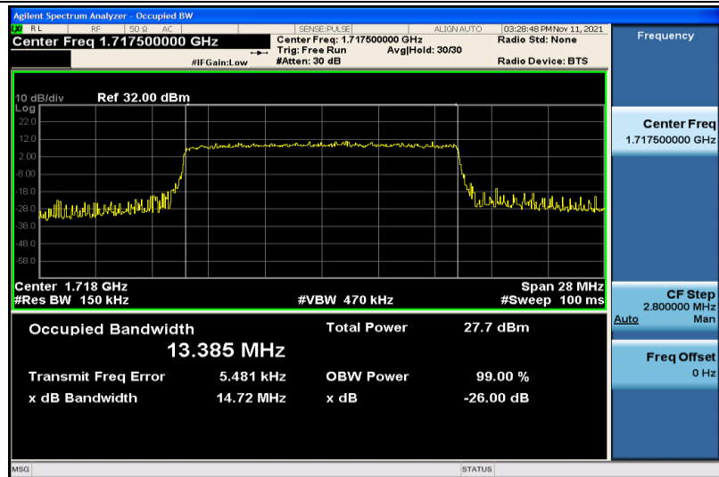
Band4-15MHz-16QAM-20025-75RB#0-13.385
