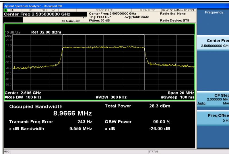
Band7-10MHz-QPSK-20800-50RB#0-8.9666
