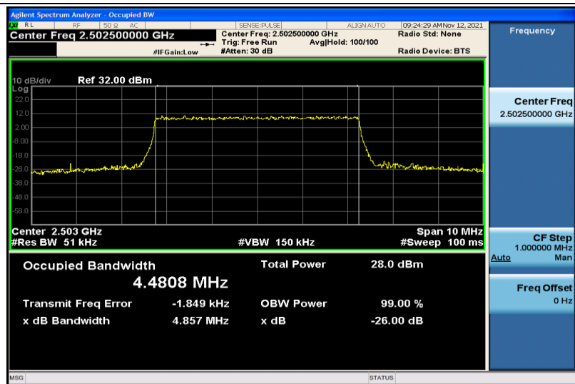
Band7-5MHz-QPSK-20775-25RB#0-4.4808
