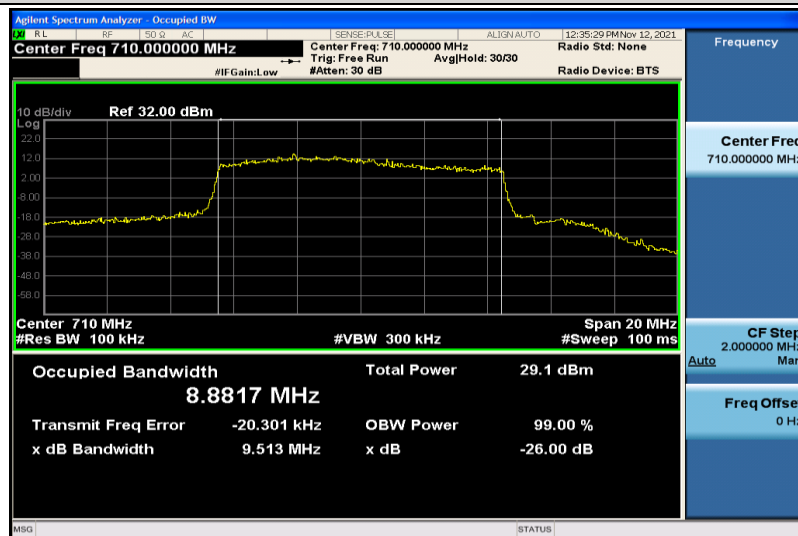
Band17-10MHz-QPSK-23790-50RB#0-8.8817
