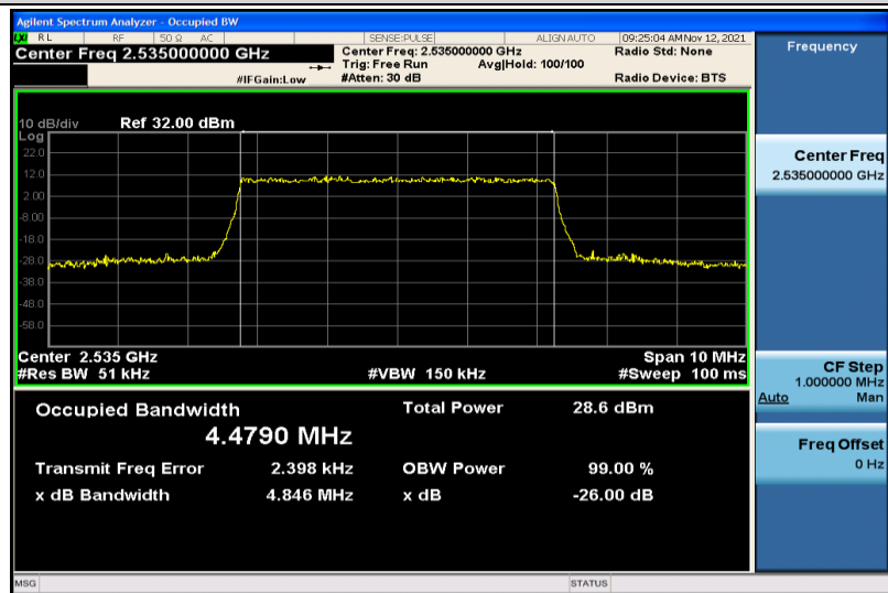
Band7-5MHz-QPSK-21100-25RB#0-4.4790
