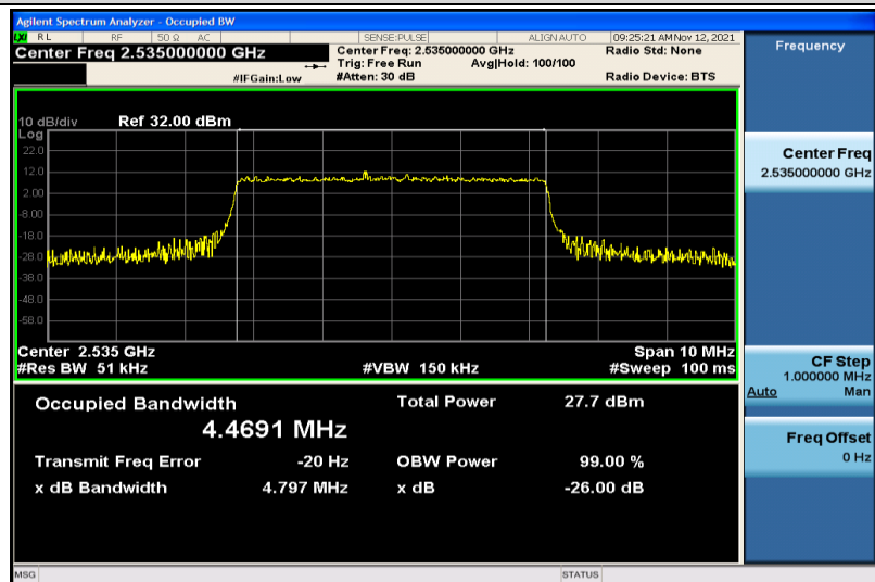
Band7-5MHz-16QAM-21100-25RB#0-4.4691
