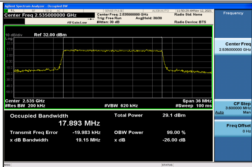
Band7-20MHz-16QAM-21100-100RB#0-17.893
