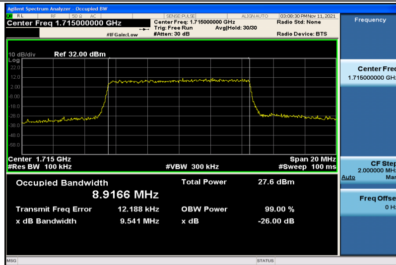
Band4-10MHz-16QAM-20000-50RB#0-8.9166
