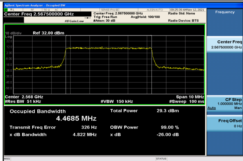
Band7-5MHz-QPSK-21425-25RB#0-4.4685
