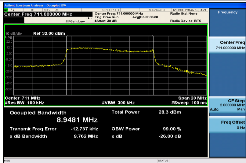
Band17-10MHz-16QAM-23800-50RB#0-8.9481
