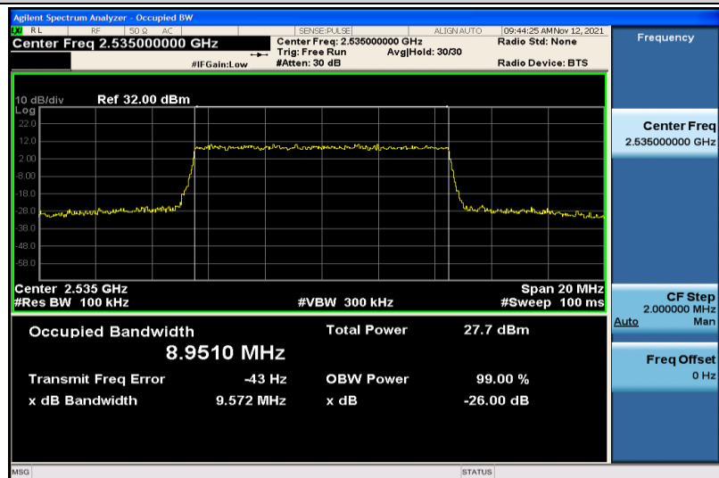
Band7-10MHz-16QAM-21100-50RB#0-8.9510
