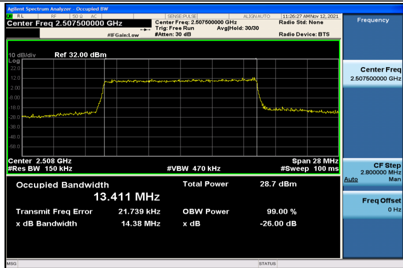
Band7-15MHz-16QAM-20825-75RB#0-13.411
