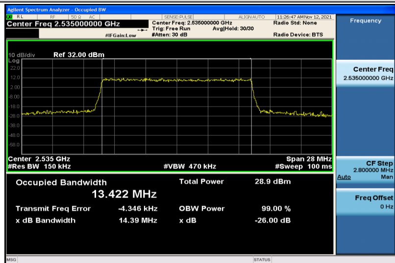
Band7-15MHz-16QAM-21100-75RB#0-13.422
