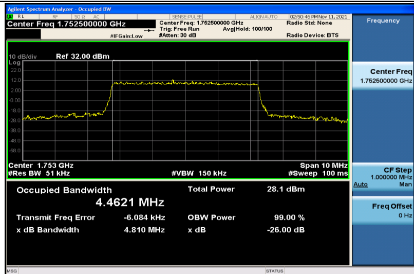
Band4-5MHz-16QAM-20375-25RB#0-4.4621
