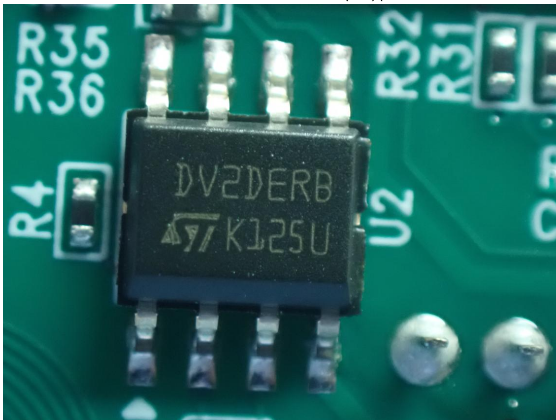
Figure 18 NFC IC (U2)(ST ST25DV04K-IER6S3) View
