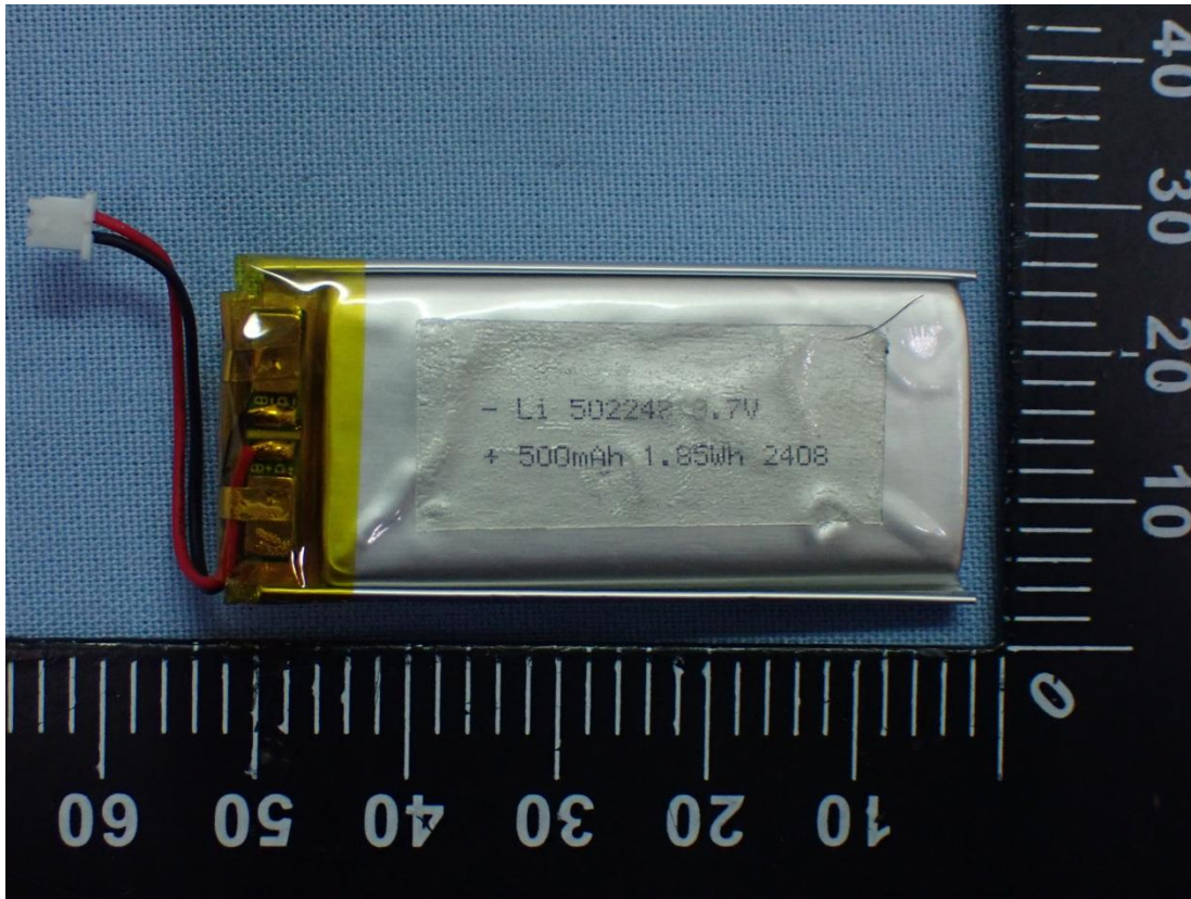
Figure 11 Battery (Front View)
