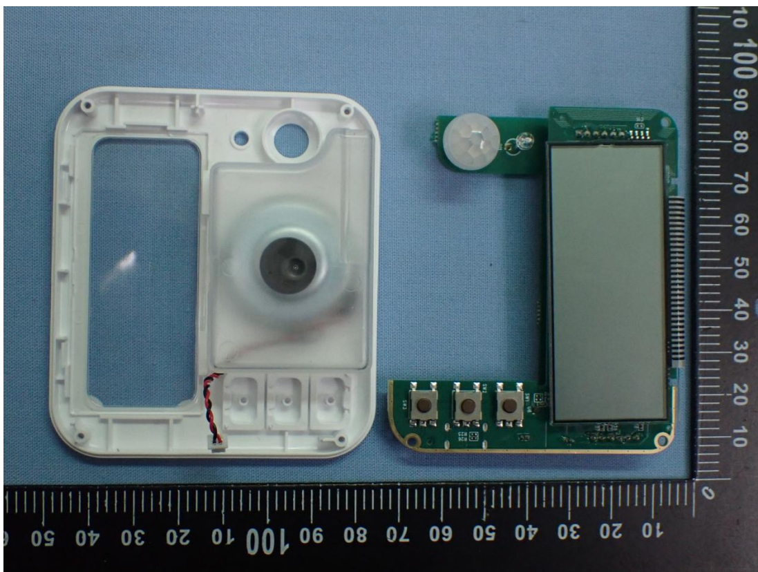
Figure 8 Internal View
