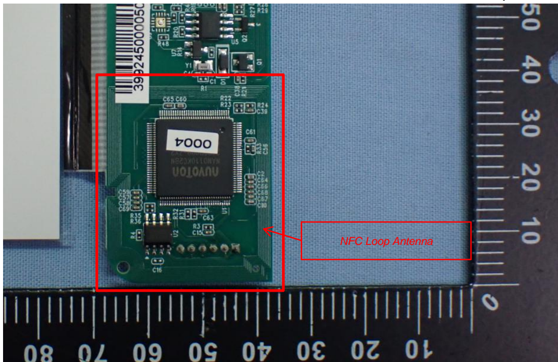
Figure 17 NFC Loop Antenna View
