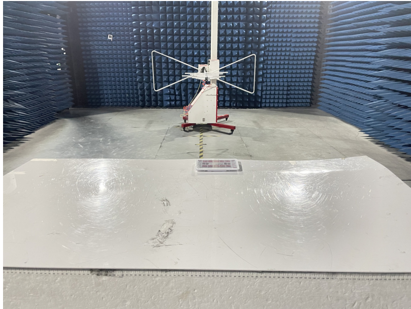
Test Model No.: Stellar Pro-750R-N Radiated Emission
