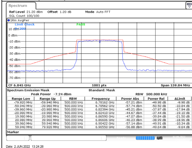
802.11ax (40MHz) / 6845MHz / Chain A / NSS-4
