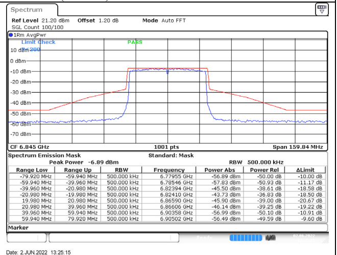
802.11ax (40MHz) / 6845MHz / Chain B / NSS-4
