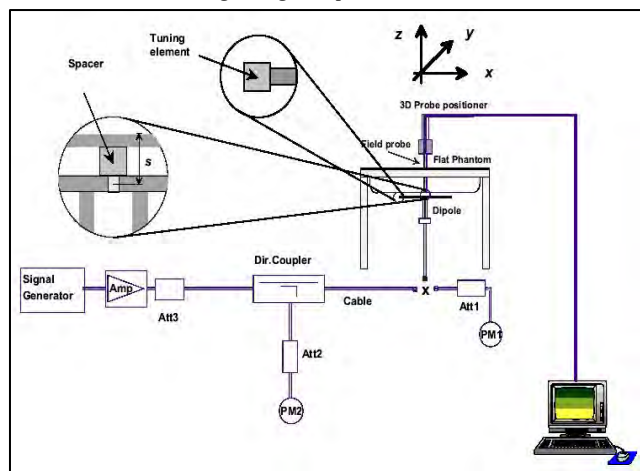
Test setup for the system performance check
