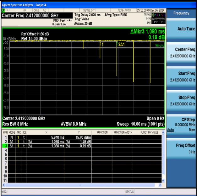
NTNV-11AX20SISO-Ant1-2412
