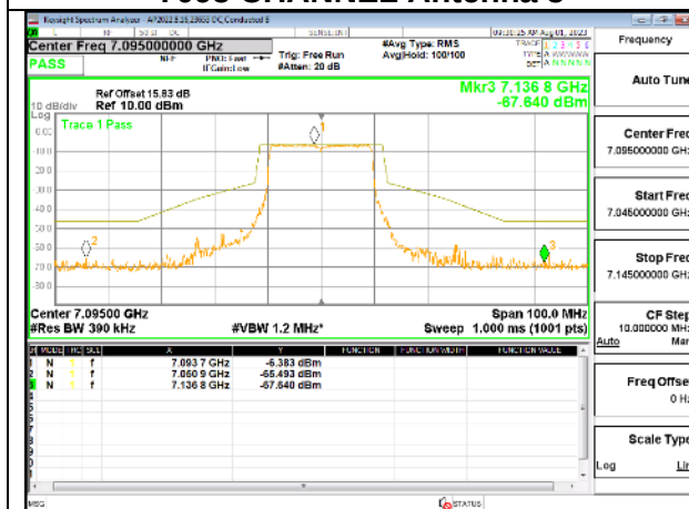
7095 CHANNEL Antenna 3
