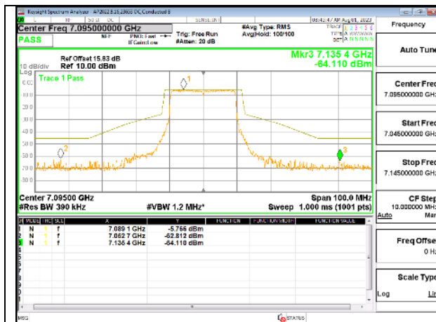
7095 CHANNEL Antenna 5
