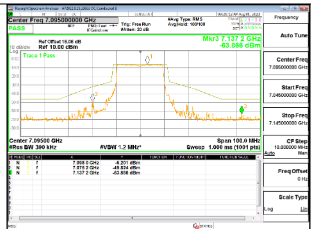
7095 CHANNEL Antenna 8
