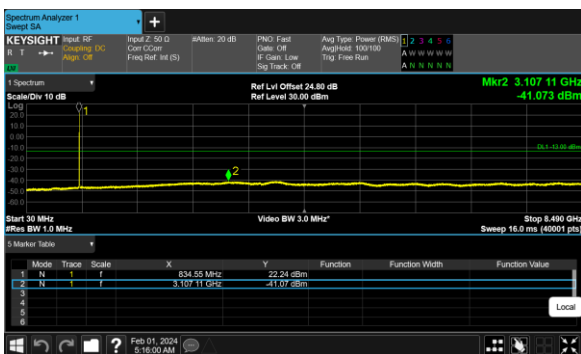
N26(5M)_DFT-s- OFDM_BPSK_Edge_1RB_Left_High_CH
