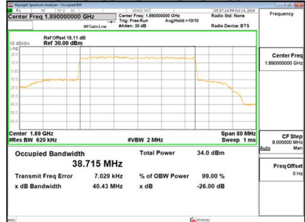
Band2_40MHz_DFT_s_OFDM_SCS15kHz_BPSK_RB216_0_CH378000
