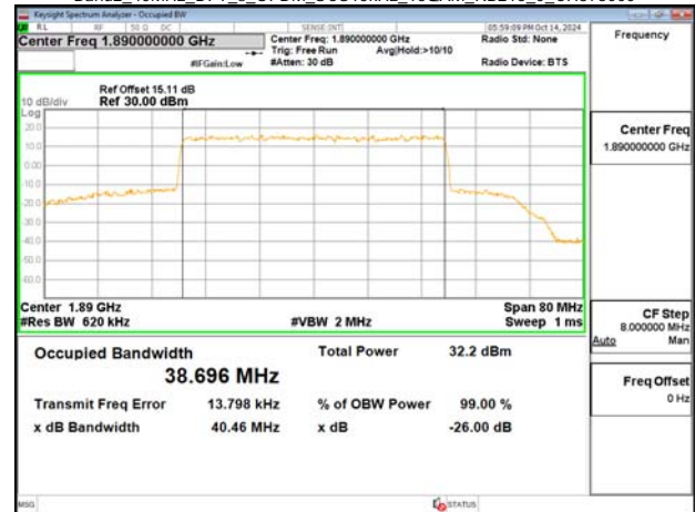
Band2_40MHz_DFT_s_OFDM_SCS15kHz_16QAM_RB216_0_CH378000
