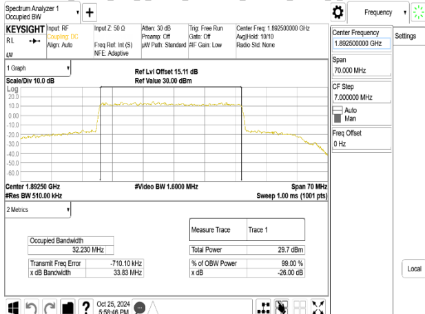
Band2_35MHz_DFT_s_OFDM_SCS15kHz_256QAM_RB180_0_CH378500
