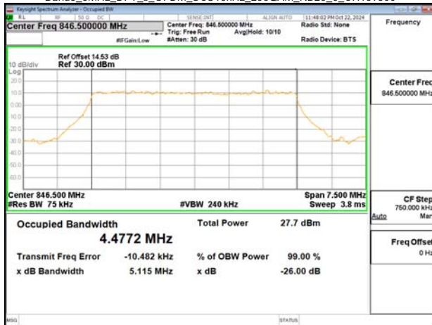
Band5_5MHz_DFT_s_OFDM_SCS15kHz_256QAM_RB25_0_CH169300
