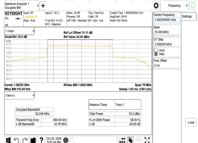
Band2_35MHz_DFT_s_OFDM_SCS15kHz_QPSK_RB180_0_CH378500
