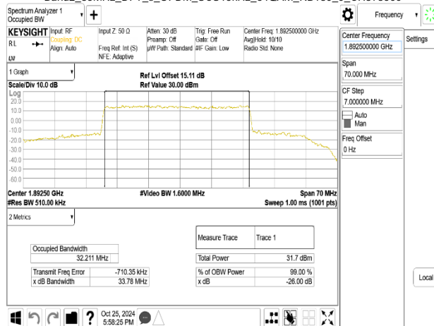
Band2_35MHz_DFT_s_OFDM_SCS15kHz_64QAM_RB180_0_CH378500
