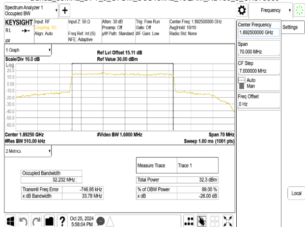
Band2_35MHz_DFT_s_OFDM_SCS15kHz_16QAM_RB180_0_CH378500
