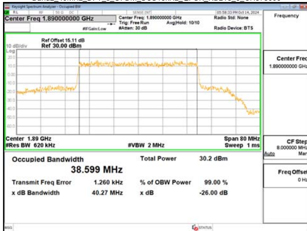
Band2_40MHz_DFT_s_OFDM_SCS15kHz_QPSK_RB216_0_CH378000
