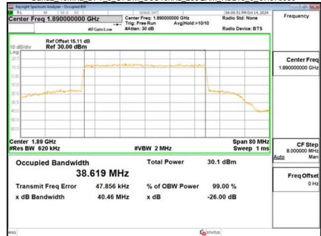
Band2_40MHz_DFT_s_OFDM_SCS15kHz_256QAM_RB216_0_CH378000
