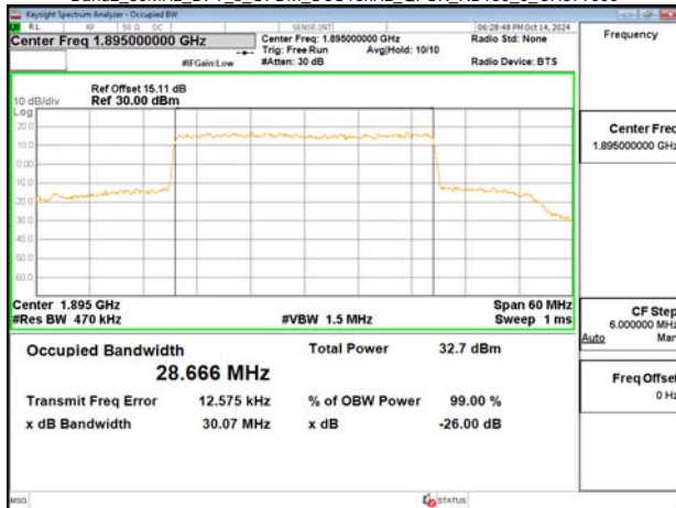
Band2_30MHz_DFT_s_OFDM_SCS15kHz_QPSK_RB160_0_CH379000
