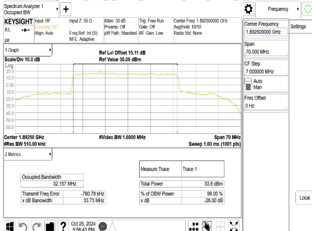
Band2_35MHz_DFT_s_OFDM_SCS15kHz_BPSK_RB180_0_CH378500
