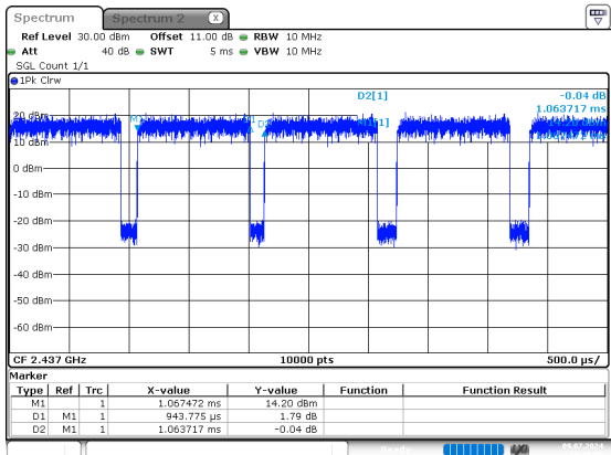
n40_2437MHz_Chain 0
