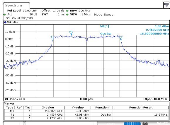
g_2462MHz_Chain 0
