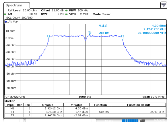
n40_2422MHz_Chain 0
