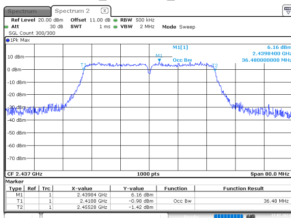
n40_2437MHz_Chain 0
