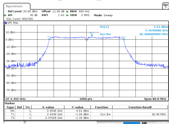
n40_2452MHz_Chain 0
