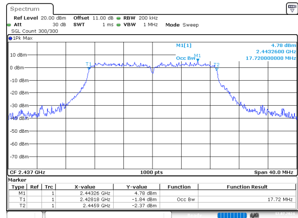
n20_2437MHz_Chain 0
