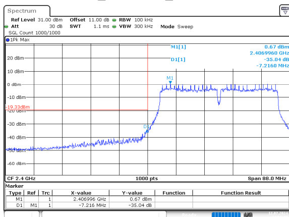
n40_2422MHz_Chain 0
