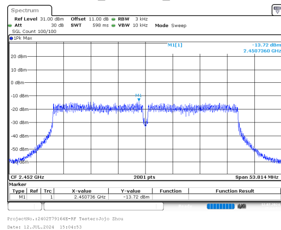
n40_2452MHz_Chain 0
