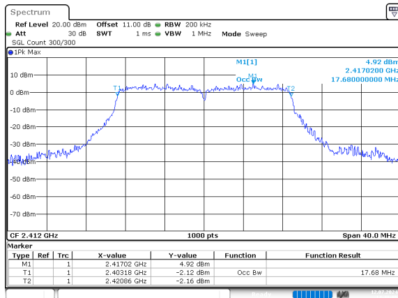
n20_2412MHz_Chain 0
