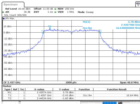
g_2437MHz_Chain 0
