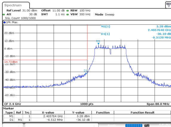
g_2412MHz_Chain 0
