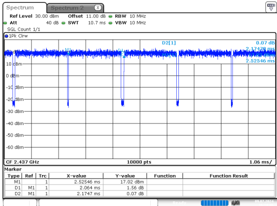
g_2437MHz_Chain 0
