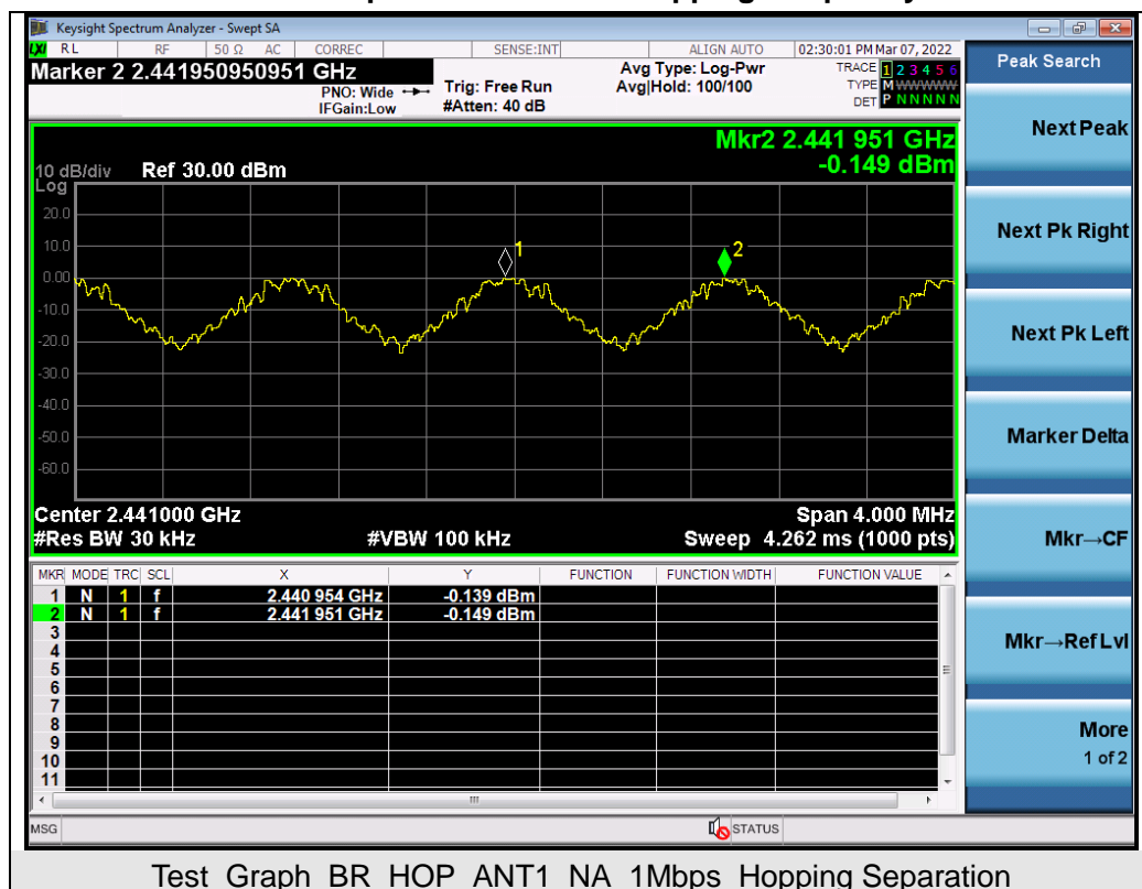
Test_Graph_BR_HOP_ANT1_NA_1Mbps_Hopping Separation
