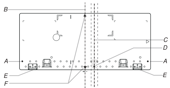
No Wall Studs at End Holes Figure 2
