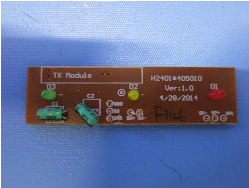
Main PCB comp side (2)
