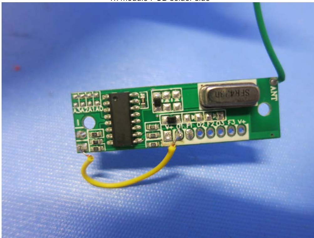
Tx module PCB solder side
