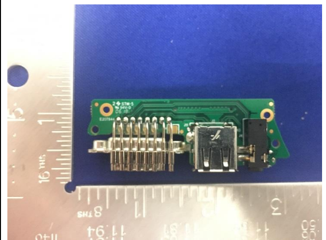
Port board – Rear view
