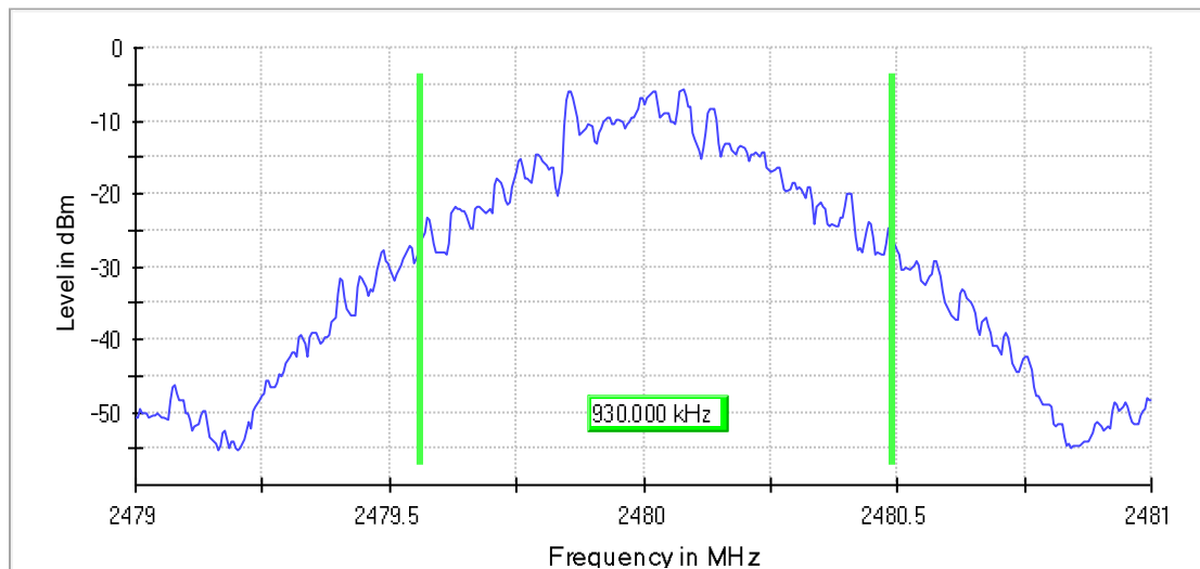
20 dB Bandwidth
