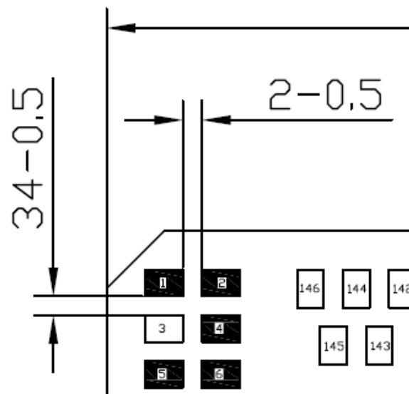
Figure 11. PCBA dimensions
