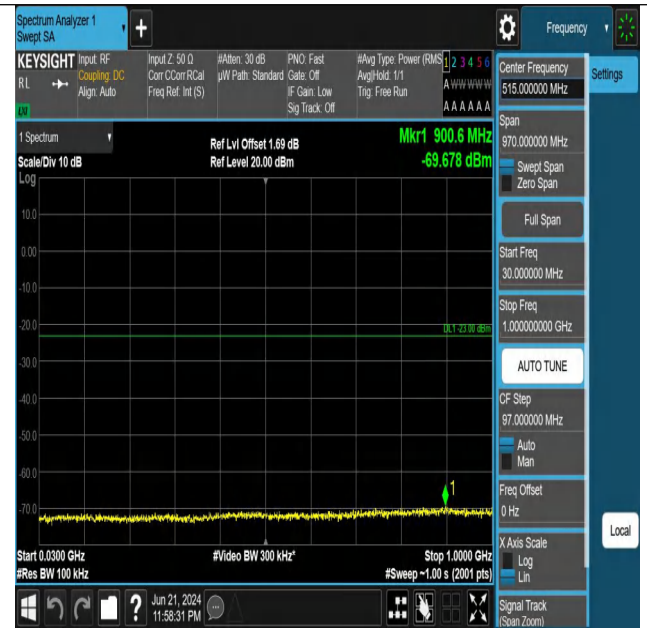
Band2_1.4MHz_QPSK_18900_1RB#5_30~1000_30~1000
