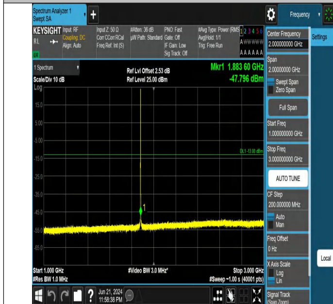
Band2_1.4MHz_QPSK_18900_1RB#5_1000~3000_1000~3000
