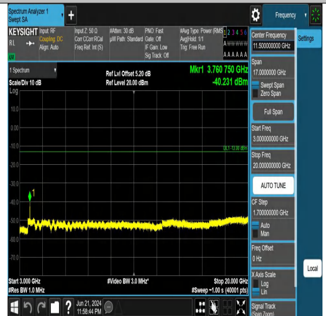
Band2_1.4MHz_QPSK_18900_1RB#5_3000~20000_3000~20000
