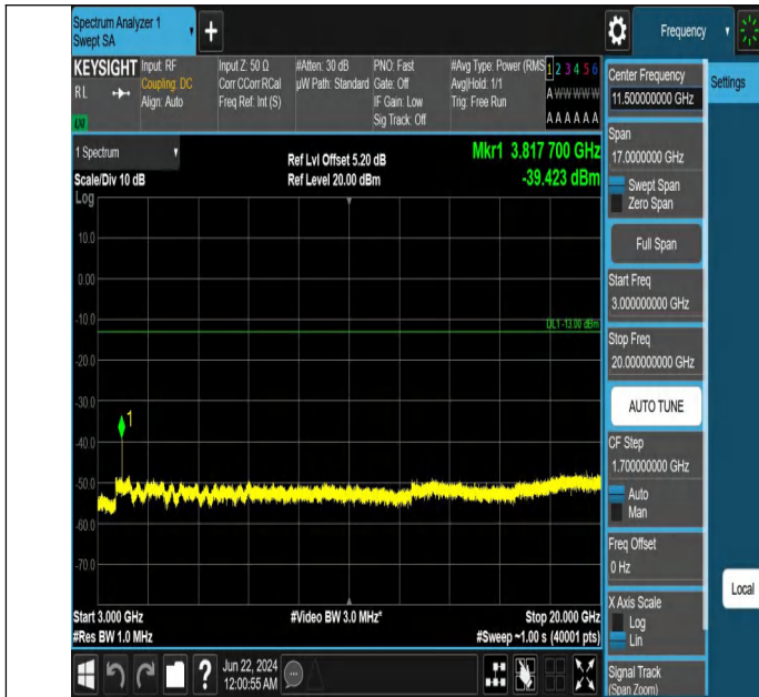
Band2_1.4MHz_QPSK_19193_1RB#0_3000~20000_3000~20000
