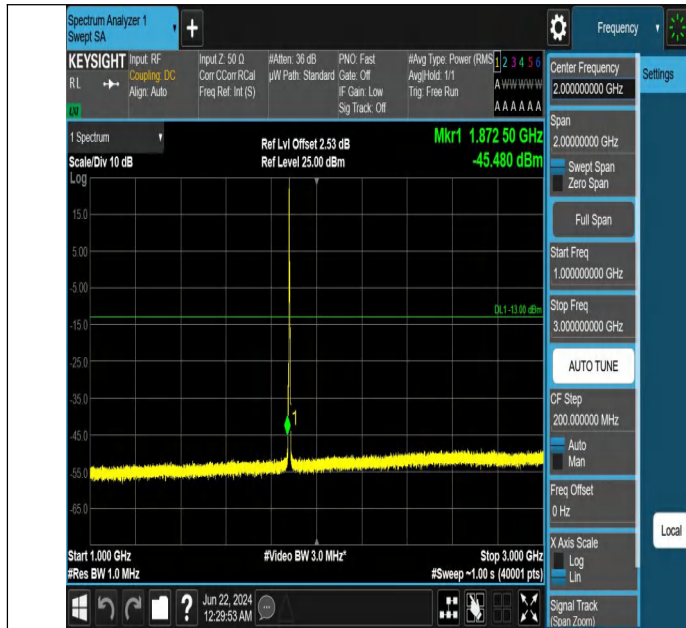
Band2_3MHz_QPSK_18900_1RB#0_1000~3000_1000~3000
