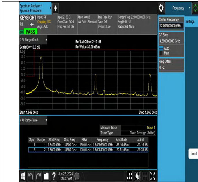
Band2_15MHz_QPSK_18675_1RB#0
