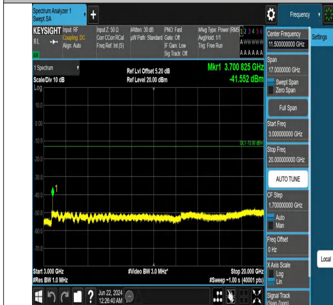
Band2_3MHz_QPSK_18615_1RB#0_3000~20000_3000~20000
