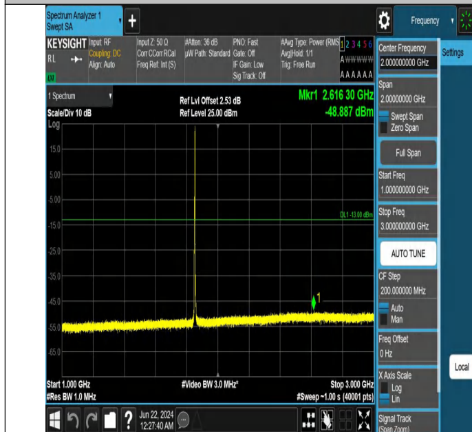
Band2_3MHz_QPSK_18615_1RB#14_1000~3000_1000~3000
