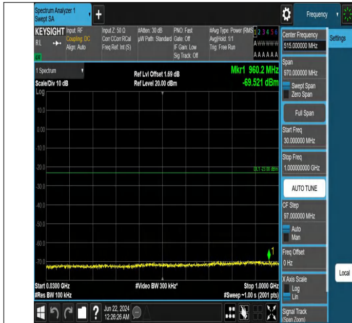
Band2_3MHz_QPSK_18615_1RB#0_30~1000_30~1000
