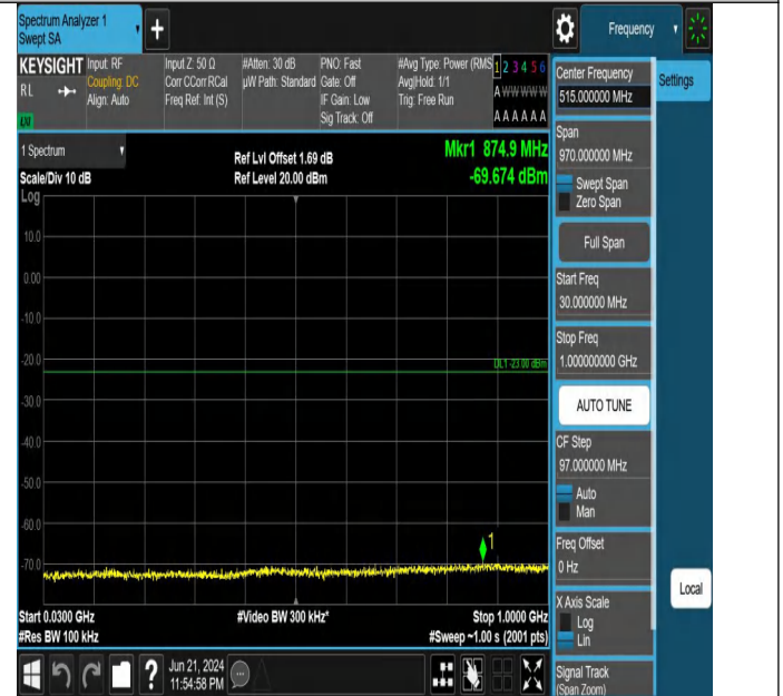
Band2_1.4MHz_QPSK_18607_1RB#5_30~1000_30~1000
