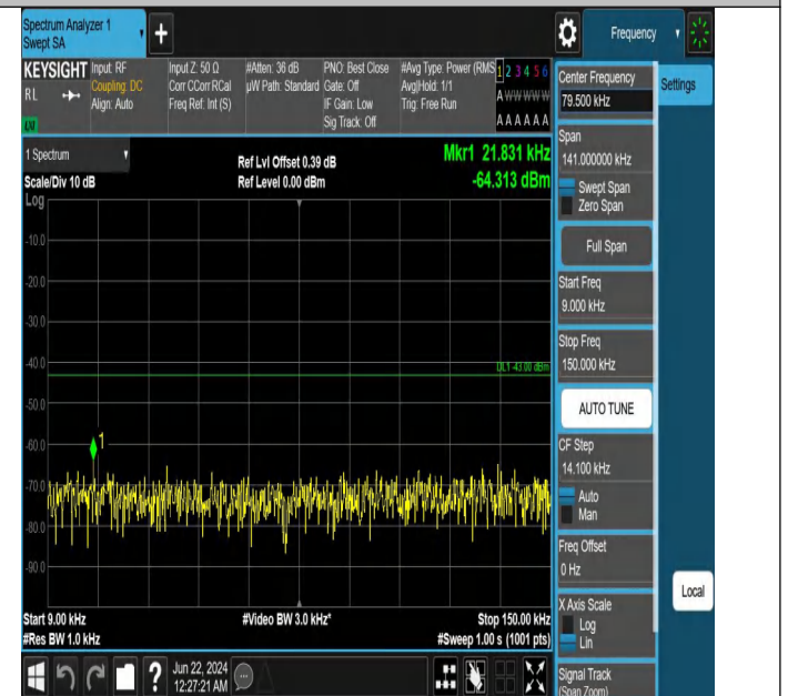
Band2_3MHz_QPSK_18615_1RB#14_0.009~0.15_0.009~0.15
