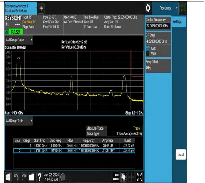
Band2_10MHz_QPSK_19150_1RB#0
