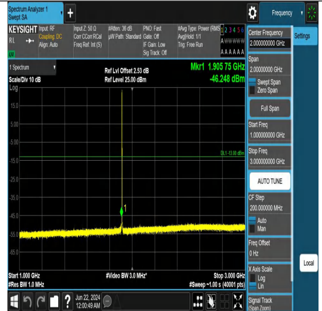
Band2_1.4MHz_QPSK_19193_1RB#0_1000~3000_1000~3000
