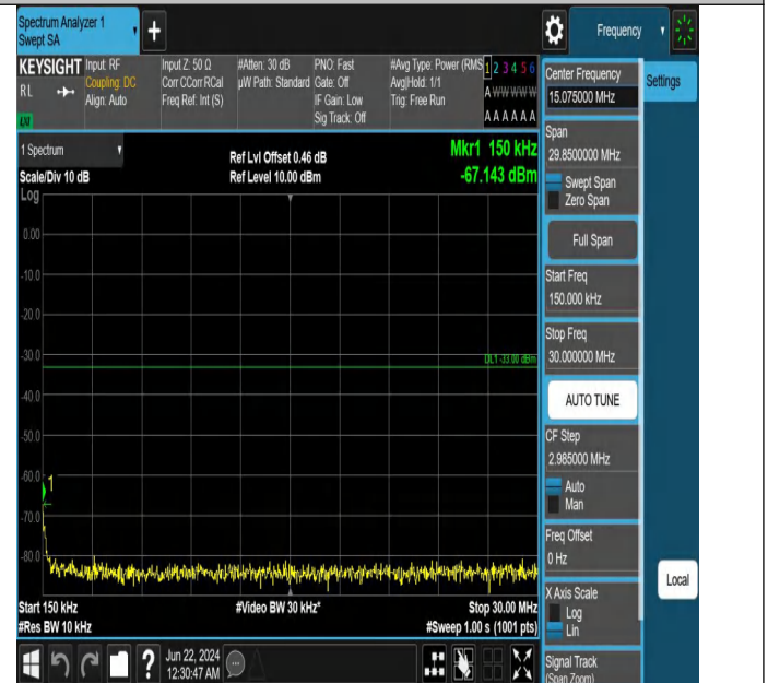
Band2_3MHz_QPSK_18900_1RB#14_0.15~30_0.15~30
