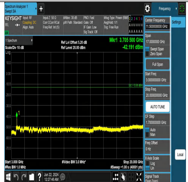
Band2_3MHz_QPSK_18615_1RB#14_3000~20000_3000~20000
