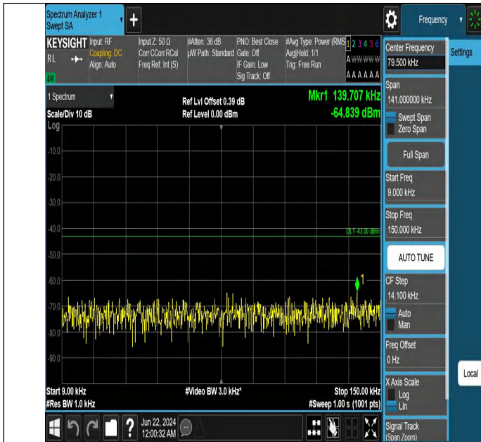
Band2_1.4MHz_QPSK_19193_1RB#0_0.009~0.15_0.009~0.15
