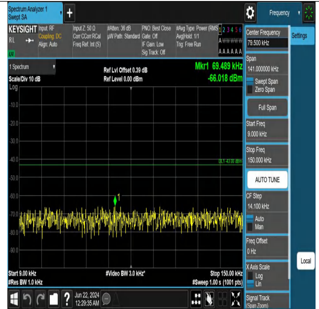
Band2_3MHz_QPSK_18900_1RB#0_0.009~0.15_0.009~0.15
