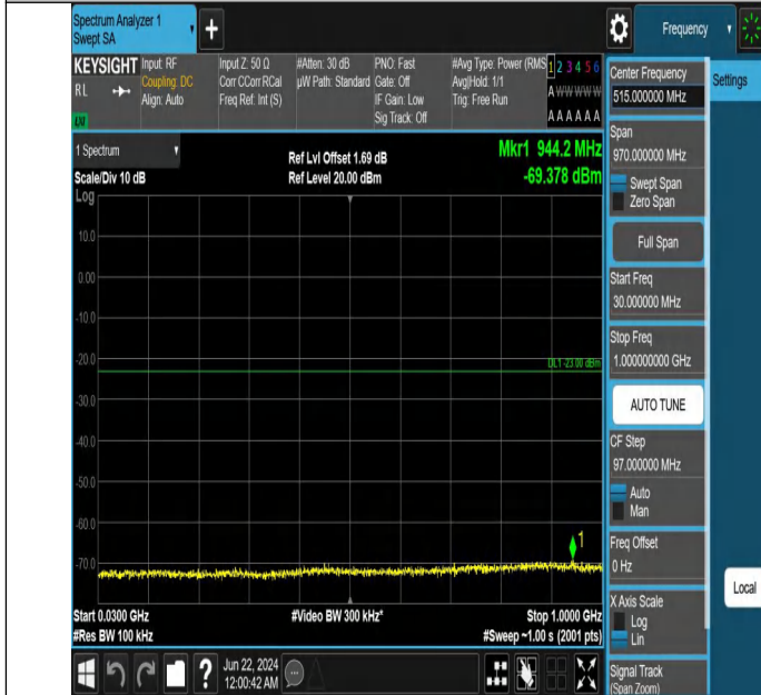
Band2_1.4MHz_QPSK_19193_1RB#0_30~1000_30~1000
