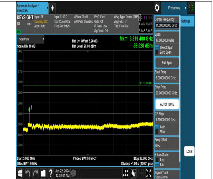
Band2_1.4MHz_QPSK_19193_1RB#5_3000~20000_3000~20000
