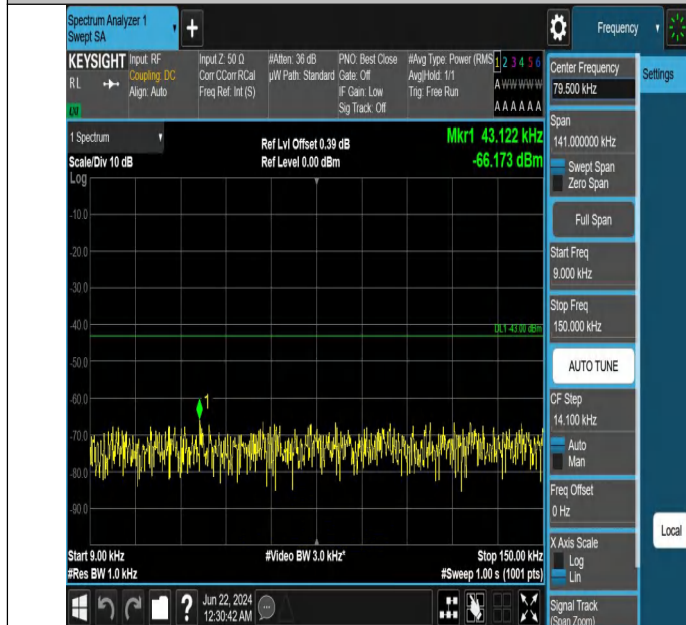
Band2_3MHz_QPSK_18900_1RB#14_0.009~0.15_0.009~0.15
