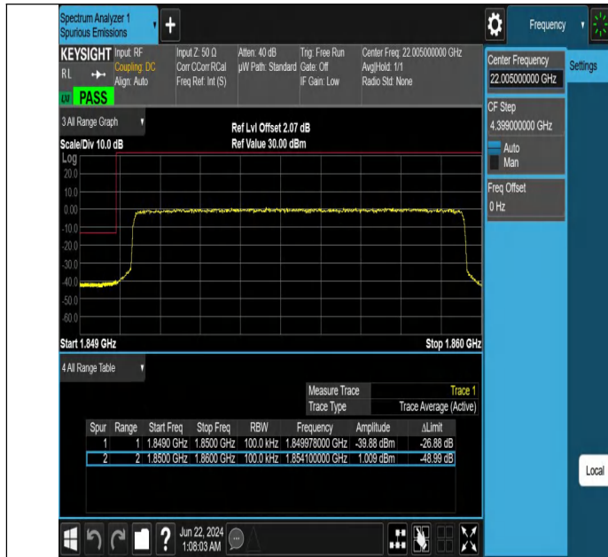
Band2_10MHz_QPSK_18650_50RB#0
