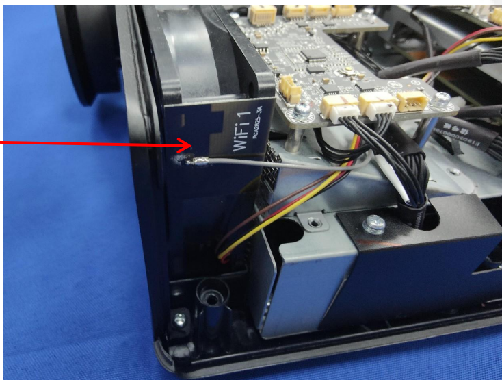
WIFI 1 Antenna
