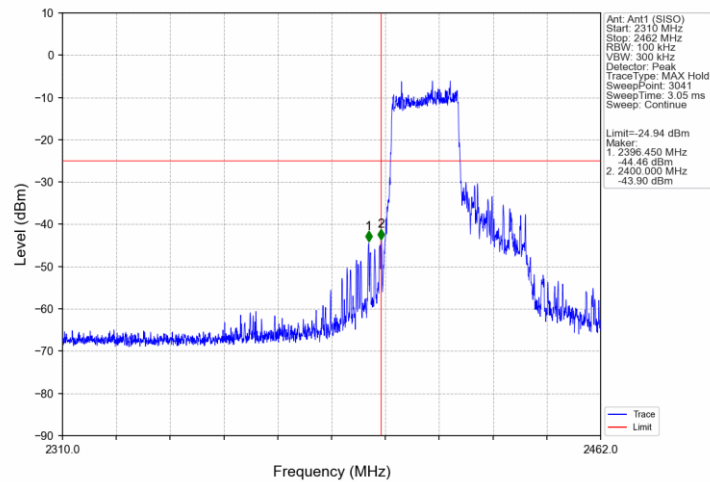
802.11ax(HEW40)_LCH_2422MHz_RU484_65_Ant1 (SISO)_NTNV
