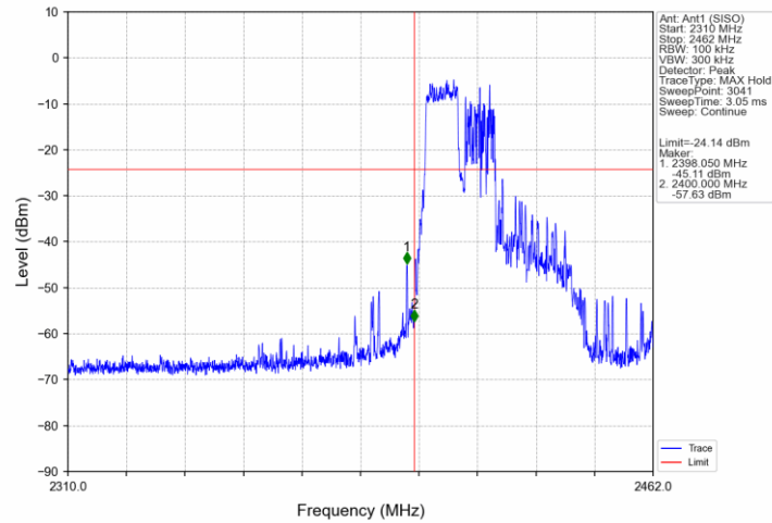
802.11ax(HEW40)_LCH_2422MHz_RU242_61_Ant1 (SISO)_NTNV
