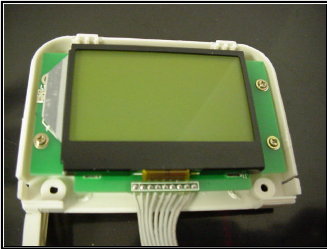
PHOTOGRAPH 16: LCD PCB TOP IN CHASSIS
