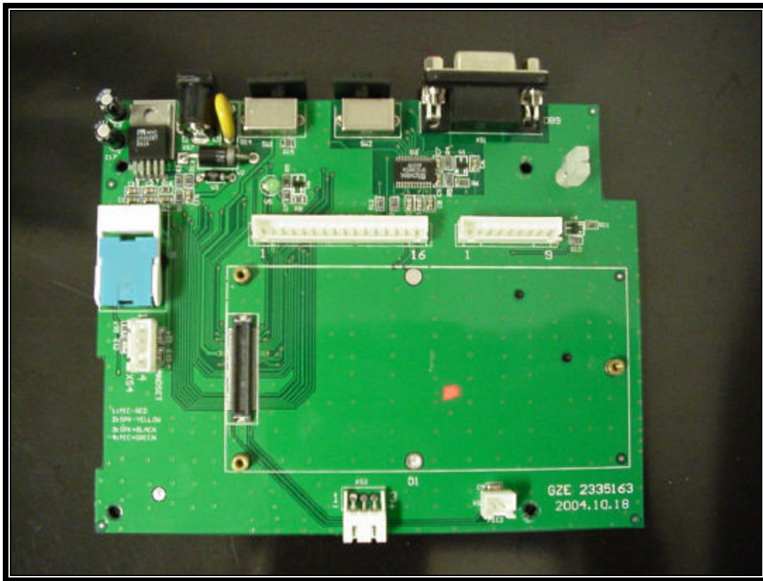
PHOTOGRAPH 21: MAIN PCB TOP
