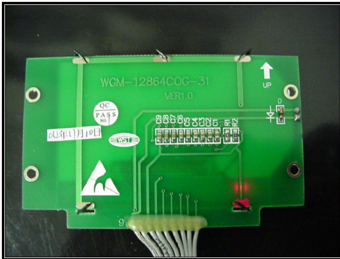
PHOTOGRAPH 18: LCD PCB BOTTOM
