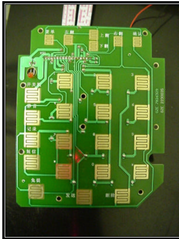
PHOTOGRAPH 15: KEYPAD PCB TOP
