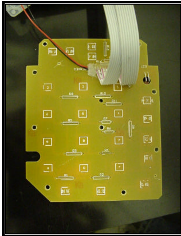
PHOTOGRAPH 14: KEYPAD PCB BOTTOM
