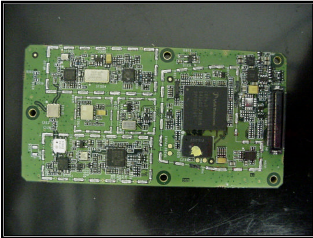
PHOTOGRAPH 13: RF PCB TOP SHIELDS REMOVED
