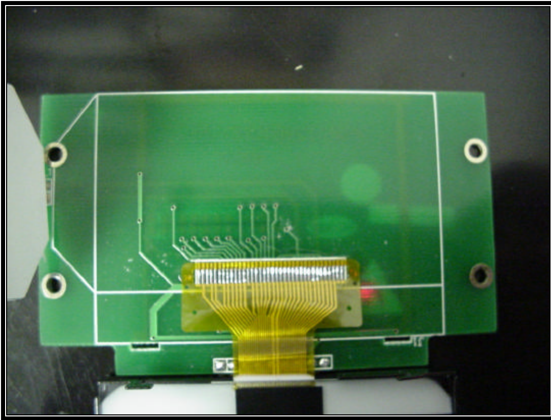
PHOTOGRAPH 19: LCD PCB LCD REMOVED
