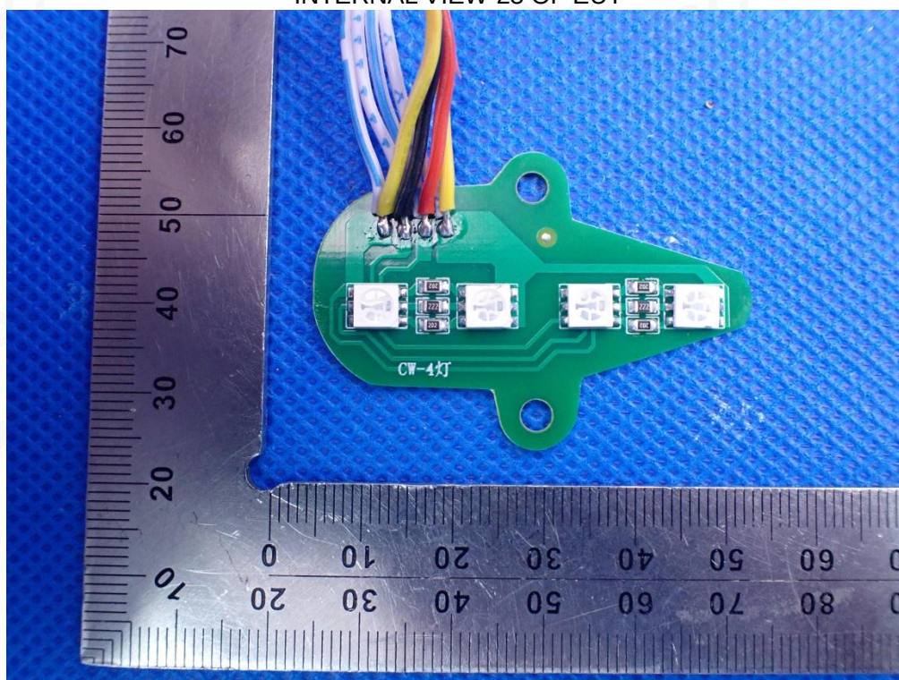
INTERNAL VIEW-25 OF EUT
