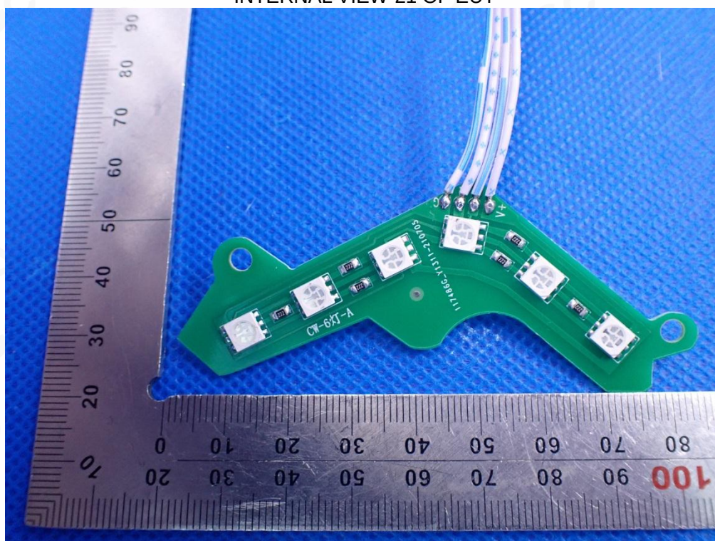
INTERNAL VIEW-21 OF EUT
