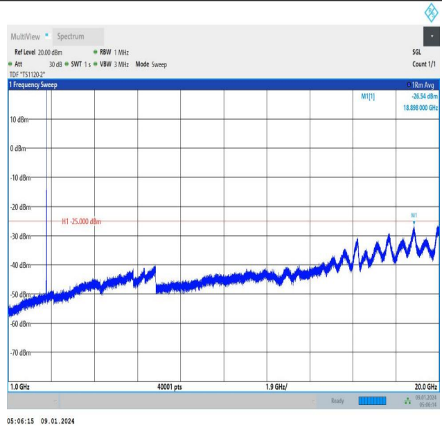
Band41_15MHz_16QAM_41515_1RB#74_1000~20000_1000~20000
