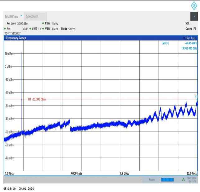
Band41_20MHz_QPSK_41490_100RB#0_1000~20000_1000~20000
