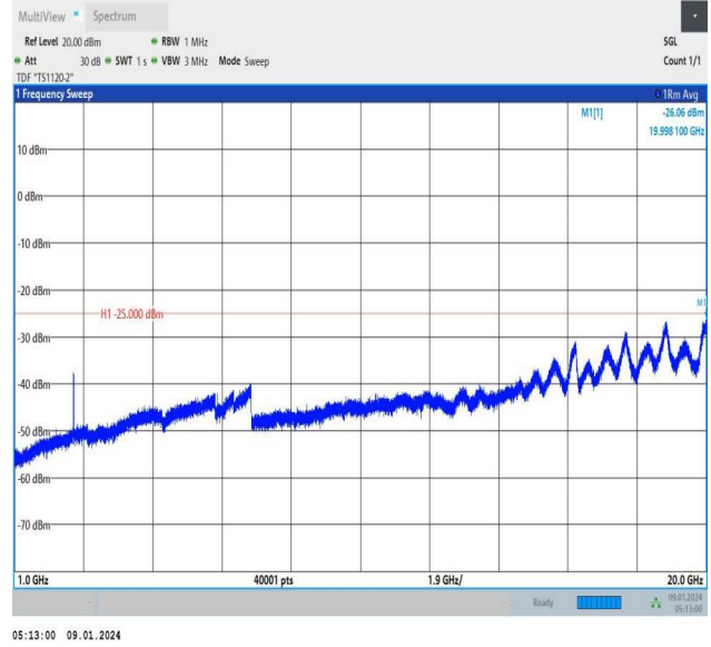
Band41_20MHz_QPSK_40620_1RB#99_1000~20000_1000~20000
