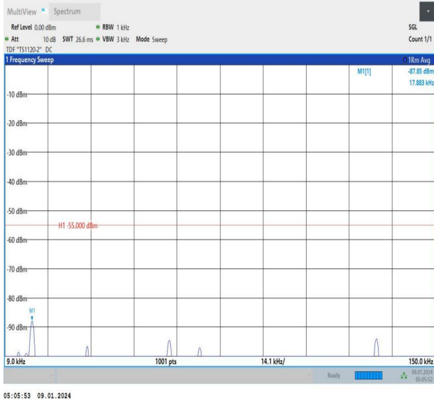
Band41_15MHz_16QAM_41515_1RB#74_0.009~0.15_0.009~0.15
