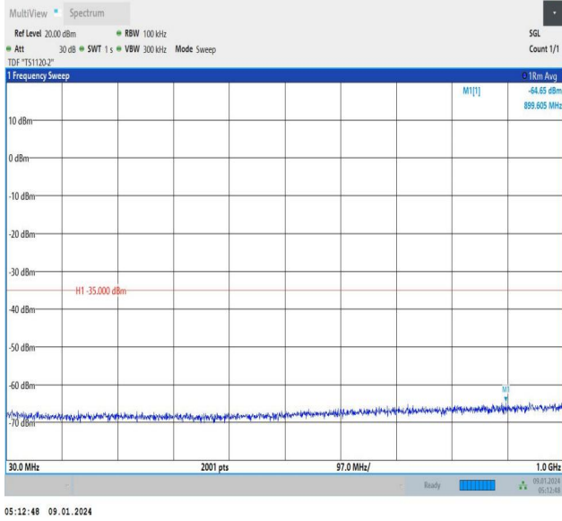
Band41_20MHz_QPSK_40620_1RB#99_30~1000_30~1000
