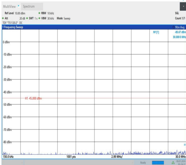
Band41_20MHz_16QAM_41490_1RB#0_0.15~30_0.15~30
