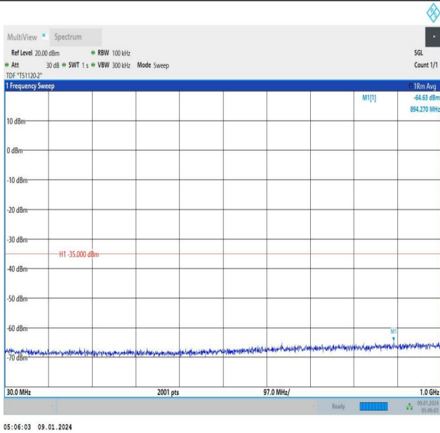
Band41_15MHz_16QAM_41515_1RB#74_30~1000_30~1000
