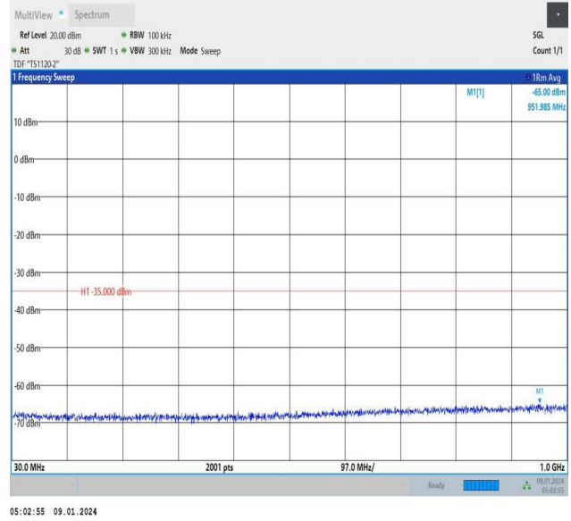
Band41_15MHz_QPSK_40620_1RB#74_30~1000_30~1000
