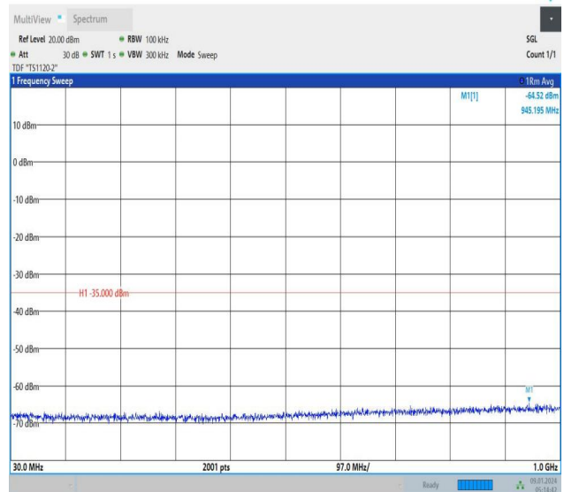
Band41_20MHz_16QAM_41490_1RB#0_30~1000_30~1000
