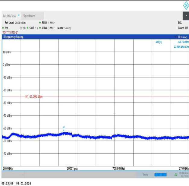
Band41_20MHz_QPSK_40620_1RB#99_20000~27000_20000~27000
