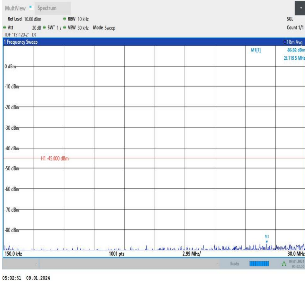
Band41_15MHz_QPSK_40620_1RB#74_0.15~30_0.15~30
