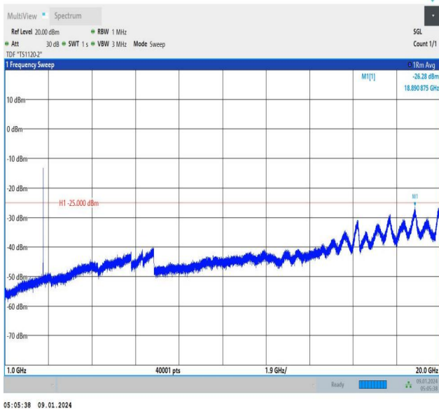
Band41_15MHz_QPSK_41515_1RB#74_1000~20000_1000~20000
