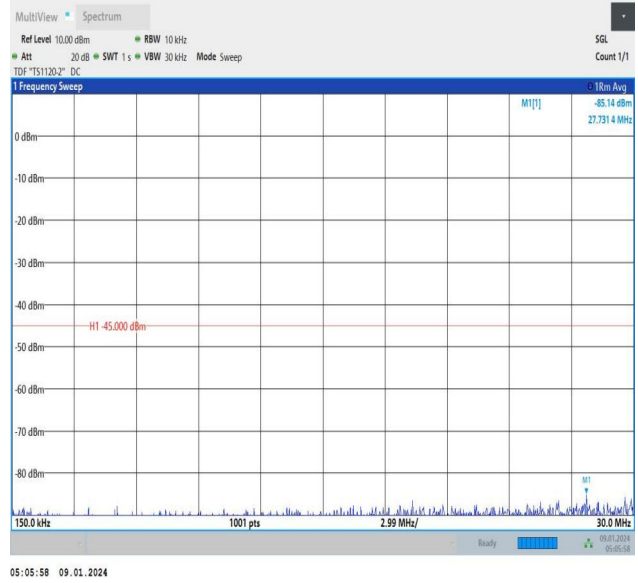
Band41_15MHz_16QAM_41515_1RB#74_0.15~30_0.15~30
