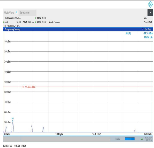
Band41_20MHz_16QAM_40620_1RB#99_0.009~0.15_0.009~0.15
