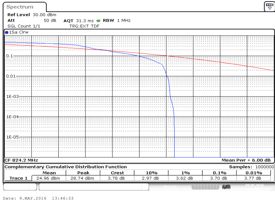
Plot 1: CCDF, channel 128
