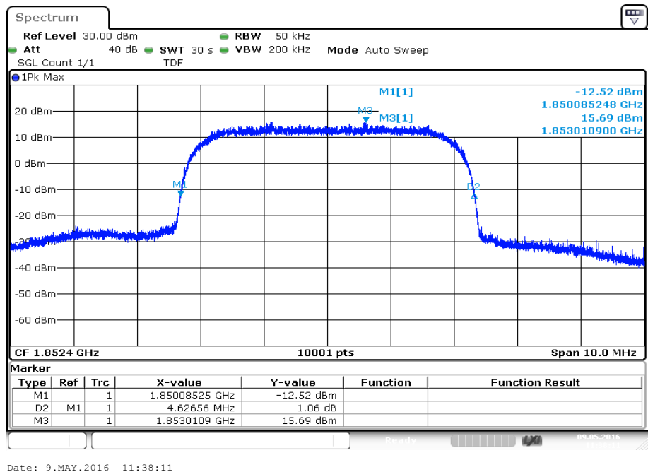
Plot 2: Channel 9262 (-26 dBc)
