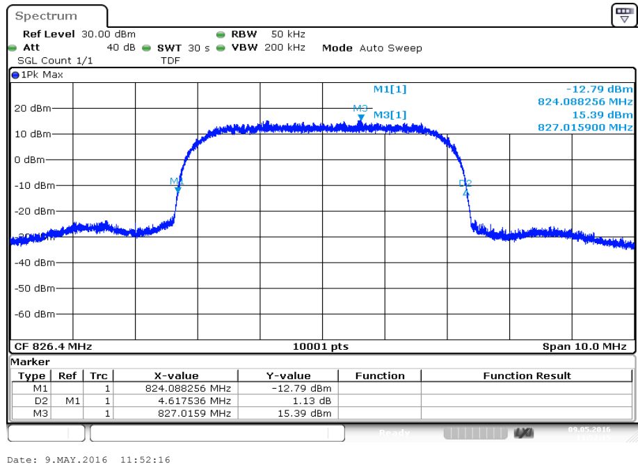
Plot 2: Channel 4132 (-26 dBc)
