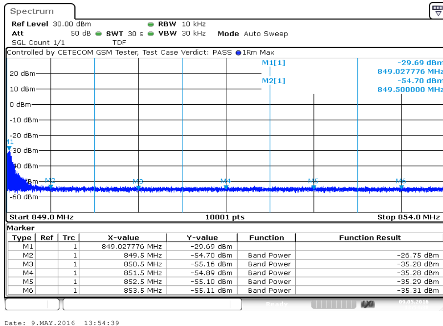
Plot 4: Channel 251 (EDGE)
