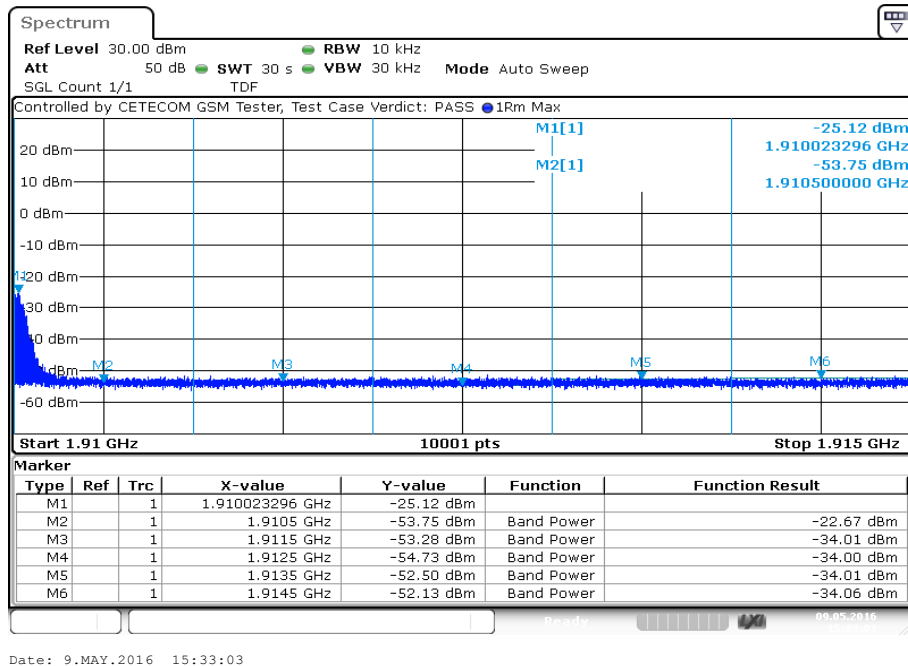
Plot 2: Channel 810 (GPRS)
