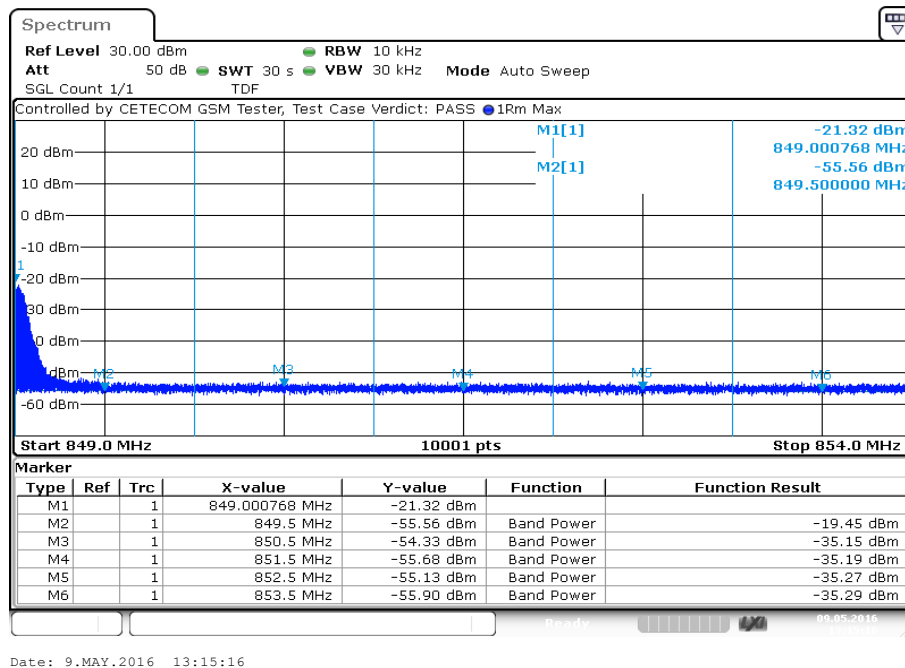
Plot 2: Channel 251 (GPRS)
