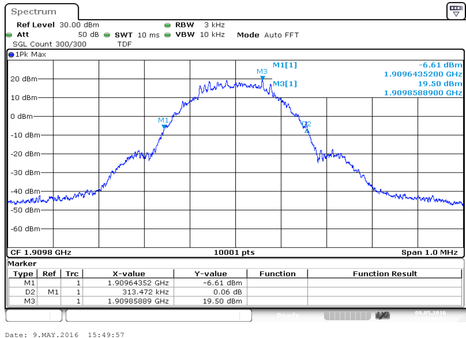
Plot 6: Channel 810 (-26 dBc)
