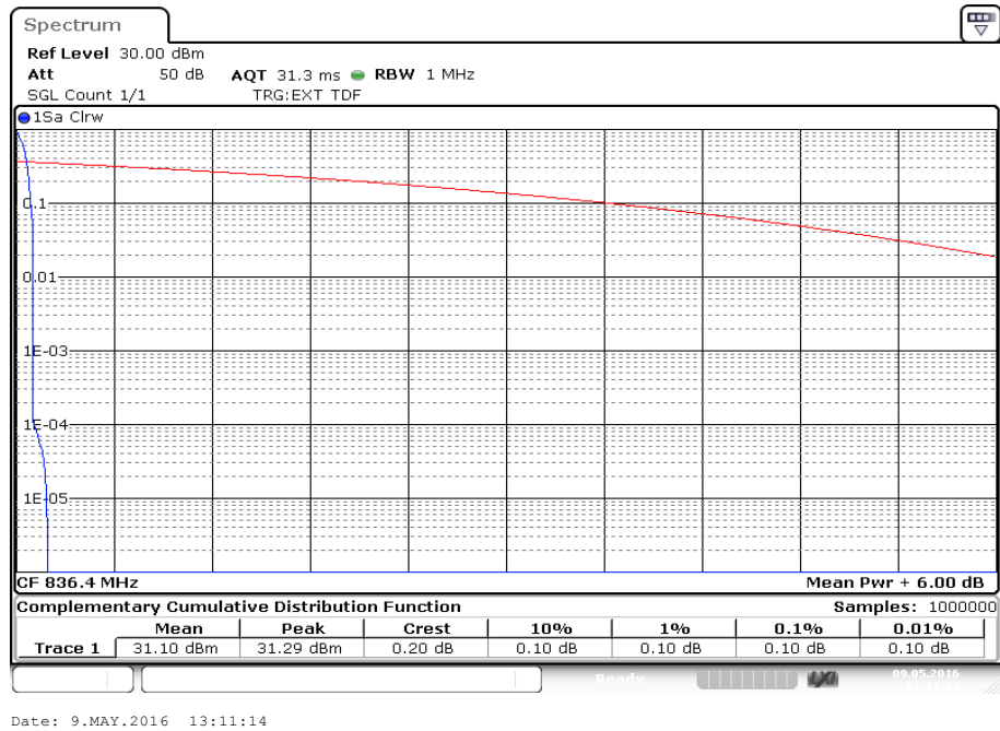
Plot 2: CCDF, channel 189
