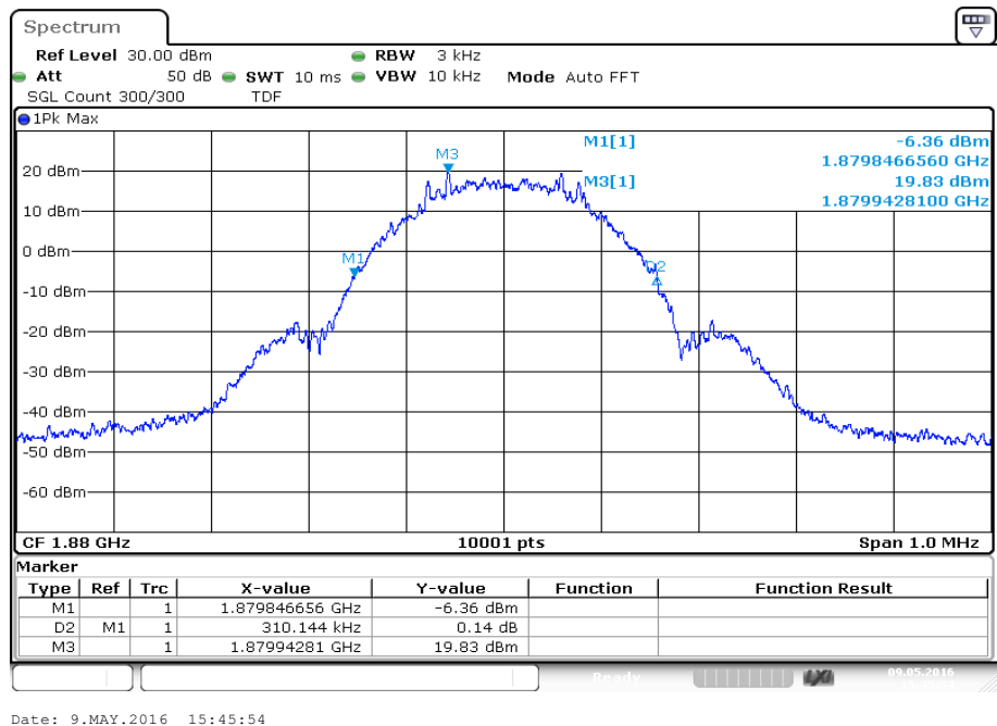
Plot 4: Channel 661 (-26 dBc)
