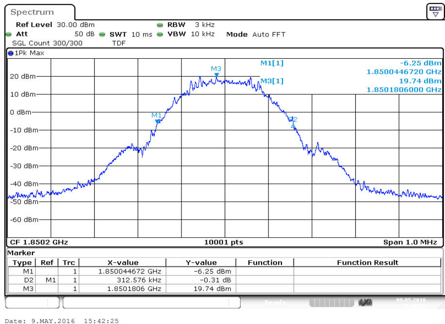
Plot 2: Channel 512 (-26 dBc)
