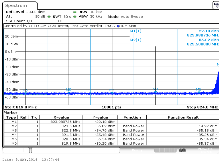
Plot 1: Channel 128 (GPRS)
