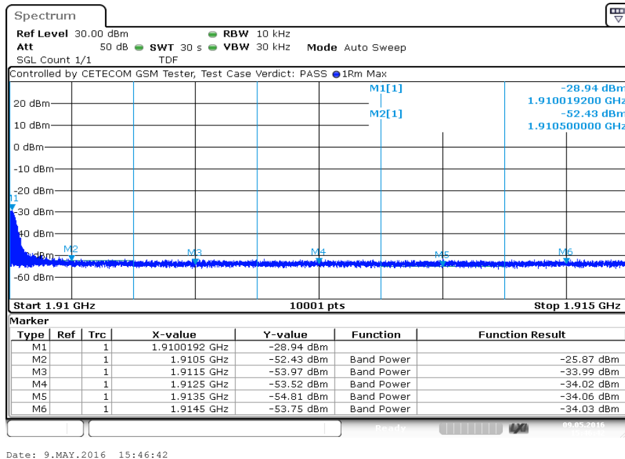
Plot 4: Channel 810 (EDGE)
