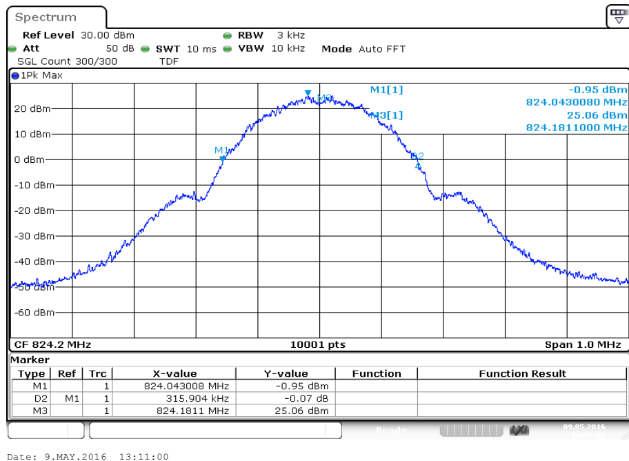
Plot 2: Channel 128 (-26 dBc)
