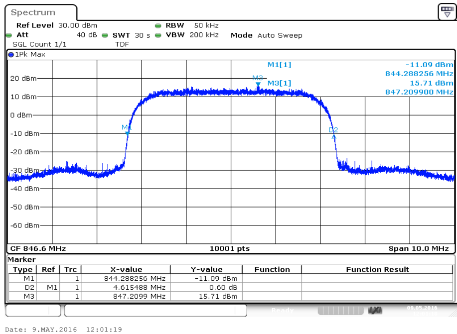
Plot 6: Channel 4233 (-26 dBc)
