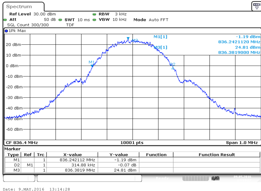
Plot 4: Channel 189 (-26 dBc)
