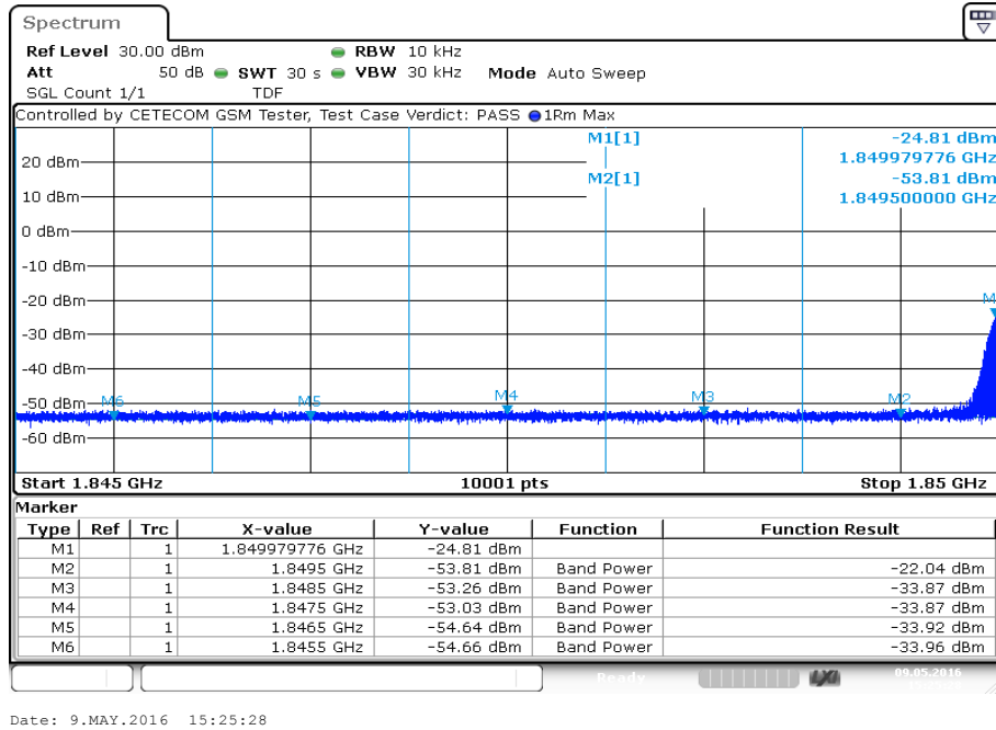
Plot 1: Channel 512 (GPRS)
