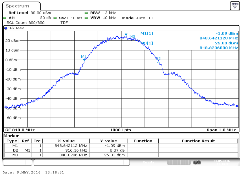
Plot 6: Channel 251 (-26 dBc)
