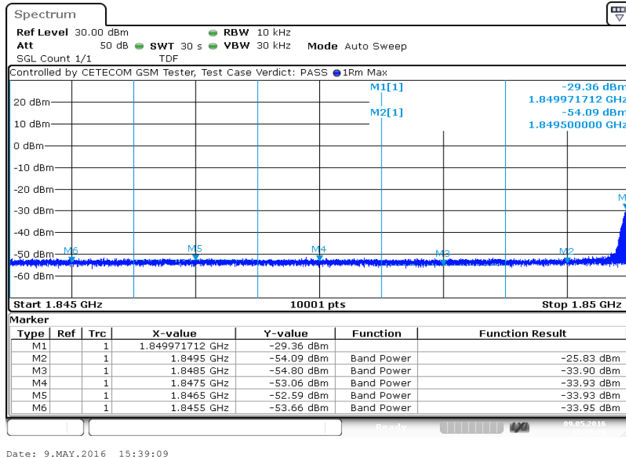
Plot 3: Channel 512 (EDGE)
