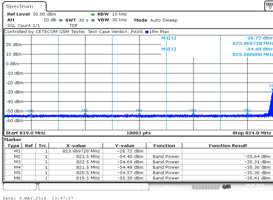
Plot 3: Channel 128 (EDGE)
