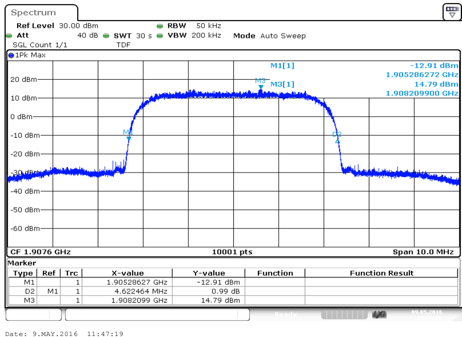
Plot 6: Channel 9538 (-26 dBc)
