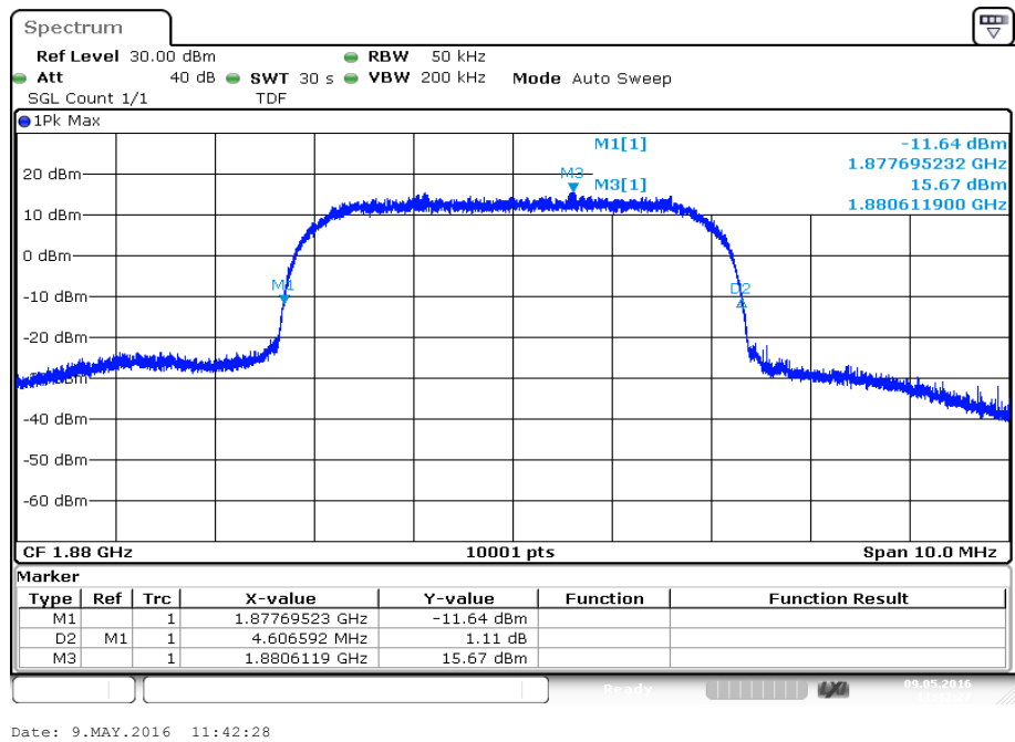
Plot 4: Channel 9400 (-26 dBc)
