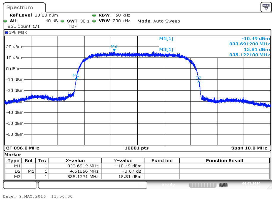
Plot 4: Channel 4180 (-26 dBc)
