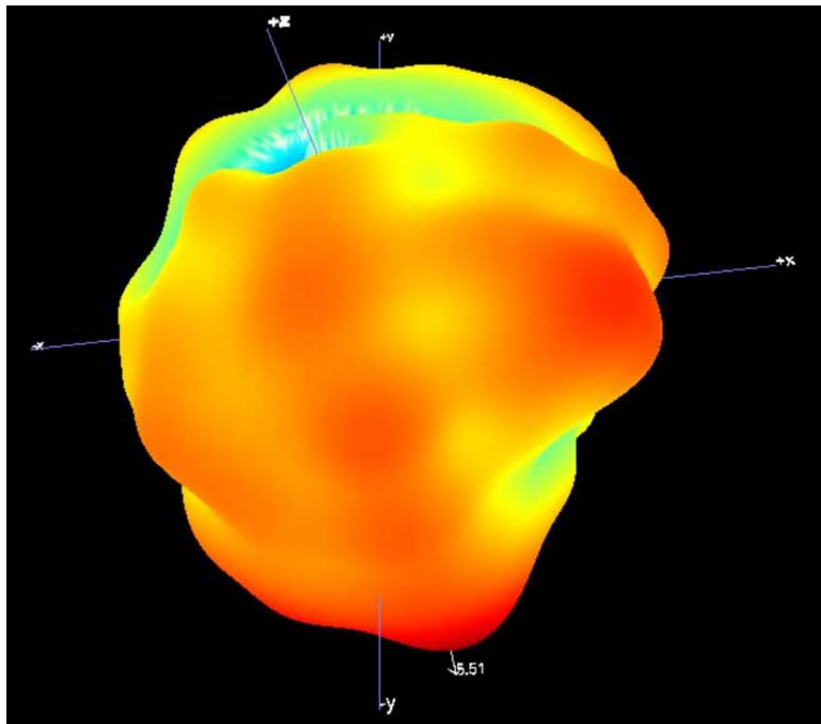
B1.3 3D Pattern for 2500MHz
