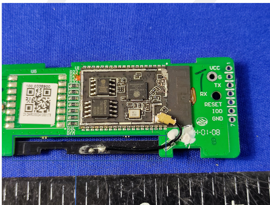
WIFI /BTANTENNA
