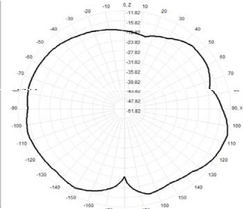
921.0MHz Total(E1-XZ), Max= -11.82dBi
