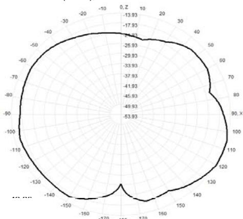
907.0MHz Total(E1-XZ), Max= -13.93dBi
