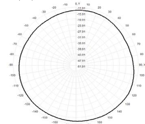
Total(H-XY), Max= -13.12dBi, CirD=3.66
