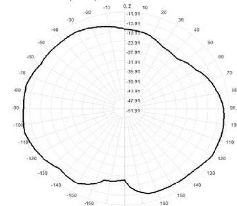
920.0MHz Total(E2-YZ), Max= -12.77dBi
