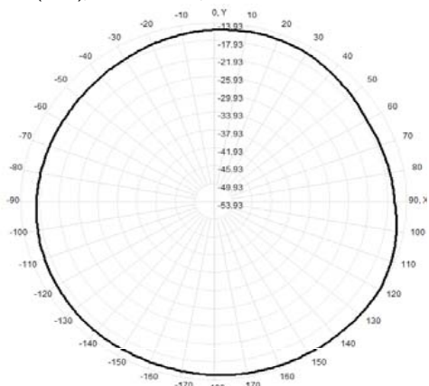
Total(H-XY), Max= -14.43dBi, CirD=3.49
