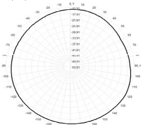
Total(H-XY), Max= -14.35dBi, CirD=3.60
