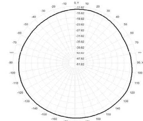
Total(H-XY), Max= -13.00dBi, CirD=3.67
