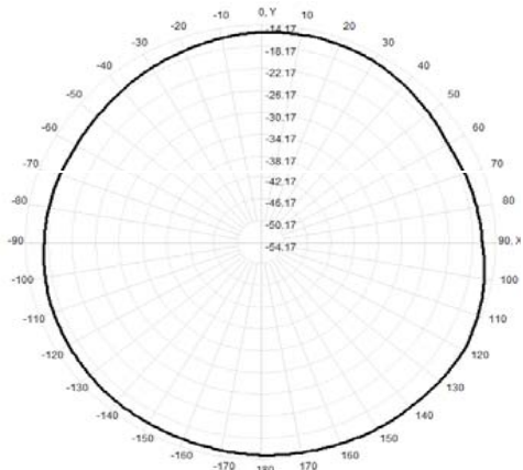
Total(H-XY), Max= -14.46dBi, CirD=3.61
