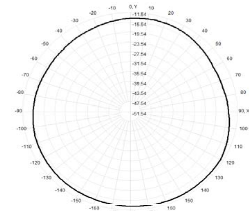
Total(H-XY), Max= -12.86dBi, CirD=3.61
