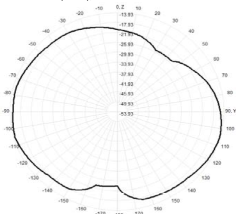
907.0MHz Total(E2-YZ), Max= -14.37dBi
