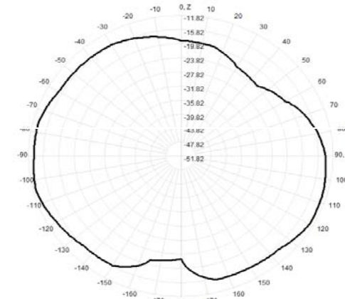
921.0MHz Total(E2-YZ), Max= -12.61dBi
