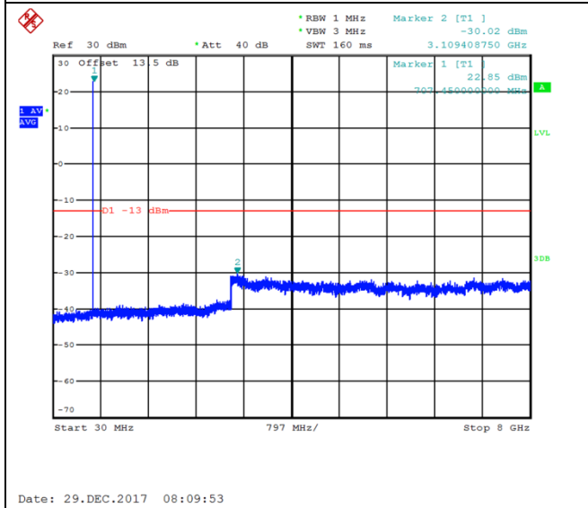
QPSK Middle channel-30MHz~8GHz
