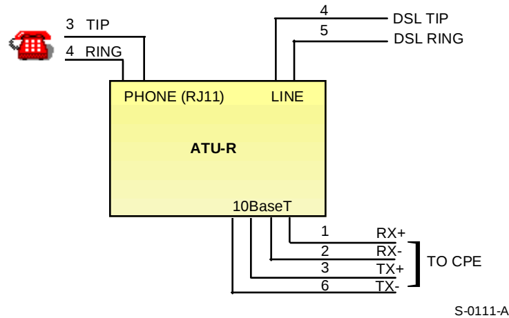
Figure 6. Installation Diagram with an Internal POTS Splitter
