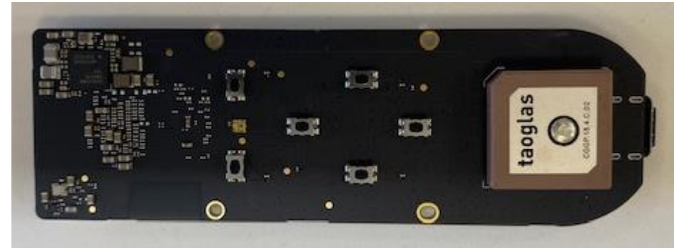
Beacon Main Logic Board Back Side
