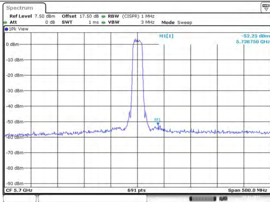
Plot on Configuration VHT20 / 5700 MHz / Peak / Port 3
