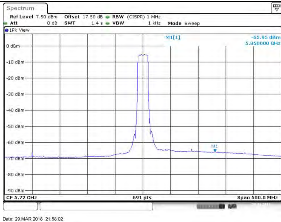
Plot on Configuration VHT20 / 5720 MHz / Average / Port 2
