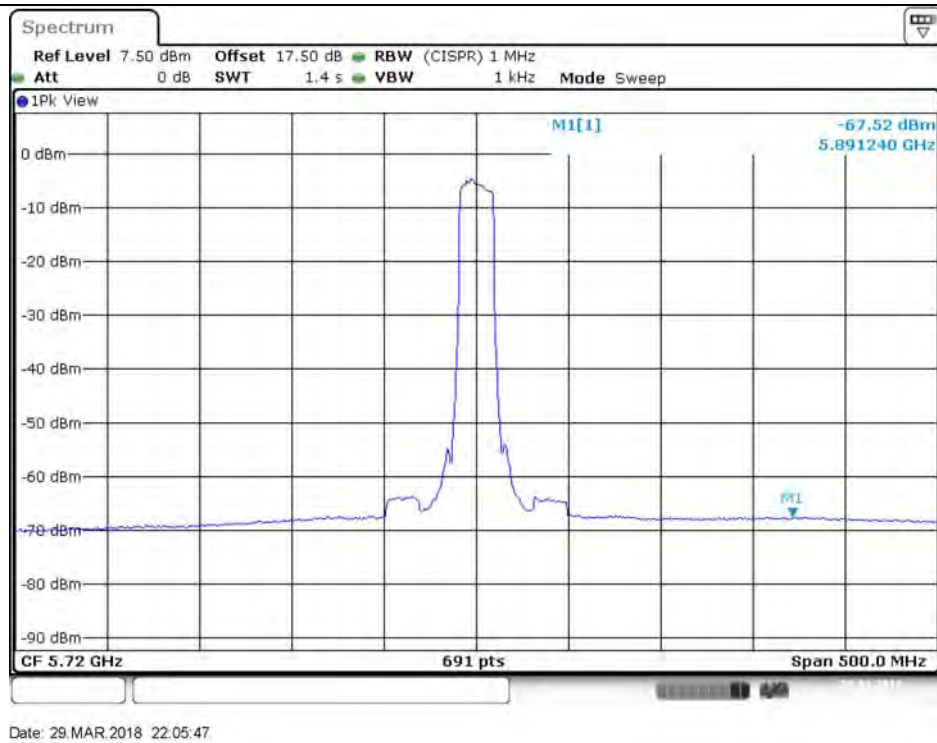
Plot on Configuration VHT20 / 5720 MHz / Average / Port 4
