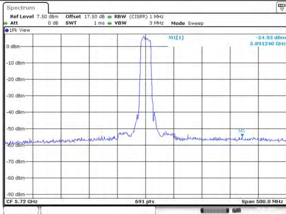
Plot on Configuration VHT20 / 5720 MHz / Peak / Port 3
