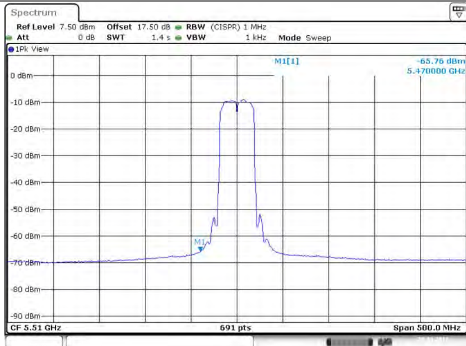
Plot on Configuration VHT40 / 5510 MHz / Average / Port 4
