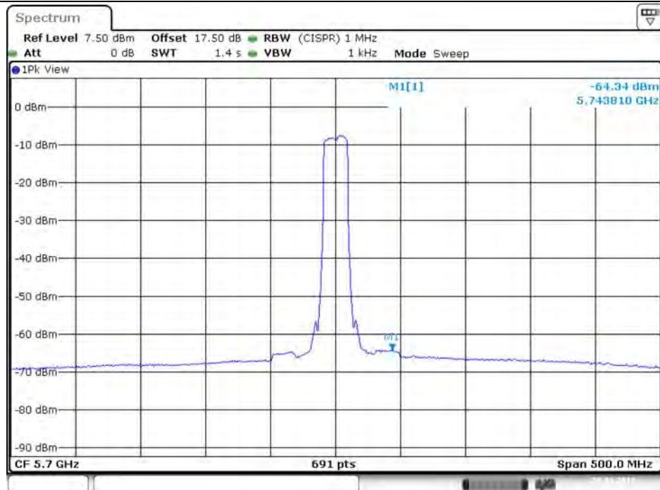
Plot on Configuration VHT20 / 5700 MHz / Average / Port 4
