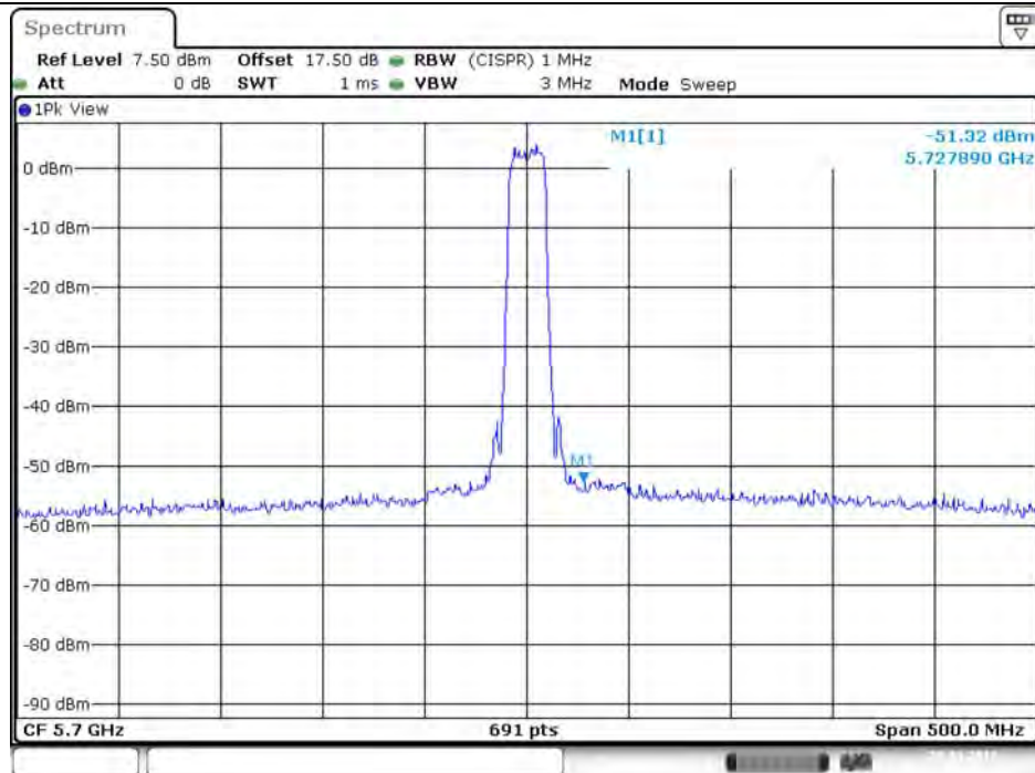
Plot on Configuration VHT20 / 5700 MHz / Peak / Port 4
