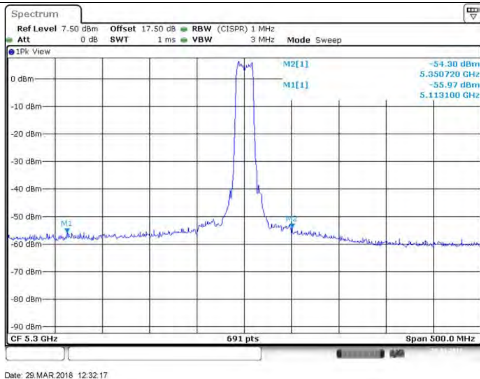
Plot on Configuration VHT20 / 5300 MHz / Peak / Port 4
