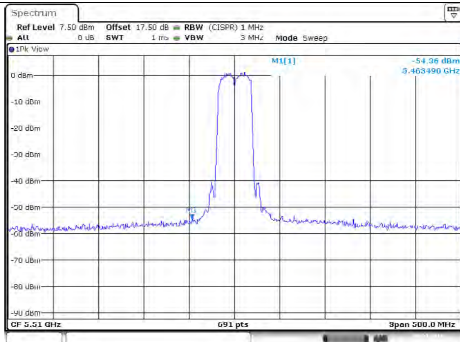
Plot on Configuration VHT40 / 5510 MHz / Peak / Port 2
