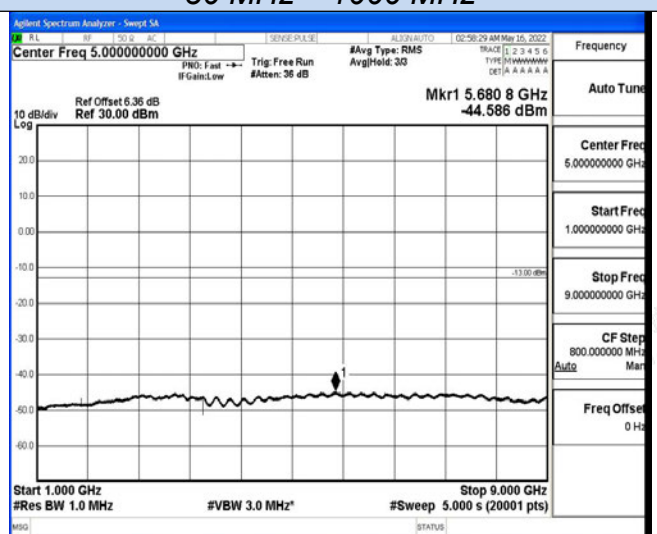
1 GHz – 9 GHz
