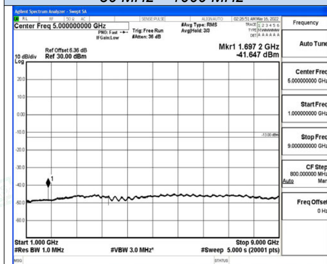
1 GHz – 9 GHz
