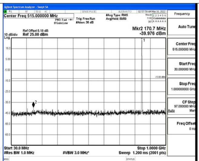
30 MHz – 1000 MHz
