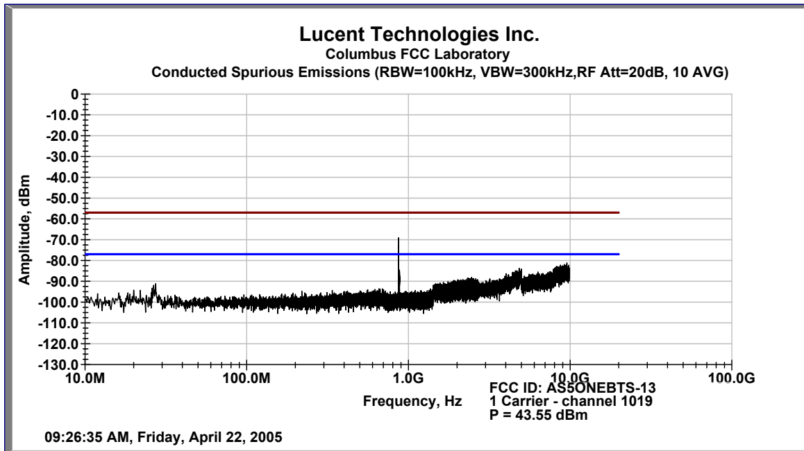
FIGURE 13.5.2 OUT-OF-BLOCK SPURIOUS CONDUCTED EMISSIONS PLOTS
