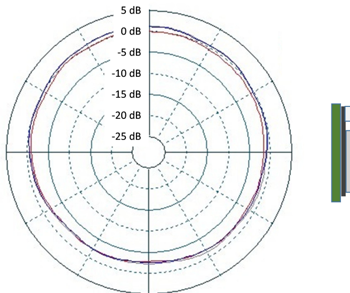
Figure 9.2. Typical 2D Radiation Pattern – Side View
