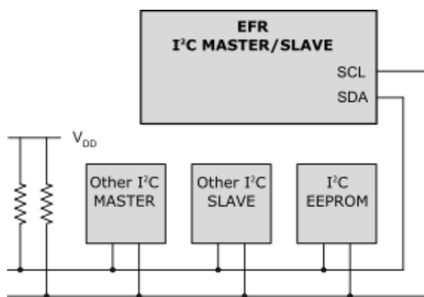
Figure 3.2. I2C
