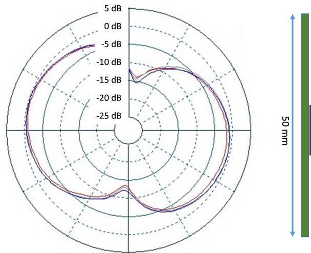
Figure 9.1. Typical 2D Radiation Pattern – Front View
