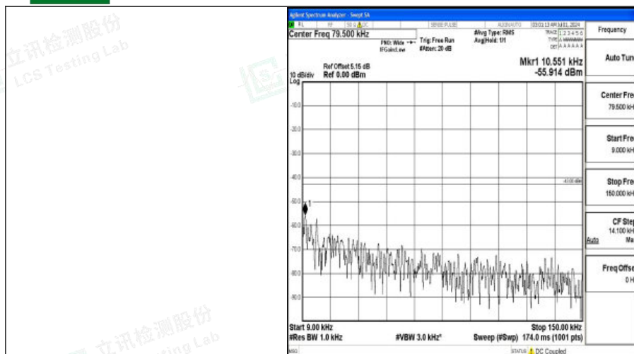
Band66_20MHz_16QAM_132572_1RB#0_0.009~0.15_0.009~0.15
