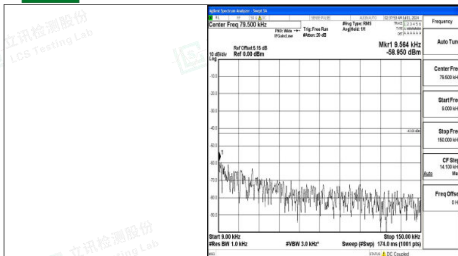
Band66_15MHz_16QAM_132597_1RB#0_0.009~0.15_0.009~0.15
