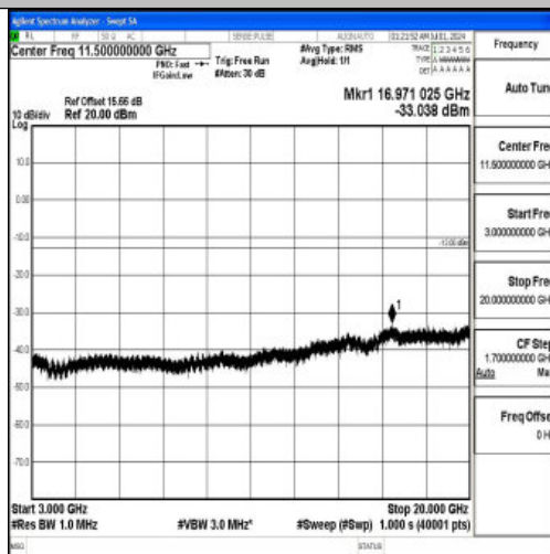
Band66_3MHz_QPSK_132657_1RB#0_3000~20000_3000~20000
