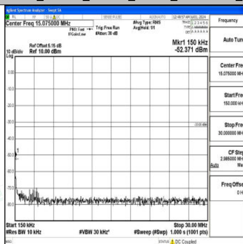
Band66_1.4MHz_16QAM_132665_1RB#0_0.15~30_0.15~30
