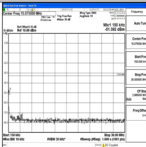
Band66_3MHz_QPSK_132657_1RB#0_0.15~30_0.15~30
