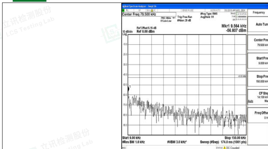
Band66_3MHz_16QAM_132657_1RB#0_0.009~0.15_0.009~0.15
