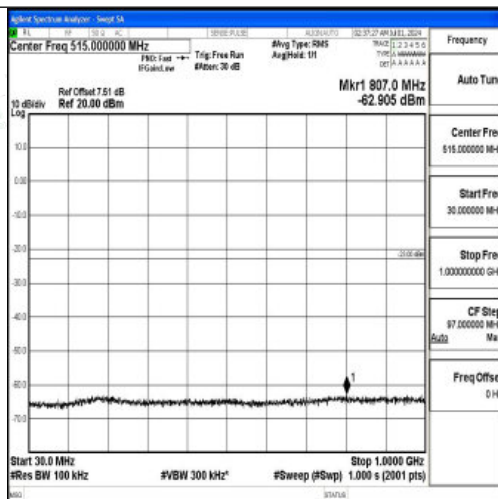
Band66_15MHz_QPSK_132597_1RB#0_30~1000_30~1000
