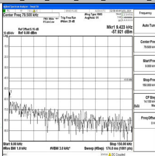
Band66_20MHz_16QAM_132072_1RB#0_0.009~0.15_0.009~0.15
