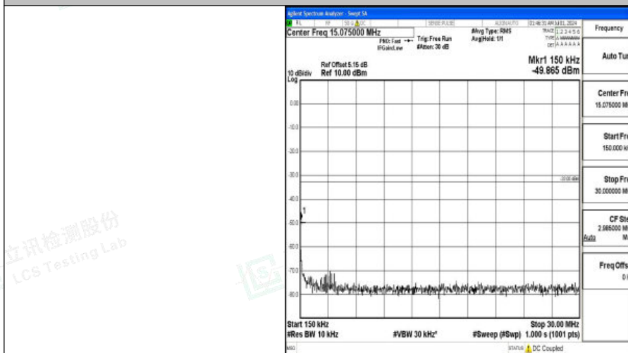
Band66_5MHz_QPSK_132322_1RB#0_0.15~30_0.15~30
