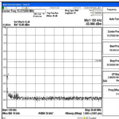
Band66_15MHz_16QAM_132322_1RB#0_0.15~30_0.15~30
