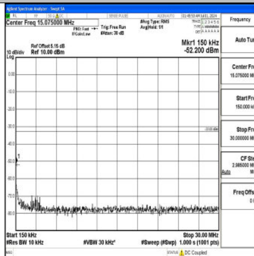
Band66_5MHz_16QAM_131997_1RB#0_0.15~30_0.15~30
