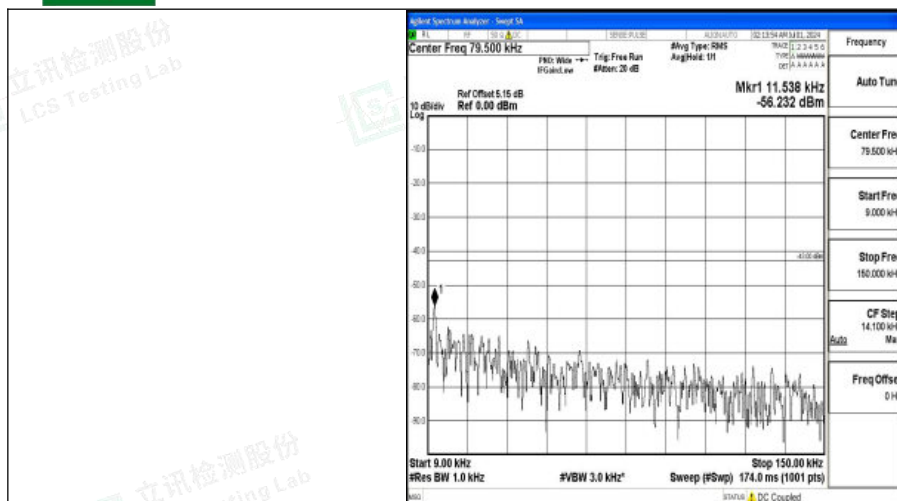
Band66_10MHz_16QAM_132622_1RB#0_0.009~0.15_0.009~0.15
