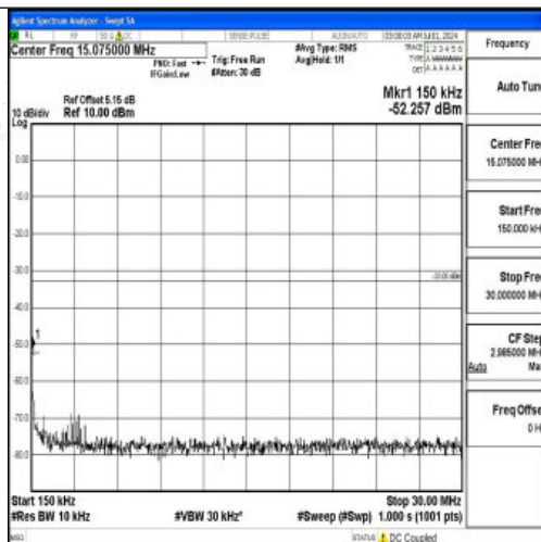
Band66_20MHz_16QAM_132322_1RB#0_0.15~30_0.15~30
