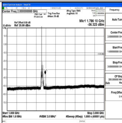
Band66_20MHz_QPSK_132072_1RB#0_1000~3000_1000~3000
