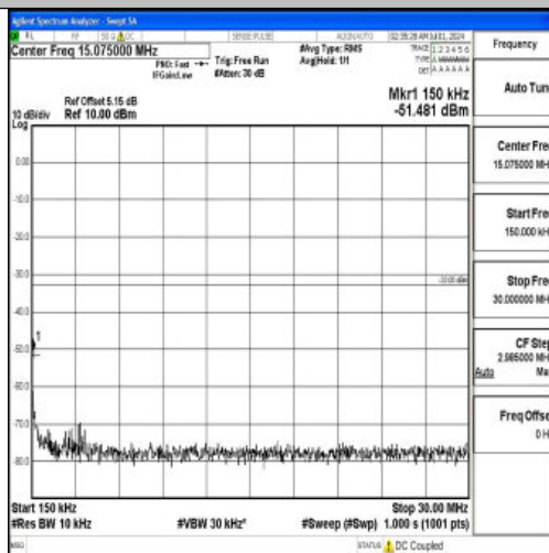
Band66_15MHz_16QAM_132047_1RB#0_0.15~30_0.15~30
