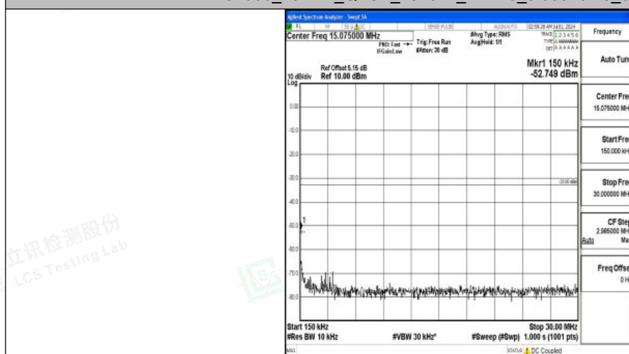
Band66_20MHz_QPSK_132322_1RB#0_0.15~30_0.15~30
