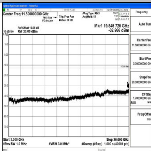
Band66_15MHz_16QAM_132047_1RB#0_3000~20000_3000~20000
