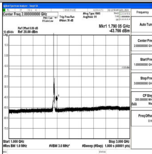
Band66_10MHz_16QAM_132322_1RB#0_1000~3000_1000~3000
