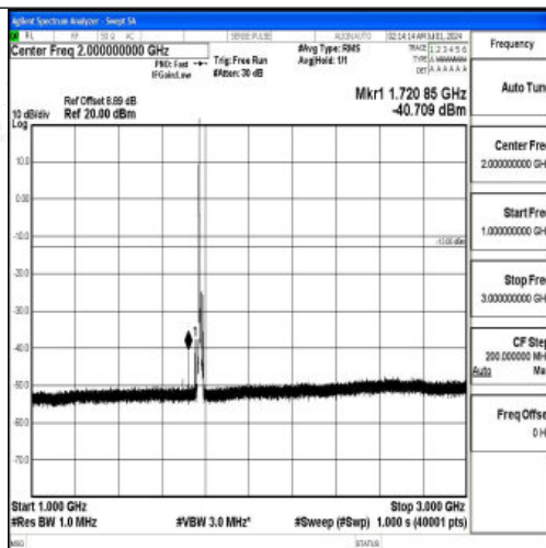
Band66_10MHz_16QAM_132622_1RB#0_1000~3000_1000~3000
