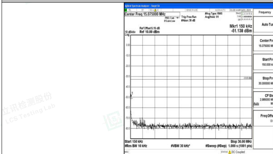
Band66_3MHz_QPSK_132322_1RB#0_0.15~30_0.15~30
