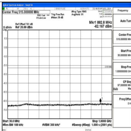
Band66_5MHz_16QAM_131997_1RB#0_30~1000_30~1000
