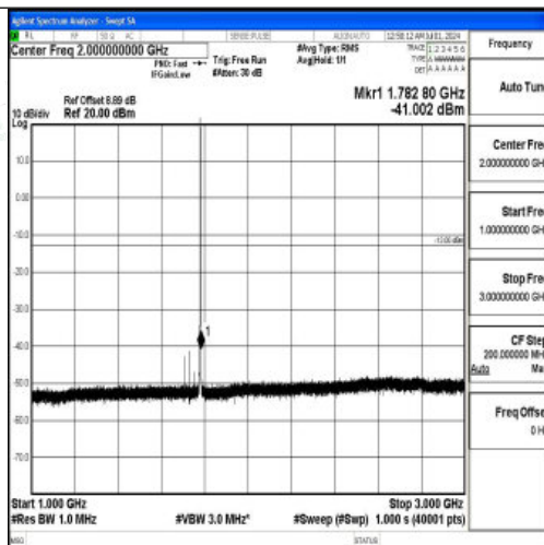
Band66_1.4MHz_16QAM_132665_1RB#0_1000~3000_1000~3000
