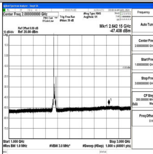
Band66_20MHz_16QAM_132322_1RB#0_1000~3000_1000~3000
