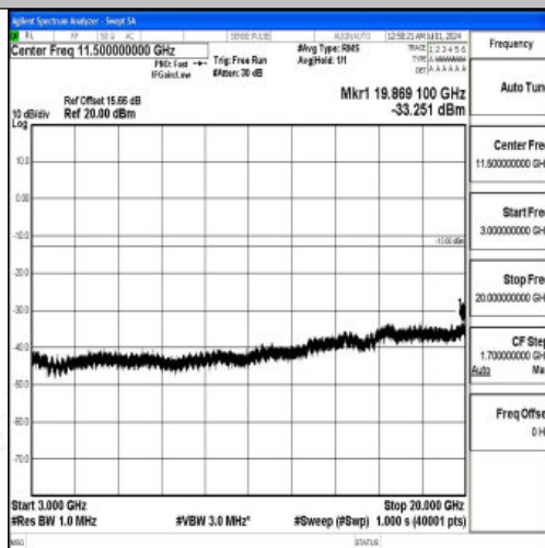
Band66_1.4MHz_16QAM_132665_1RB#0_3000~20000_3000~20000
