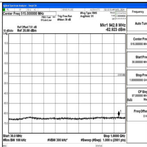
Band66_10MHz_QPSK_132622_1RB#0_30~1000_30~1000
