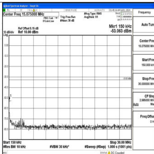
Band66_5MHz_QPSK_131997_1RB#0_0.15~30_0.15~30
