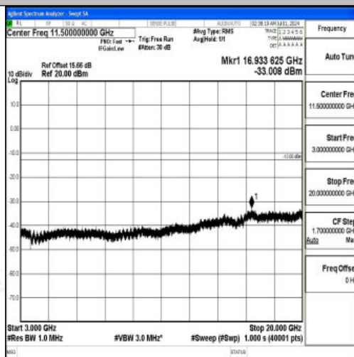
Band66_15MHz_16QAM_132597_1RB#0_3000~20000_3000~20000
