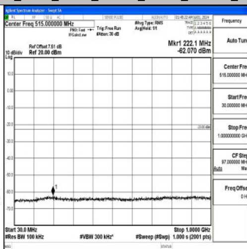
Band66_5MHz_QPSK_131997_1RB#0_30~1000_30~1000
