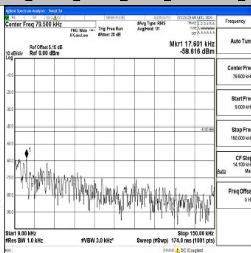
Band66_3MHz_QPSK_132657_1RB#0_0.009~0.15_0.009~0.15
