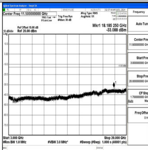
Band66_15MHz_QPSK_132597_1RB#0_3000~20000_3000~20000
