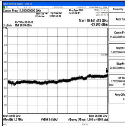
Band66_5MHz_QPSK_131997_1RB#0_3000~20000_3000~20000
