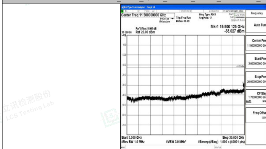
Band66_5MHz_QPSK_132322_1RB#0_3000~20000_3000~20000
