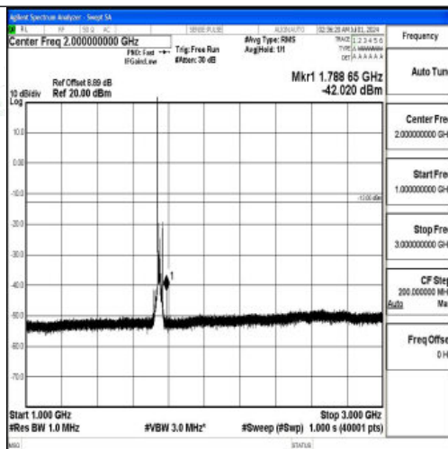
Band66_15MHz_QPSK_132322_1RB#0_1000~3000_1000~3000
