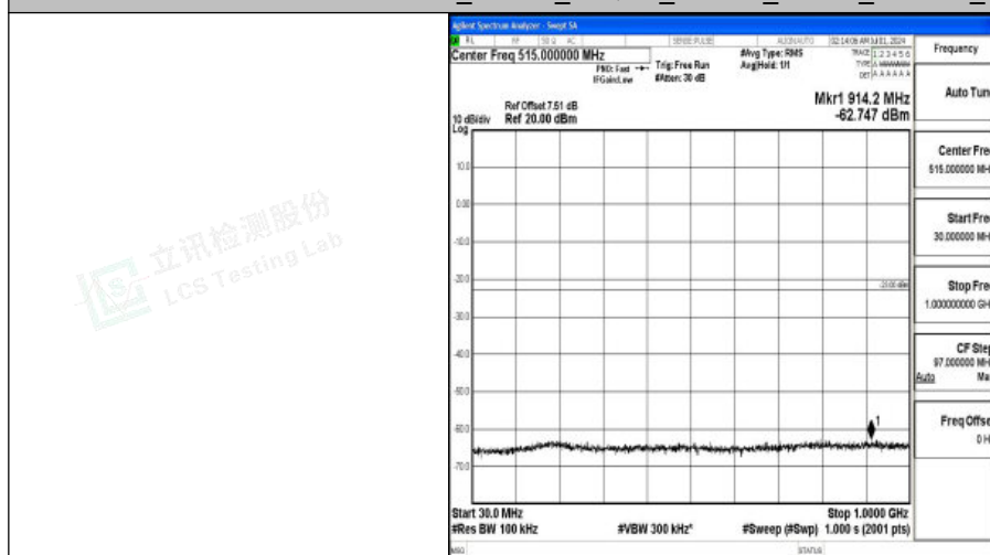
Band66_10MHz_16QAM_132622_1RB#0_30~1000_30~1000
