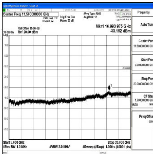
Band66_15MHz_16QAM_132322_1RB#0_3000~20000_3000~20000
