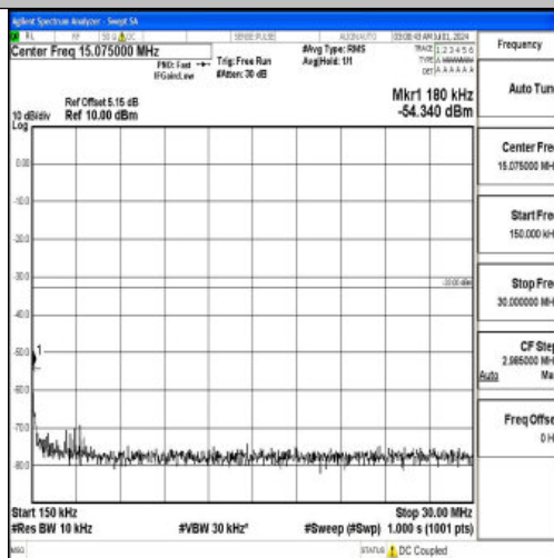
Band66_20MHz_QPSK_132572_1RB#0_0.15~30_0.15~30
