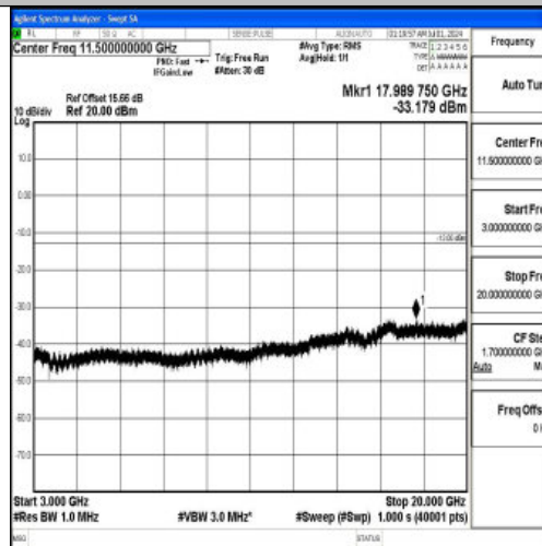
Band66_3MHz_16QAM_131987_1RB#0_3000~20000_3000~20000
