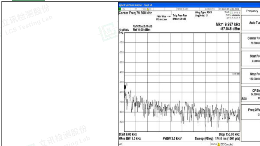
Band66_5MHz_QPSK_132322_1RB#0_0.009~0.15_0.009~0.15
