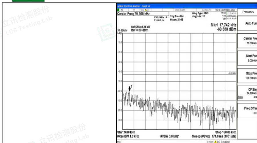
Band66_5MHz_16QAM_132647_1RB#0_0.009~0.15_0.009~0.15
