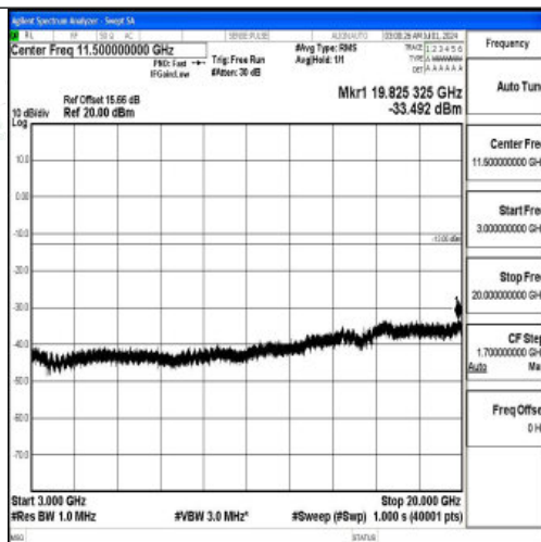
Band66_20MHz_16QAM_132322_1RB#0_3000~20000_3000~20000
