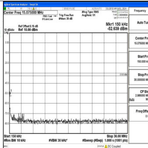
Band66_3MHz_16QAM_132322_1RB#0_0.15~30_0.15~30
