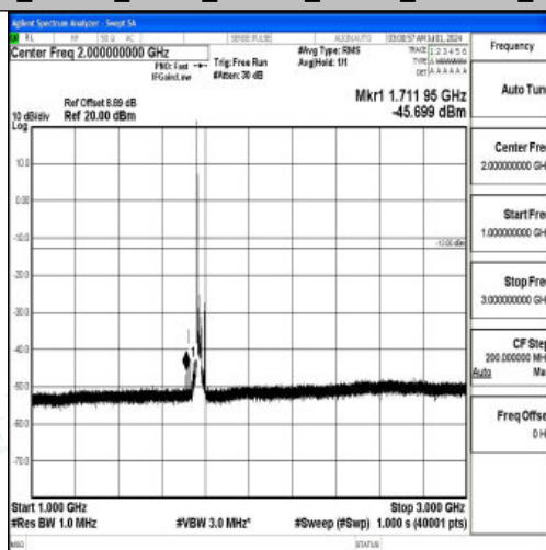
Band66_20MHz_QPSK_132572_1RB#0_1000~3000_1000~3000
