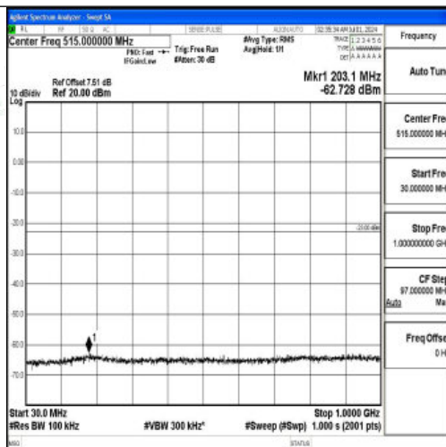
Band66_15MHz_16QAM_132047_1RB#0_30~1000_30~1000
