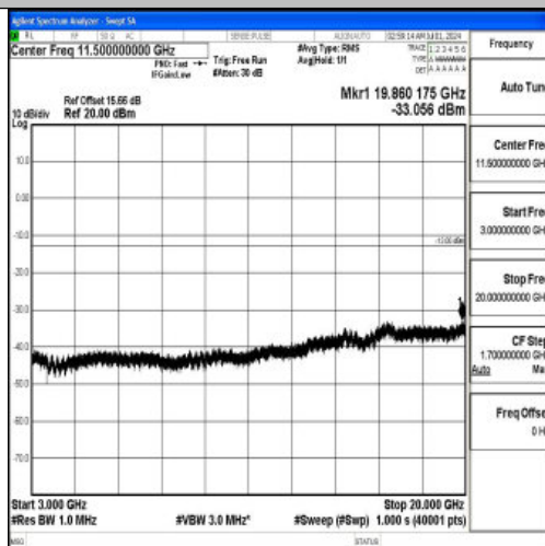
Band66_20MHz_16QAM_132072_1RB#0_3000~20000_3000~20000
