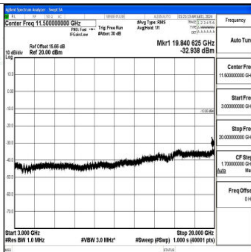
Band66_3MHz_16QAM_132322_1RB#0_3000~20000_3000~20000
