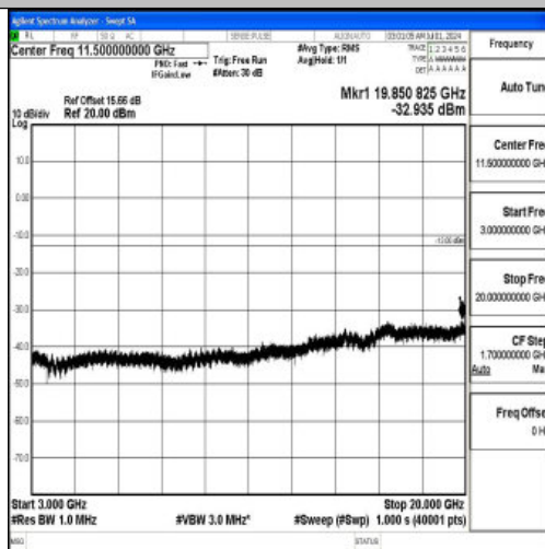
Band66_20MHz_QPSK_132572_1RB#0_3000~20000_3000~20000
