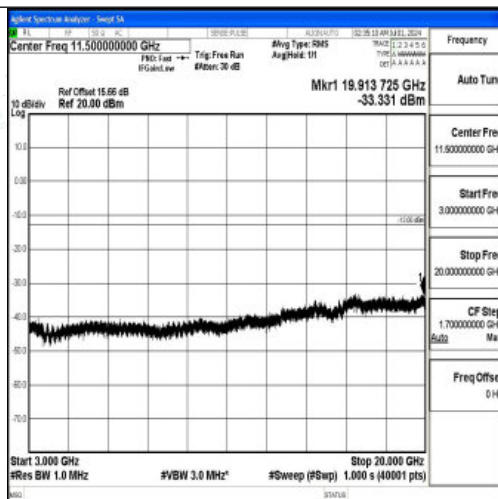
Band66_15MHz_QPSK_132047_1RB#0_3000~20000_3000~20000
