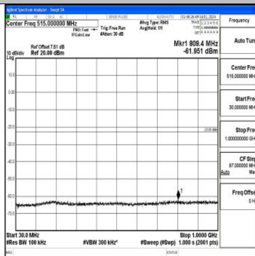
Band66_5MHz_16QAM_132647_1RB#0_30~1000_30~1000
