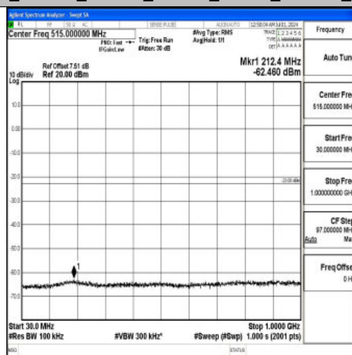
Band66_1.4MHz_16QAM_132665_1RB#0_30~1000_30~1000
