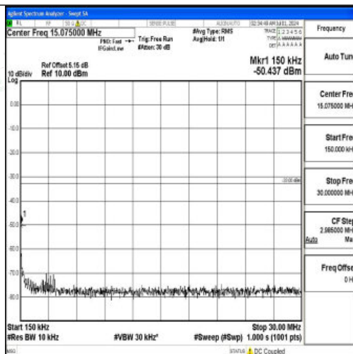
Band66_15MHz_QPSK_132047_1RB#0_0.15~30_0.15~30
