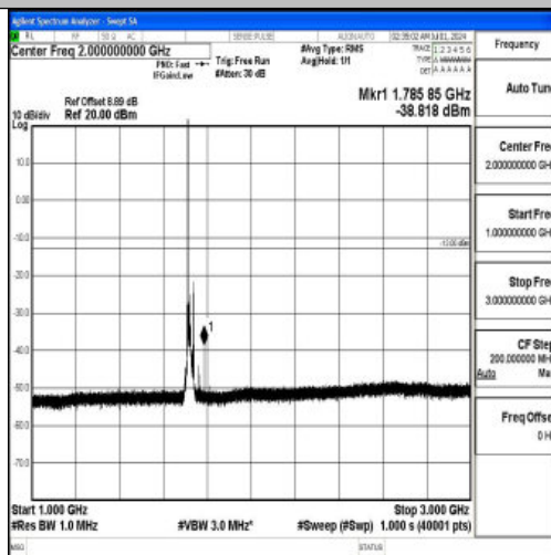
Band66_15MHz_QPSK_132047_1RB#0_1000~3000_1000~3000
