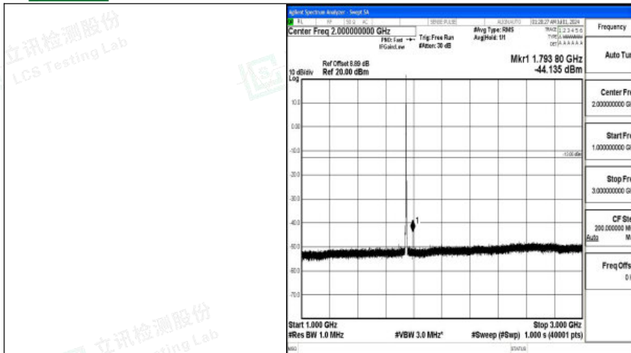
Band66_3MHz_QPSK_132322_1RB#0_1000~3000_1000~3000
