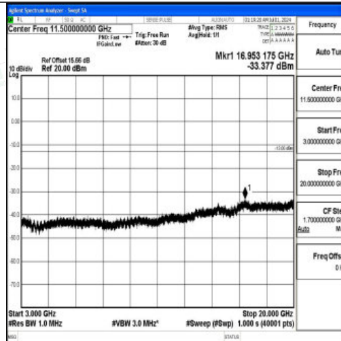
Band66_3MHz_QPSK_131987_1RB#0_3000~20000_3000~20000
