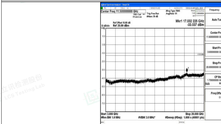
Band66_20MHz_16QAM_132572_1RB#0_3000~20000_3000~20000
