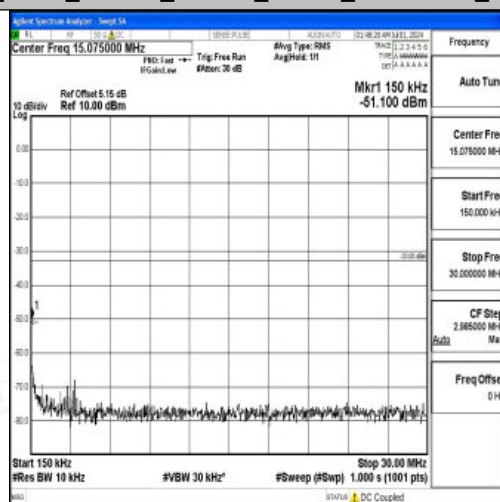
Band66_5MHz_16QAM_132647_1RB#0_0.15~30_0.15~30
