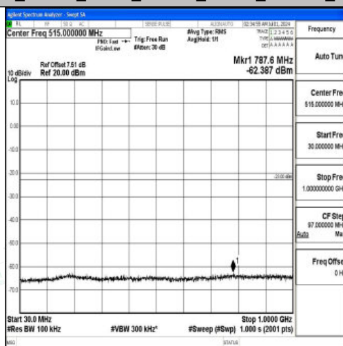
Band66_15MHz_QPSK_132047_1RB#0_30~1000_30~1000
