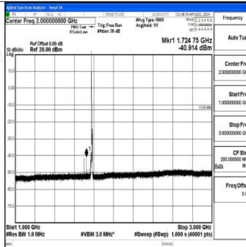
Band66_5MHz_16QAM_132647_1RB#0_1000~3000_1000~3000
