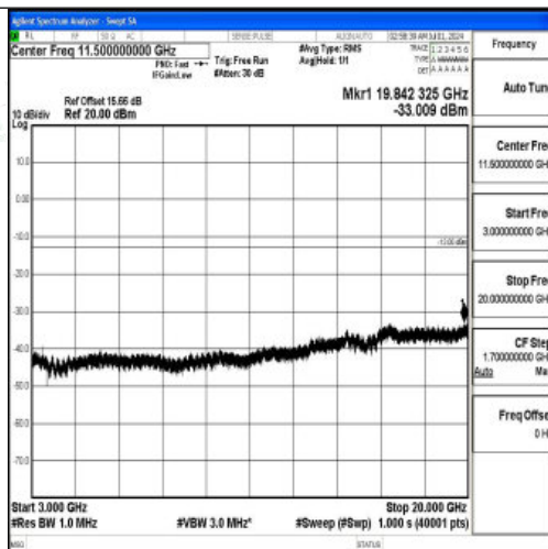
Band66_20MHz_QPSK_132072_1RB#0_3000~20000_3000~20000
