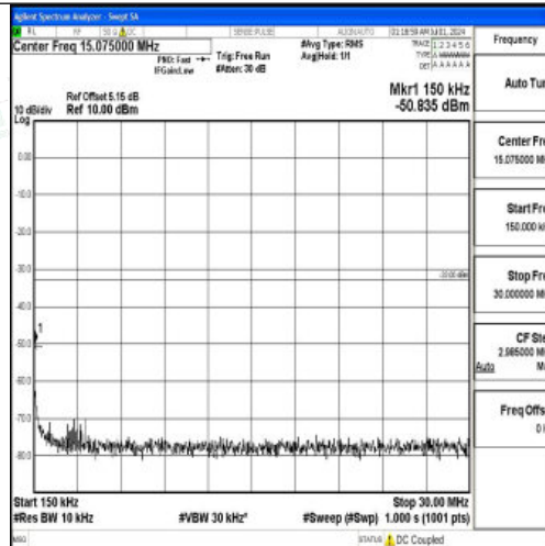
Band66_3MHz_QPSK_131987_1RB#0_0.15~30_0.15~30
