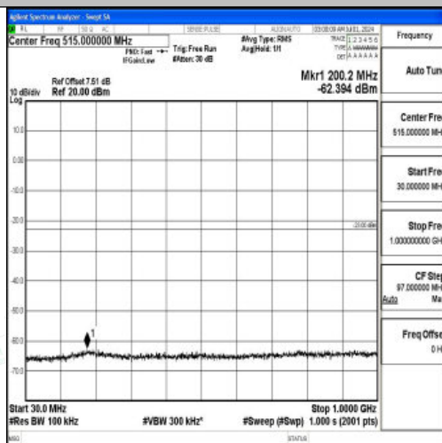
Band66_20MHz_16QAM_132322_1RB#0_30~1000_30~1000
