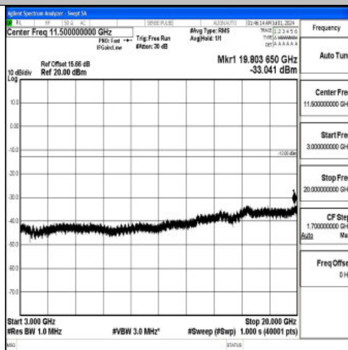
Band66_5MHz_16QAM_131997_1RB#0_3000~20000_3000~20000
