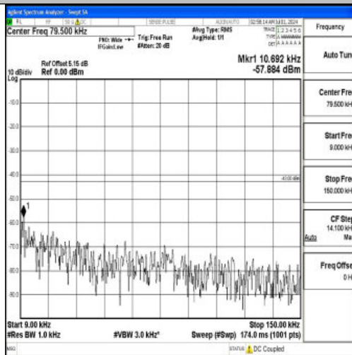
Band66_20MHz_QPSK_132072_1RB#0_0.009~0.15_0.009~0.15
