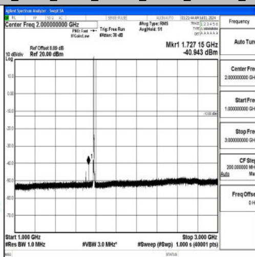
Band66_3MHz_QPSK_132657_1RB#0_1000~3000_1000~3000
