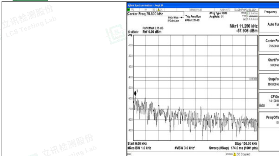
Band66_3MHz_QPSK_132322_1RB#0_0.009~0.15_0.009~0.15
