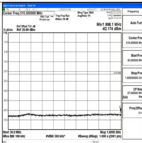
Band66_1.4MHz_QPSK_132665_1RB#0_30~1000_30~1000
