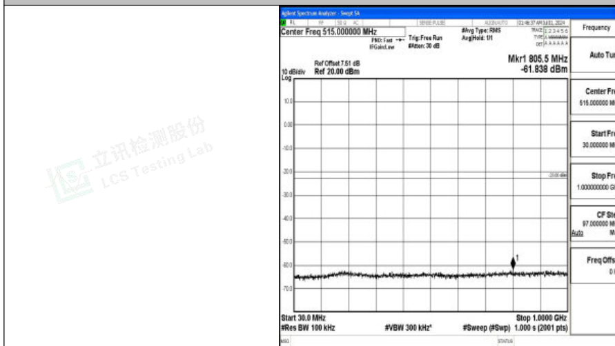
Band66_5MHz_QPSK_132322_1RB#0_30~1000_30~1000
