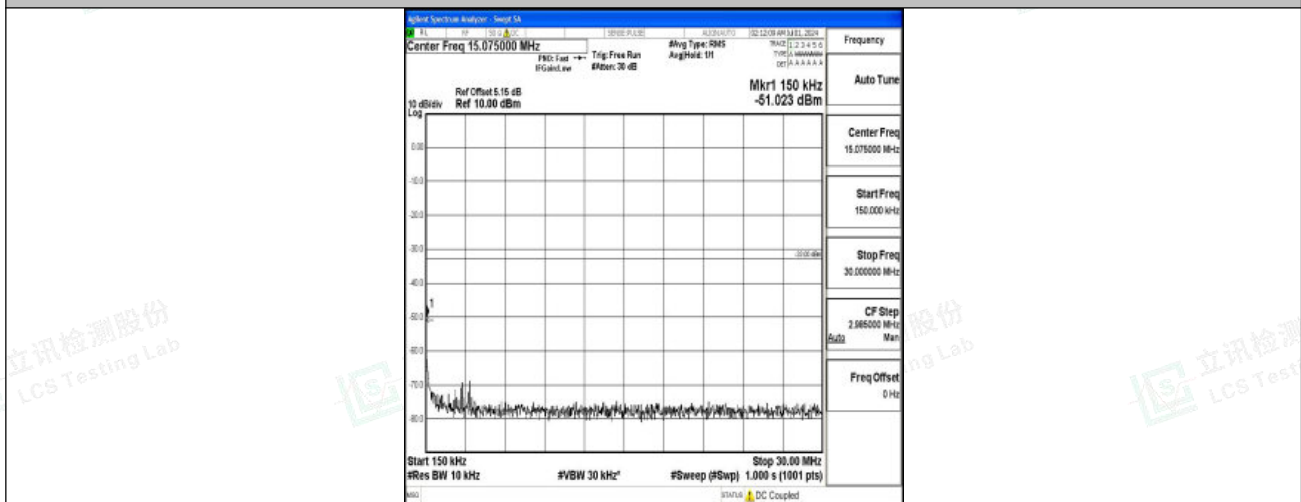
Band66_10MHz_QPSK_132322_1RB#0_0.15~30_0.15~30
