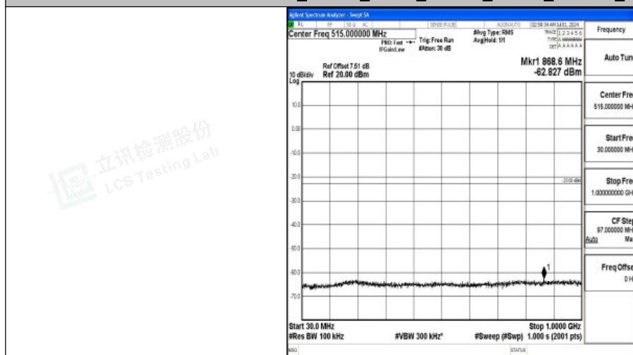
Band66_20MHz_QPSK_132322_1RB#0_30~1000_30~1000
