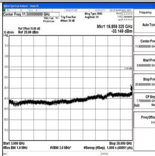
Band66_10MHz_QPSK_132622_1RB#0_3000~20000_3000~20000
