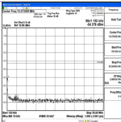
Band66_5MHz_16QAM_132322_1RB#0_0.15~30_0.15~30
