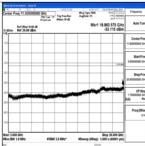
Band66_10MHz_16QAM_132322_1RB#0_3000~20000_3000~20000
