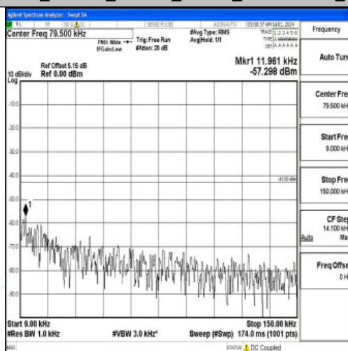
Band66_20MHz_QPSK_132572_1RB#0_0.009~0.15_0.009~0.15
