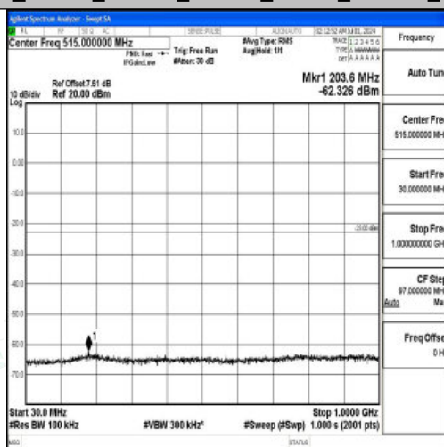
Band66_10MHz_16QAM_132322_1RB#0_30~1000_30~1000
