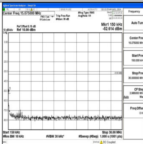
Band66_10MHz_QPSK_132622_1RB#0_0.15~30_0.15~30
