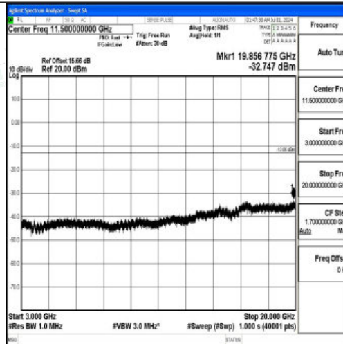
Band66_5MHz_16QAM_132322_1RB#0_3000~20000_3000~20000
