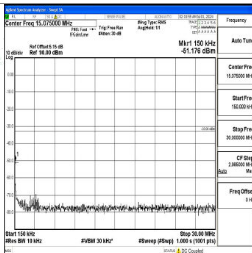
Band66_10MHz_QPSK_132022_1RB#0_0.15~30_0.15~30
