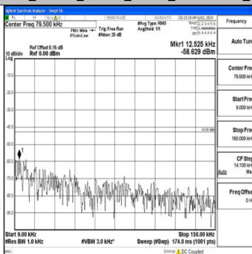
Band66_10MHz_QPSK_132622_1RB#0_0.009~0.15_0.009~0.15
