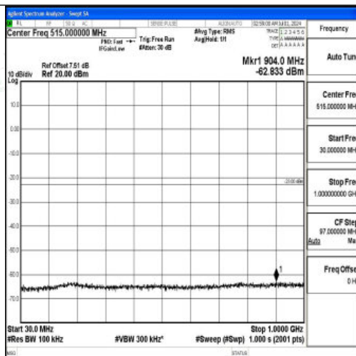
Band66_20MHz_16QAM_132072_1RB#0_30~1000_30~1000
