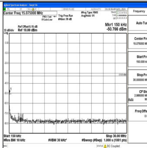
Band66_3MHz_16QAM_131987_1RB#0_0.15~30_0.15~30
