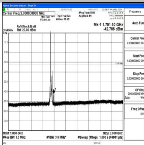
Band66_15MHz_16QAM_132322_1RB#0_1000~3000_1000~3000
