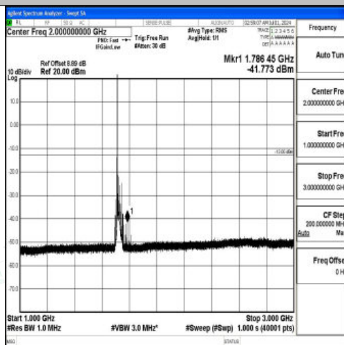
Band66_20MHz_16QAM_132072_1RB#0_1000~3000_1000~3000
