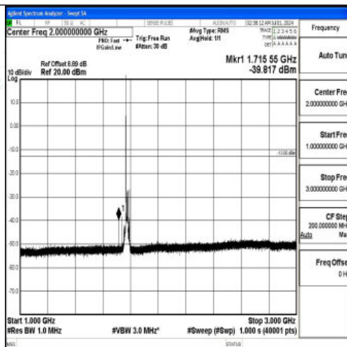
Band66_15MHz_16QAM_132597_1RB#0_1000~3000_1000~3000
