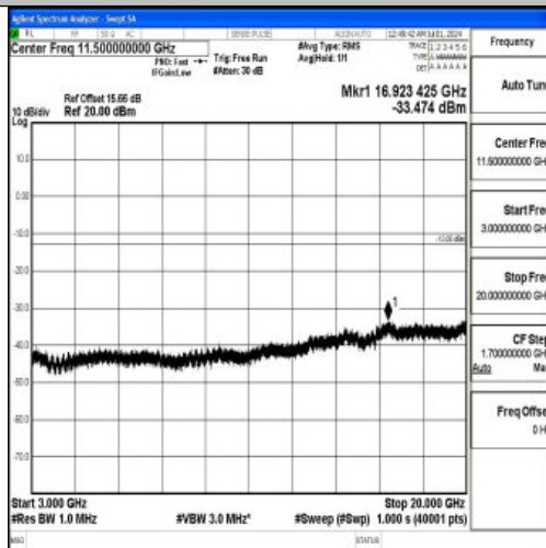
Band66_1.4MHz_QPSK_132665_1RB#0_3000~20000_3000~20000
