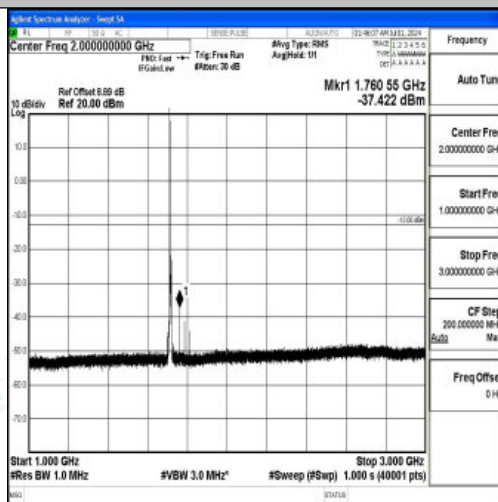
Band66_5MHz_16QAM_131997_1RB#0_1000~3000_1000~3000
