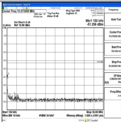
Band66_20MHz_16QAM_132072_1RB#0_0.15~30_0.15~30
