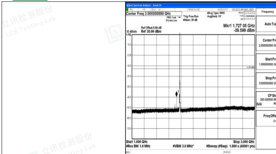
Band66_3MHz_16QAM_132657_1RB#0_1000~3000_1000~3000
