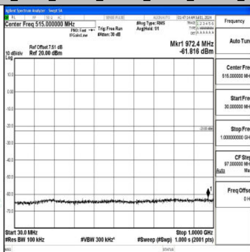
Band66_5MHz_16QAM_132322_1RB#0_30~1000_30~1000
