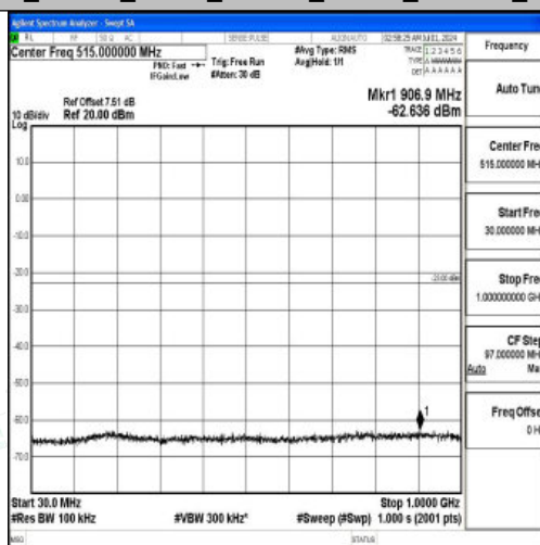
Band66_20MHz_QPSK_132072_1RB#0_30~1000_30~1000
