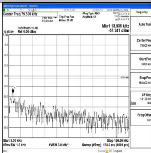
Band66_15MHz_QPSK_132047_1RB#0_0.009~0.15_0.009~0.15
