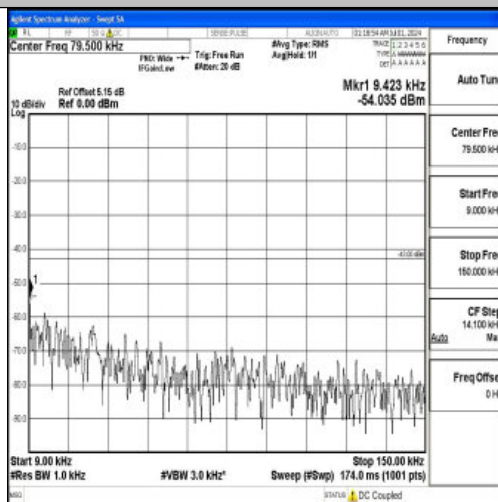
Band66_3MHz_QPSK_131987_1RB#0_0.009~0.15_0.009~0.15
