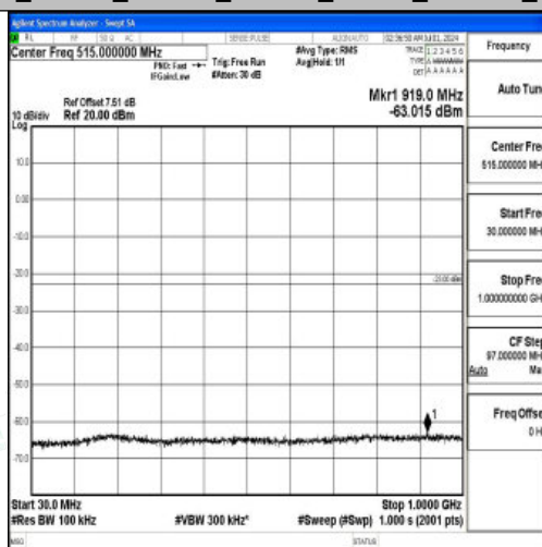
Band66_15MHz_16QAM_132322_1RB#0_30~1000_30~1000
