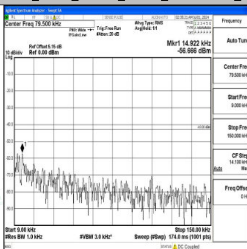
Band66_15MHz_16QAM_132047_1RB#0_0.009~0.15_0.009~0.15
