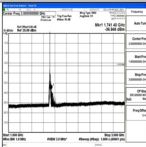
Band66_10MHz_16QAM_132022_1RB#0_1000~3000_1000~3000
