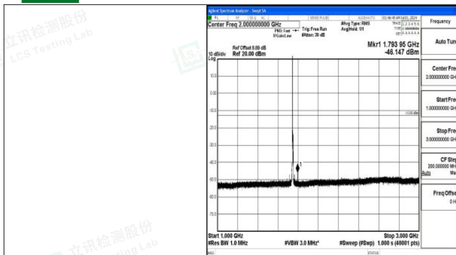
Band66_5MHz_QPSK_132322_1RB#0_1000~3000_1000~3000
