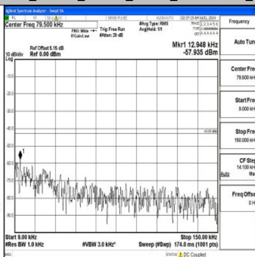
Band66_15MHz_QPSK_132597_1RB#0_0.009~0.15_0.009~0.15
