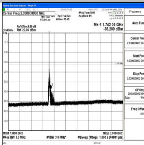
Band66_10MHz_QPSK_132022_1RB#0_1000~3000_1000~3000
