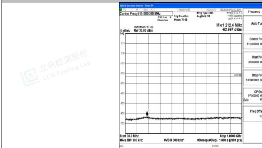
Band66_3MHz_QPSK_132322_1RB#0_30~1000_30~1000
