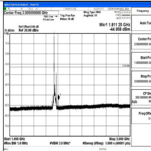
Band66_20MHz_QPSK_132322_1RB#0_1000~3000_1000~3000
