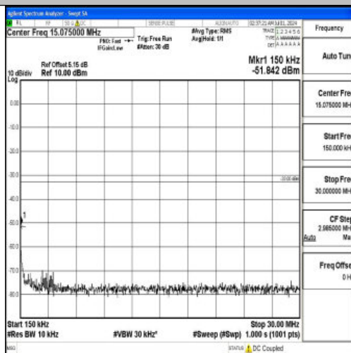
Band66_15MHz_QPSK_132597_1RB#0_0.15~30_0.15~30
