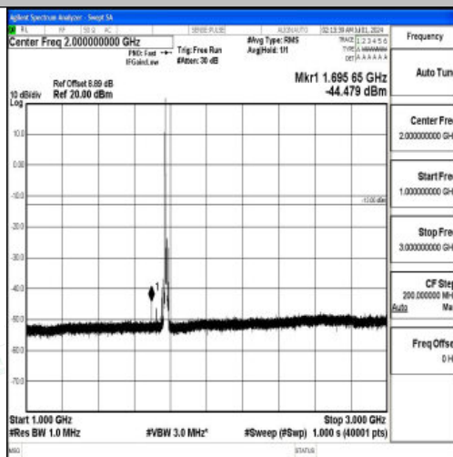
Band66_10MHz_QPSK_132622_1RB#0_1000~3000_1000~3000
