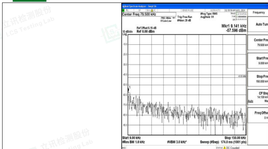
Band66_15MHz_QPSK_132322_1RB#0_0.009~0.15_0.009~0.15
