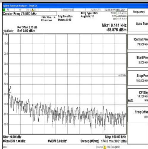
Band66_15MHz_16QAM_132322_1RB#0_0.009~0.15_0.009~0.15
