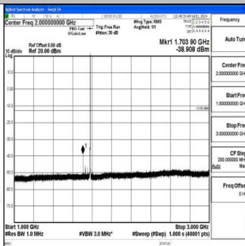
Band66_1.4MHz_QPSK_132665_1RB#0_1000~3000_1000~3000
