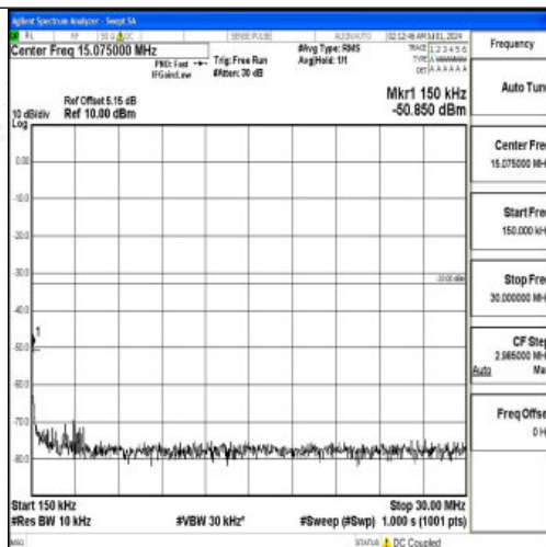
Band66_10MHz_16QAM_132322_1RB#0_0.15~30_0.15~30
