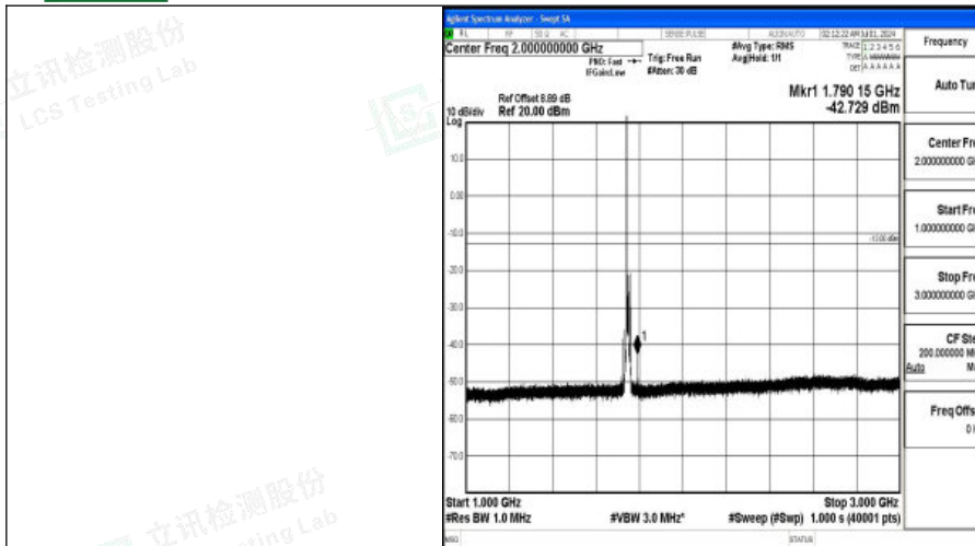
Band66_10MHz_QPSK_132322_1RB#0_1000~3000_1000~3000
