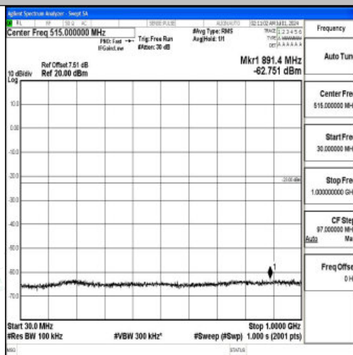
Band66_10MHz_QPSK_132022_1RB#0_30~1000_30~1000
