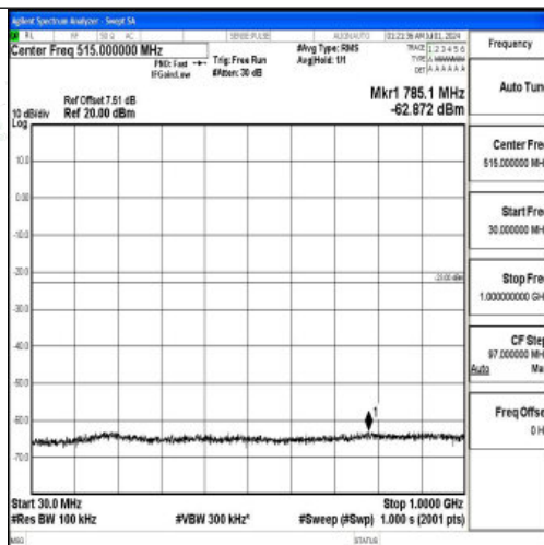
Band66_3MHz_QPSK_132657_1RB#0_30~1000_30~1000
