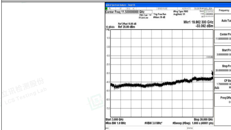
Band66_3MHz_QPSK_132322_1RB#0_3000~20000_3000~20000
