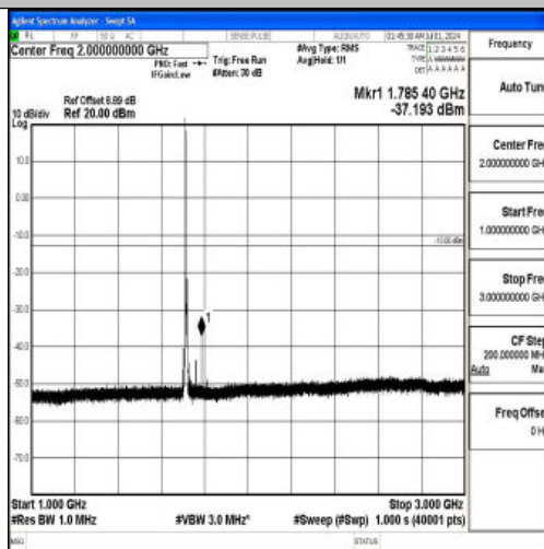
Band66_5MHz_QPSK_131997_1RB#0_1000~3000_1000~3000
