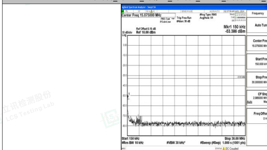
Band66_15MHz_16QAM_132597_1RB#0_0.15~30_0.15~30
