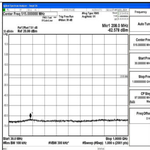
Band66_10MHz_16QAM_132022_1RB#0_30~1000_30~1000
