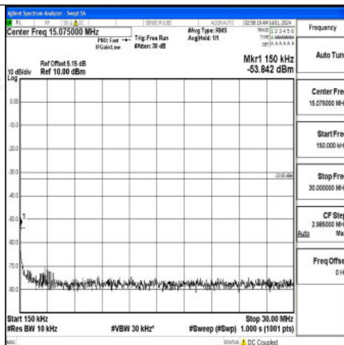
Band66_20MHz_QPSK_132072_1RB#0_0.15~30_0.15~30
