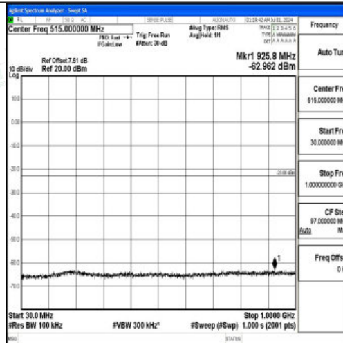
Band66_3MHz_16QAM_131987_1RB#0_30~1000_30~1000
