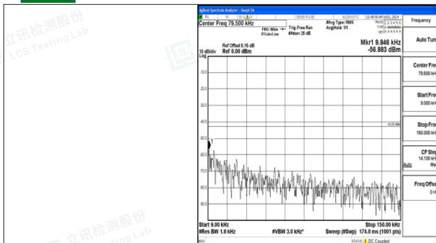
Band66_1.4MHz_16QAM_132665_1RB#0_0.009~0.15_0.009~0.15
