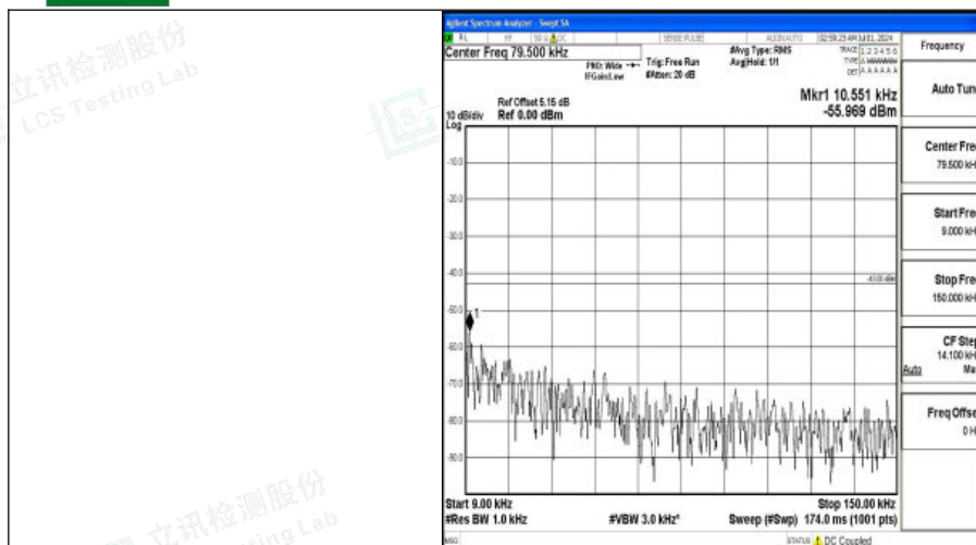
Band66_20MHz_QPSK_132322_1RB#0_0.009~0.15_0.009~0.15
