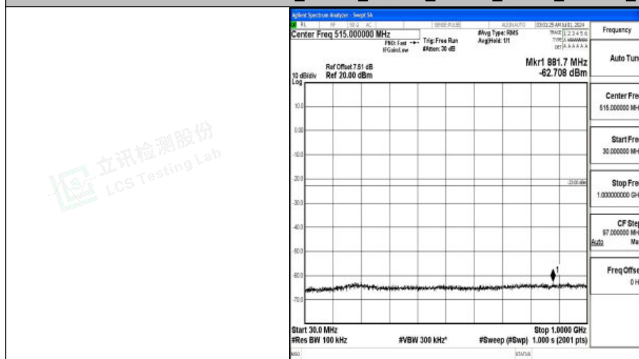
Band66_20MHz_16QAM_132572_1RB#0_30~1000_30~1000
