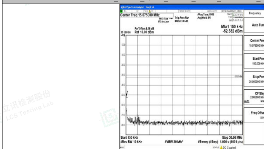
Band66_15MHz_QPSK_132322_1RB#0_0.15~30_0.15~30
