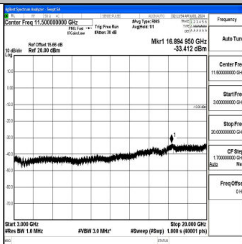
Band66_10MHz_16QAM_132022_1RB#0_3000~20000_3000~20000
