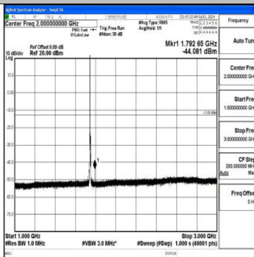
Band66_5MHz_16QAM_132322_1RB#0_1000~3000_1000~3000
