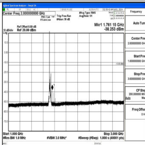
Band66_15MHz_16QAM_132047_1RB#0_1000~3000_1000~3000
