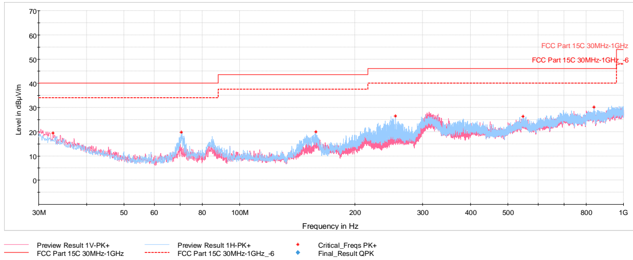
Plot 7-32. Radiated Spurious Emissions Below 1GHz (2Mbps – Ch.19, Pol. H & V, with Laptop)
