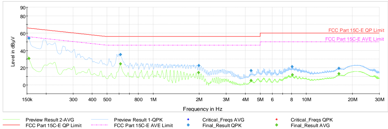
Plot 7-34. AC Line Conducted Plot with Bluetooth LE (N, 2Mbps – Ch.0, with Laptop)
