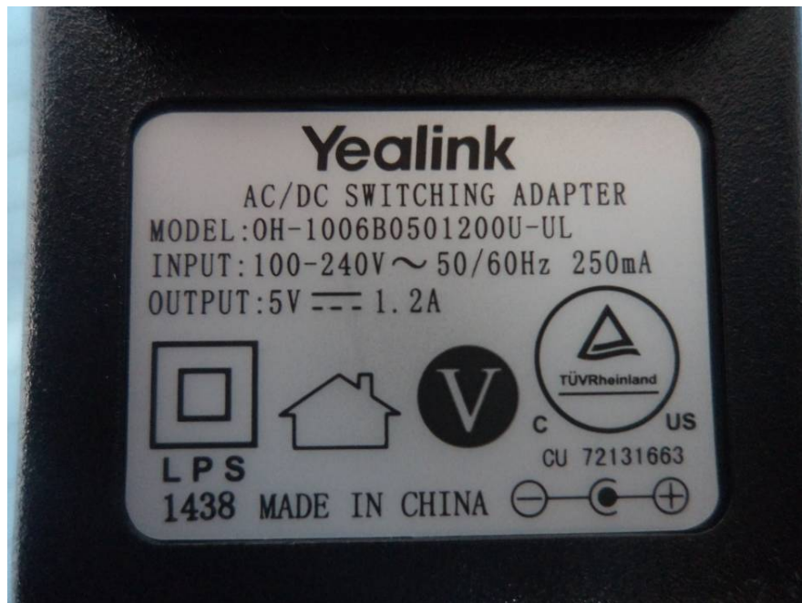
EUT – Adapter 2 Label View
