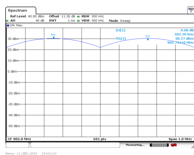
Channel Separation Plot on Channel 48 - 49
