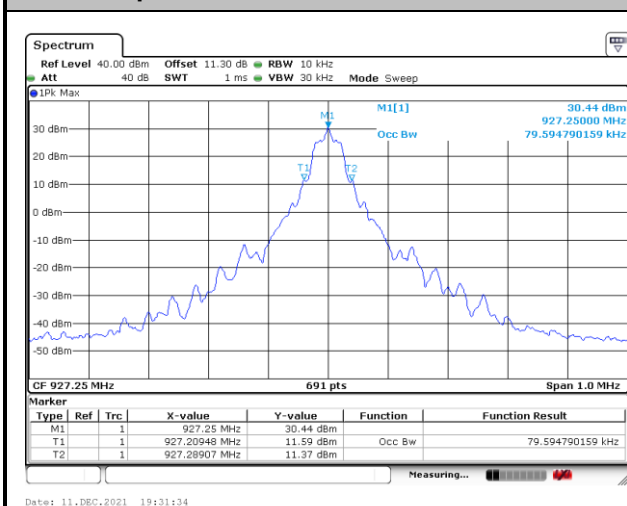
99% Occupied Bandwidth Plot on Channel 49
