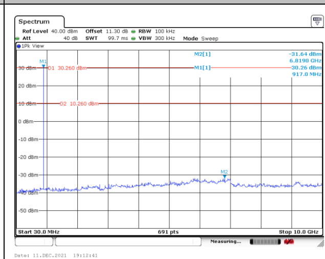
CSE Plot on Channel 24 between 30MHz ~ 10 GHz
