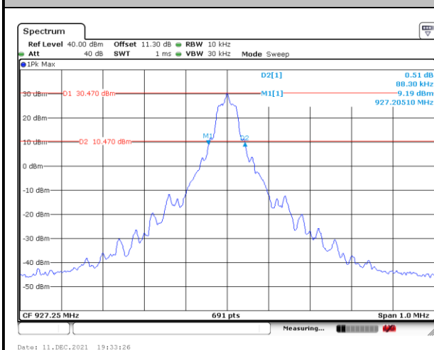
20 dB Bandwidth Plot on Channel 49
