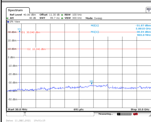
CSE Plot on Channel 00 between 30MHz ~ 10 GHz
