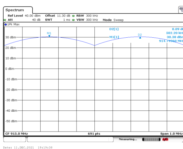
Channel Separation Plot on Channel 24 - 25
