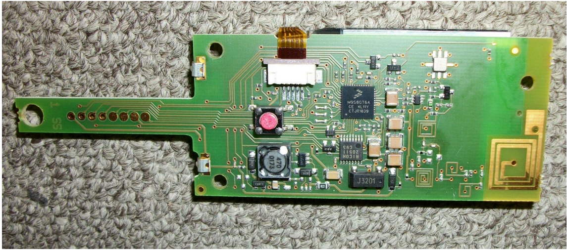
Figure 7.5 Component Side
