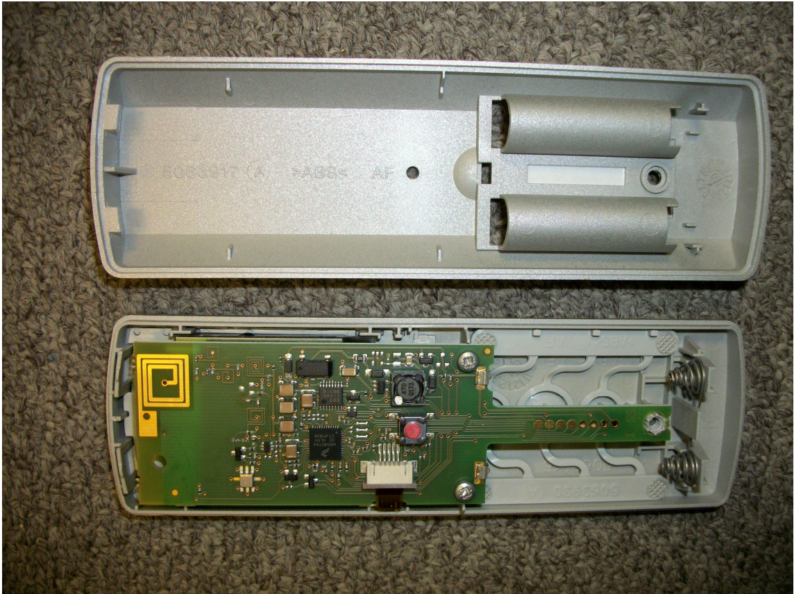
Figure 7.4 Inside View
