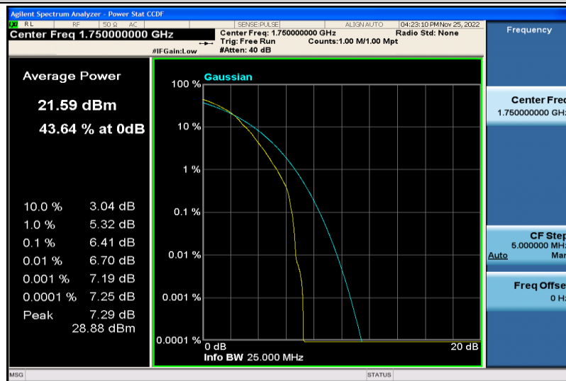
Band4-10MHz-64QAM-20350-1RB#0
