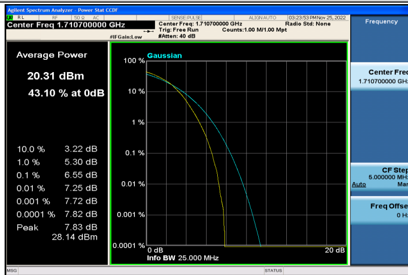
Band4-1.4MHz-64QAM-19957-6RB#0
