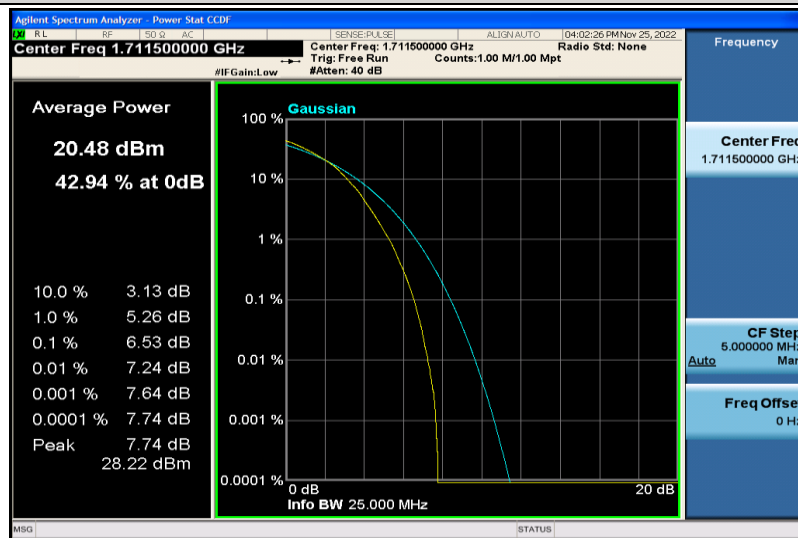
Band4-3MHz-64QAM-19965-15RB#0
