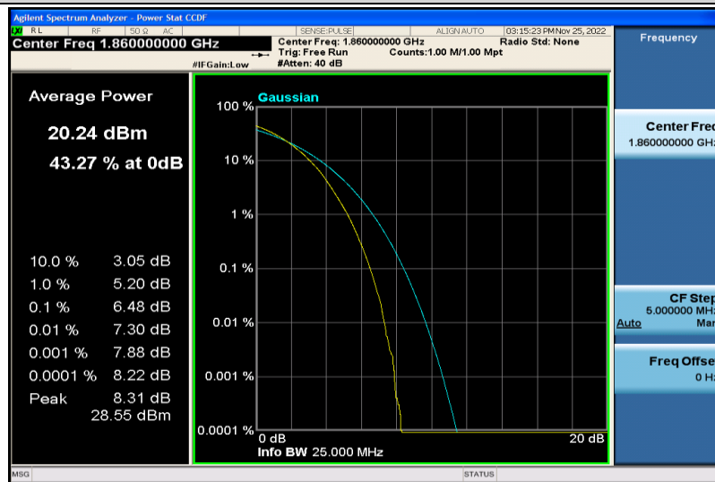
Band2-20MHz-64QAM-18700-100RB#0
