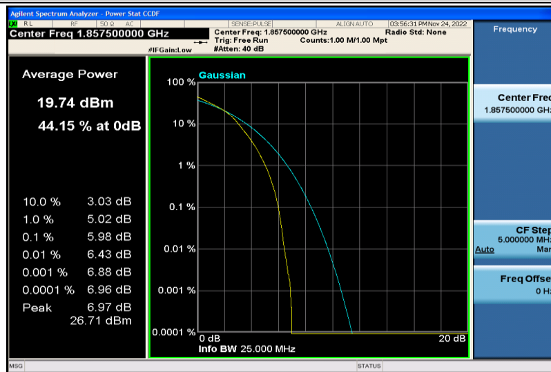
Band2-15MHz-16QAM-18675-5RB#0
