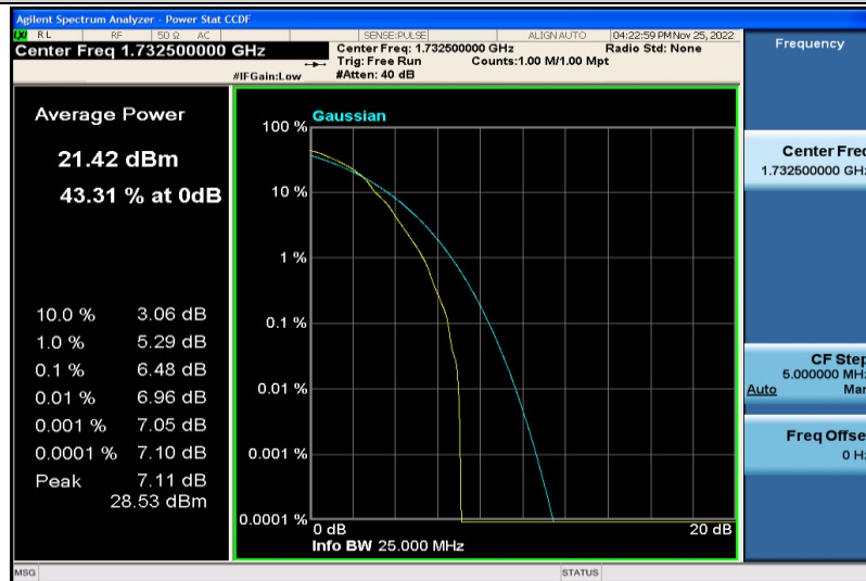
Band4-10MHz-64QAM-20175-1RB#0
