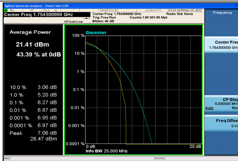
Band4-1.4MHz-64QAM-20393-1RB#0
