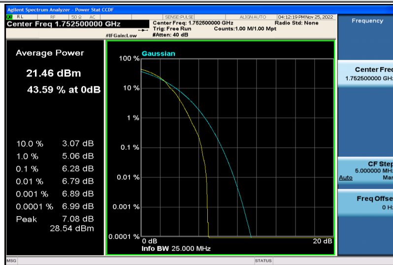
Band4-5MHz-64QAM-20375-1RB#0
