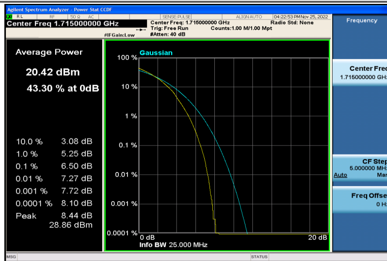
Band4-10MHz-64QAM-20000-50RB#0
