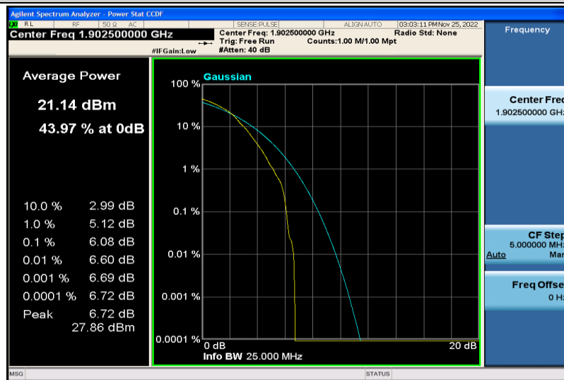
Band2-15MHz-64QAM-19125-1RB#0
