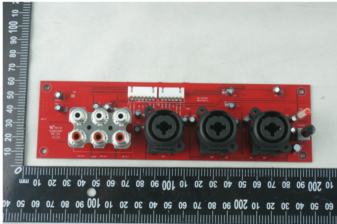
EUT MAIN BOARD FRONT VIEW 4
