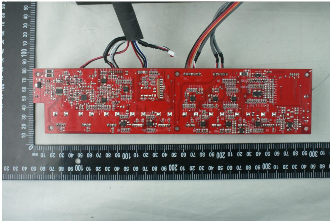
EUT MAIN BOARD BACK VIEW 1
