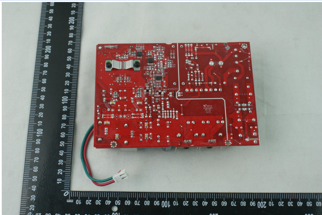
EEUT MAIN BOARD BACK VIEW 2
