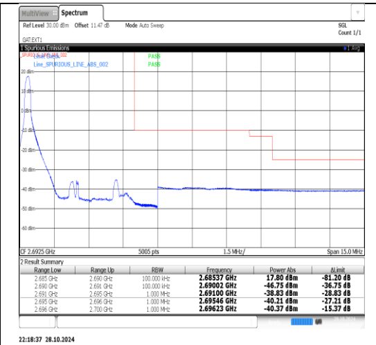
Band41-5MHz-16QAM-41565-1RB#24-PASS
