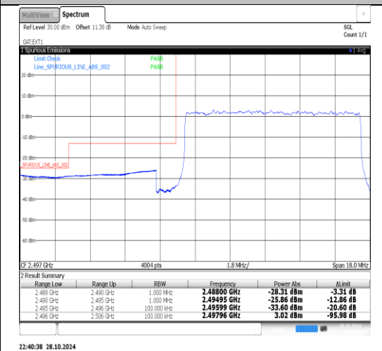
Band41-10MHz-QPSK-41540-1RB#0-PASS
