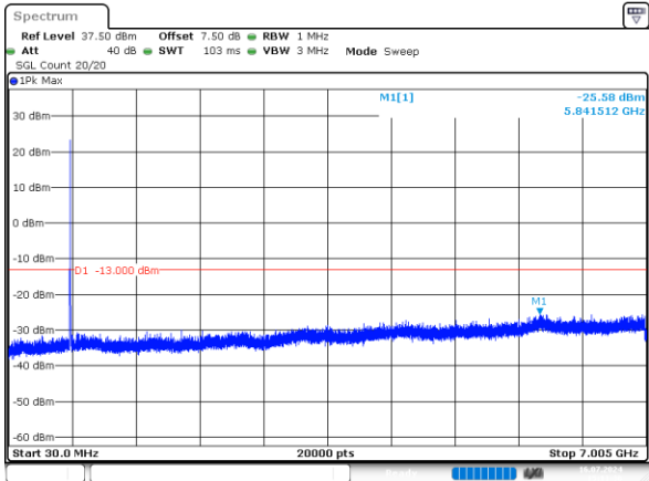
3MHz_Low_QPSK_15@0 -25.58dBm
