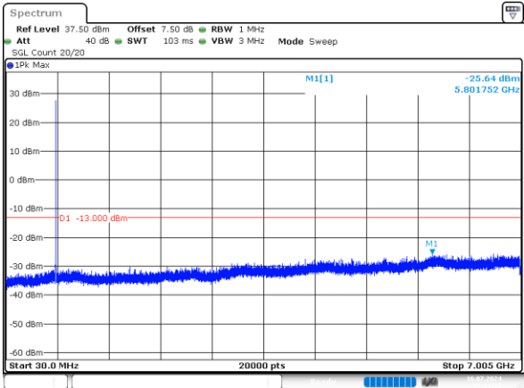
3MHz_Low_QPSK_1@0 -25.64dBm
