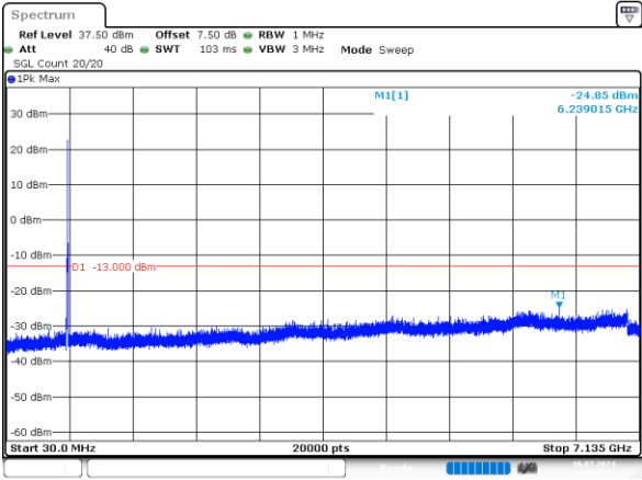
5MHz_High_QPSK_25@0 -24.85dBm
