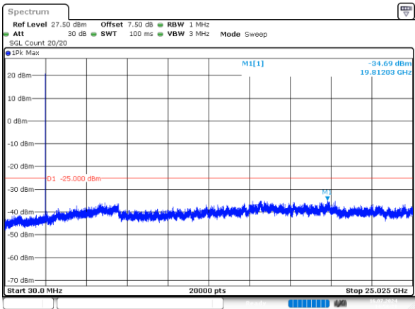
5MHz_Low_QPSK_1@0 -34.69dBm
