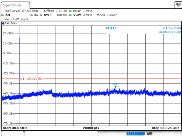
5MHz_Low_QPSK_25@0 -34.62dBm
