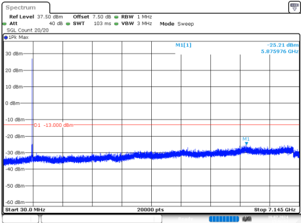
3MHz_High_QPSK_1@0 -25.21dBm
