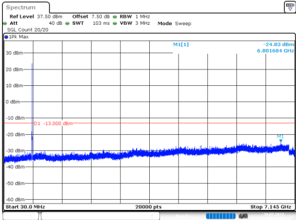
3MHz_High_QPSK_15@0 -24.83dBm
