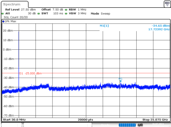
15MHz_Low_QPSK_1@0 -34.65dBm
