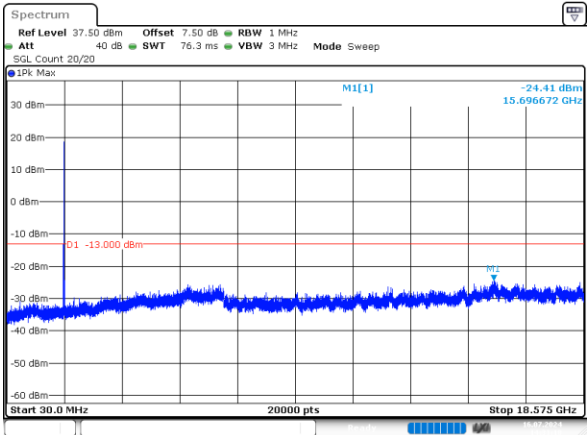
15MHz_Low_QPSK_1@0 -24.41dBm
