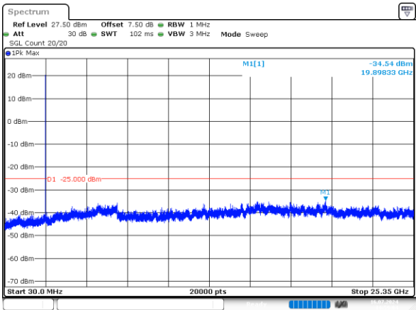
5MHz_Middle_QPSK_1@0 -34.54dBm
