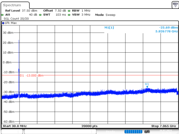
5MHz_Low_QPSK_25@0 -25.69dBm
