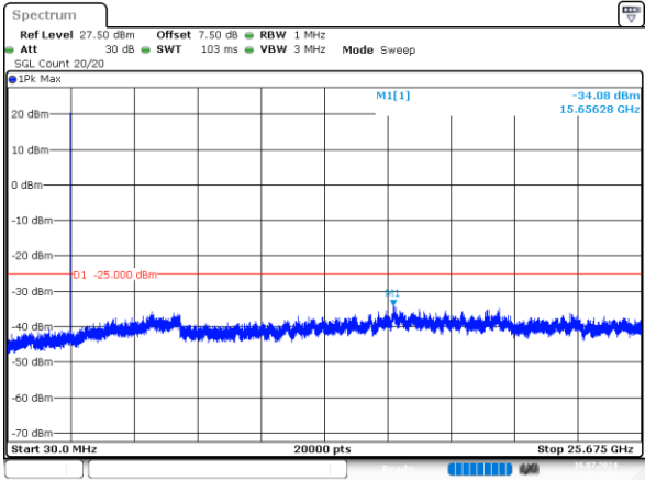
5MHz_High_QPSK_1@0 -34.08dBm
