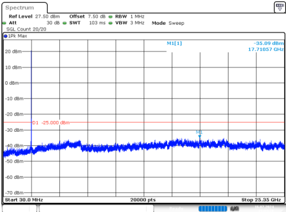
15MHz_Middle_QPSK_1@0 -35.09dBm
