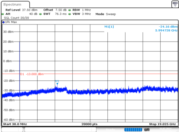
15MHz_High_QPSK_1@0 -24.16dBm
