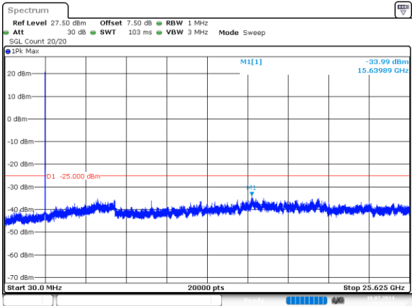
15MHz_High_QPSK_1@0 -33.99dBm
