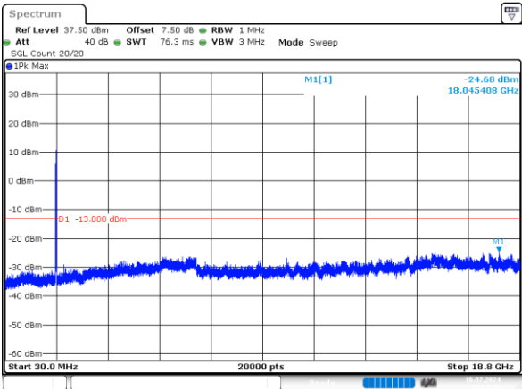
20MHz_Middle_QPSK_100@0 -24.68dBm
