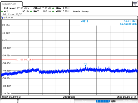
5MHz_Middle_QPSK_25@0 -34.41dBm
