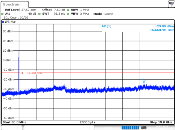
20MHz_High_QPSK_100@0 -23.99dBm
