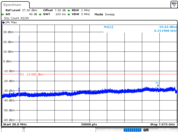
3MHz_Middle_QPSK_1@0 -25.65dBm
