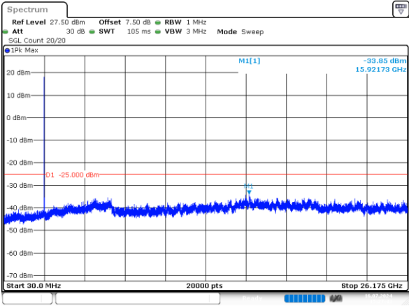
5MHz_High_QPSK_25@0 -33.85dBm
