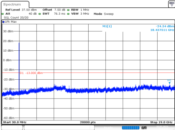
20MHz_High_QPSK_1@0 -24.54dBm
