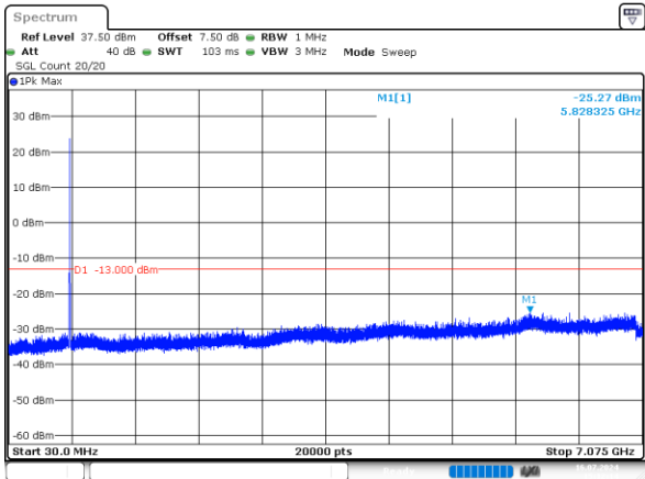
3MHz_Middle_QPSK_15@0 -25.27dBm
