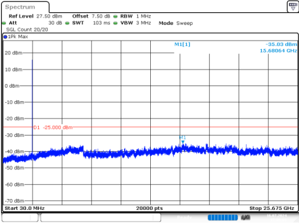
5MHz_High_QPSK_25@0 -35.03dBm
