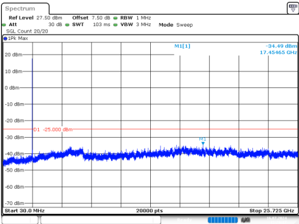
5MHz_Low_QPSK_25@0 -34.49dBm
