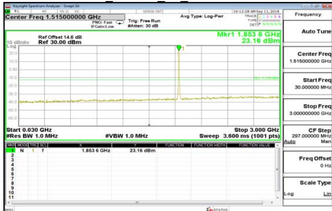
30MHz~3GHz_HSUPA_B2_LowCH9262-1852.4
