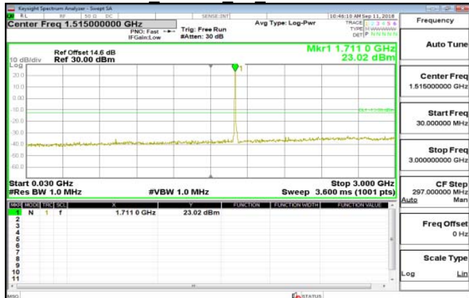
30MHz~3GHz_HSUPA_B4_LowCH1312-1712.4
