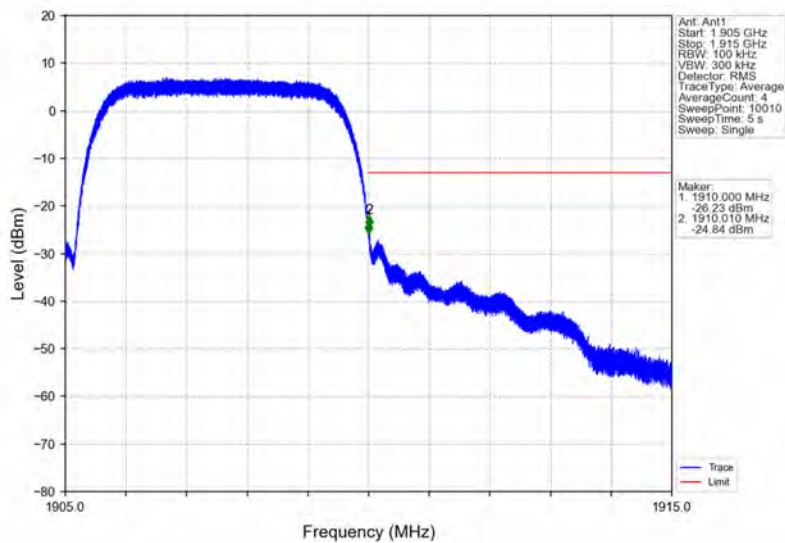
Band2_HSUPA_HCH_1907.6MHz_Subtest 1_NTNV
