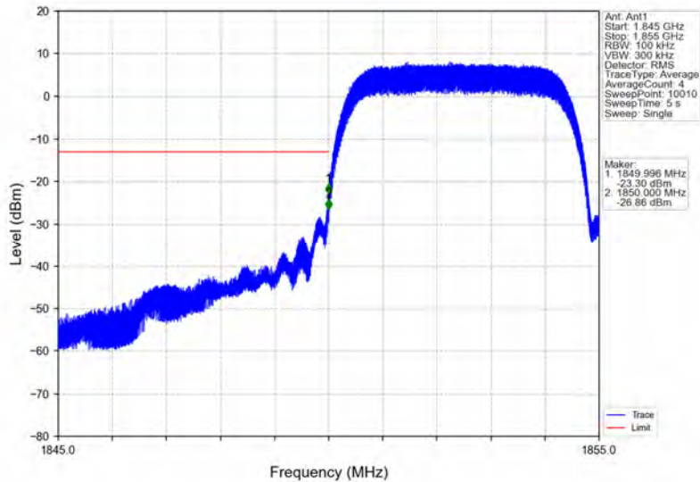
Band2_HSUPA_LCH_1852.4MHz_Subtest 1_NTNV
