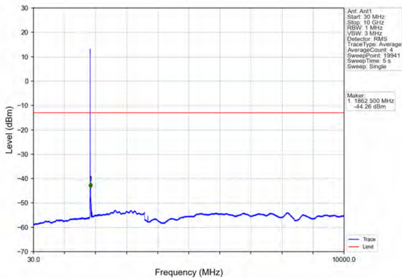
Band2_HSUPA_LCH_1852.4MHz_Subtest 1_NTNV
