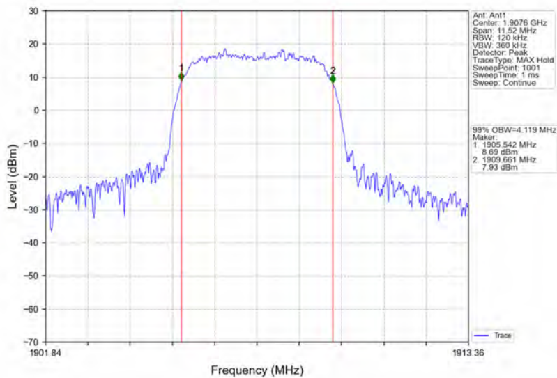
Band2_HSDPA_HCH_1907.6MHz_Subtest 1_NTNV
