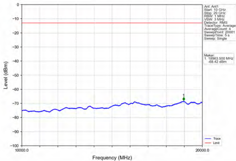
Band2_HSUPA_HCH_1907.6MHz_Subtest 1_NTNV
