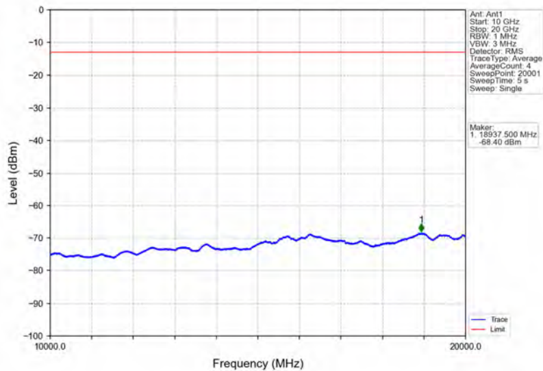
Band2_RMC_MCH_1880MHz_12.2kbps RMC_NTNV
