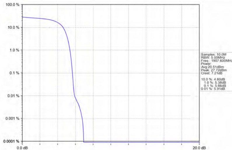
Band2_HSDPA_HCH_1907.6MHz_Subtest 1_NTNV
