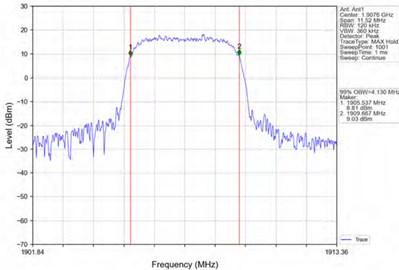
Band2_HSUPA_HCH_1907.6MHz_Subtest 1_NTNV
