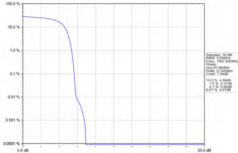
Band2_HSUPA_HCH_1907.6MHz_Subtest 1_NTNV
