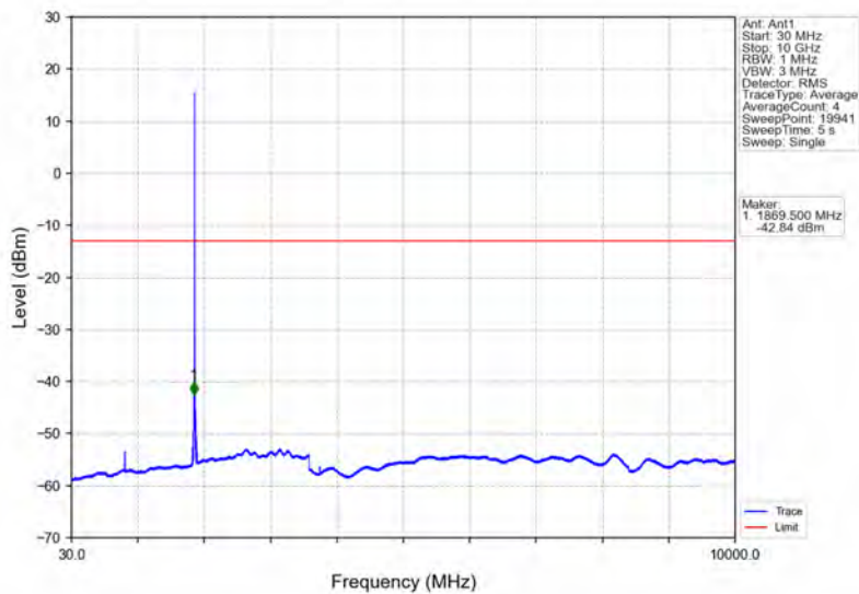
Band2_HSDPA_MCH_1880MHz_Subtest 1_NTNV
