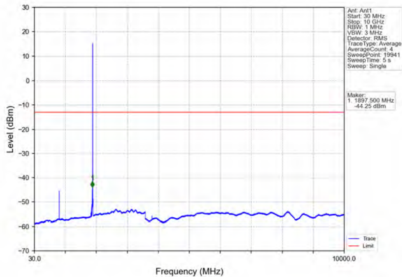
Band2_HSUPA_HCH_1907.6MHz_Subtest 1_NTNV
