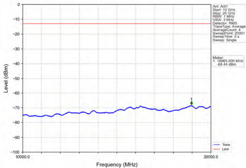
Band2_RMC_HCH_1907.6MHz_12.2kbps RMC_NTNV
