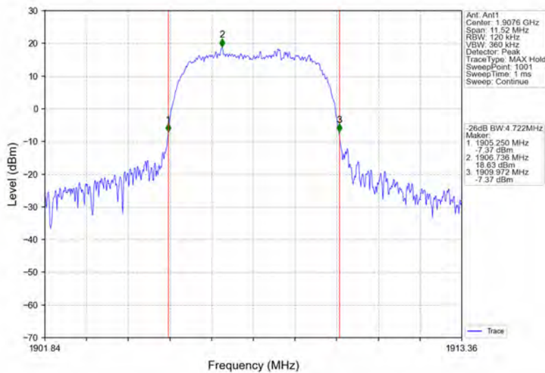
Band2_HSDPA_HCH_1907.6MHz_Subtest 1_NTNV
