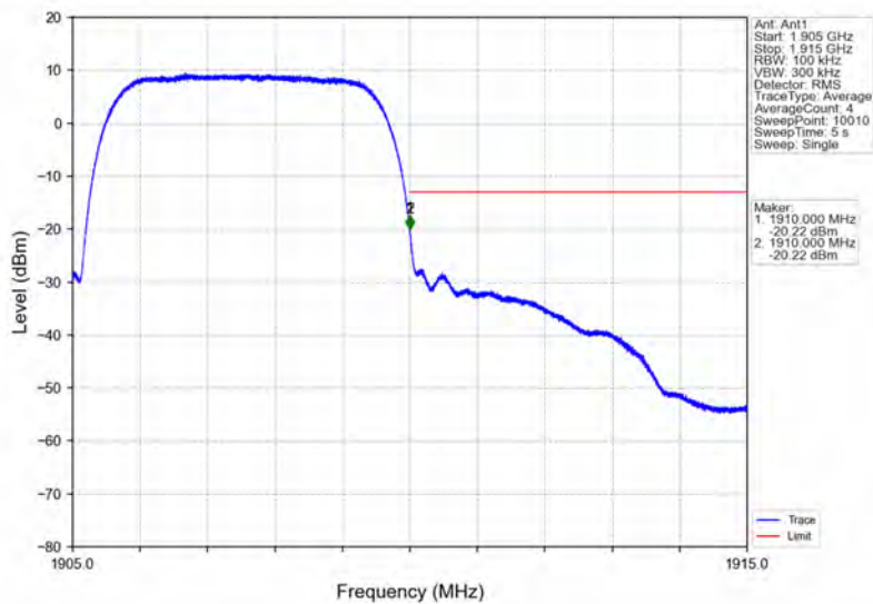
Band2_RMC_HCH_1907.6MHz_12.2kbps RMC_NTNV
