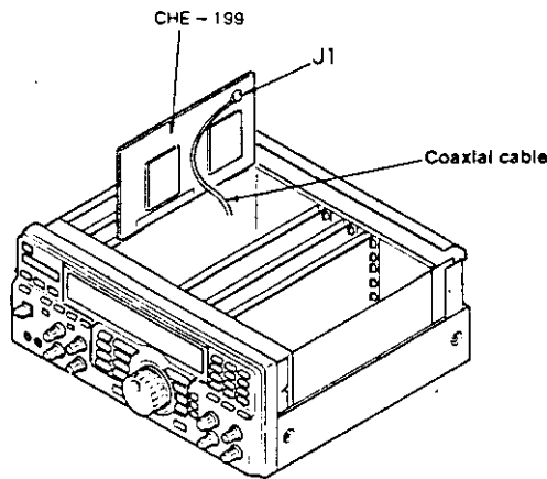
Figure 7-2 Mounting the Wideband Converter Unit
