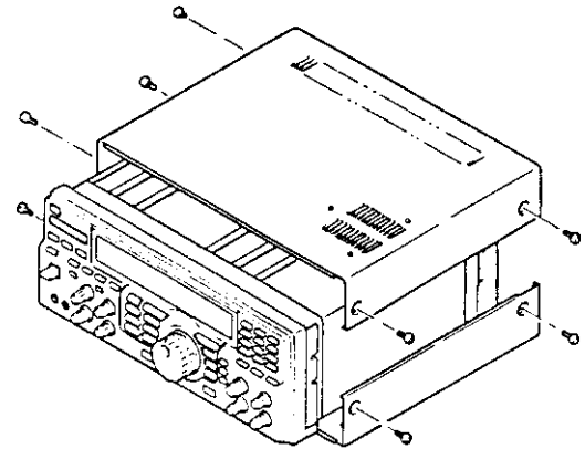
Figure 7-3 How to Remove the Covers
