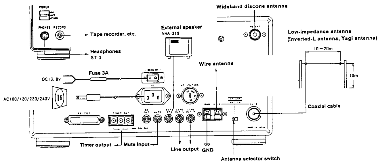
Figure 3-6 How to Connect the External Terminals
