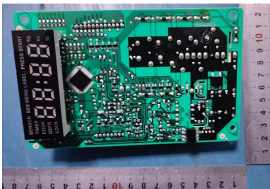
Original Mother board -bottom
