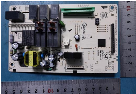
Original Mother board-top view
