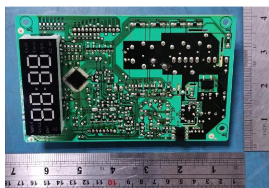
New Mother board -bottom
