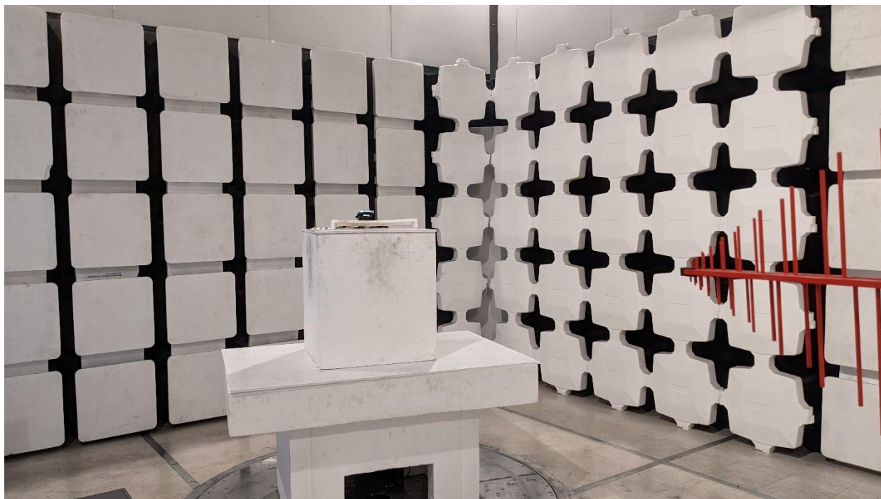
Emissions 30MHz to 1GHz
