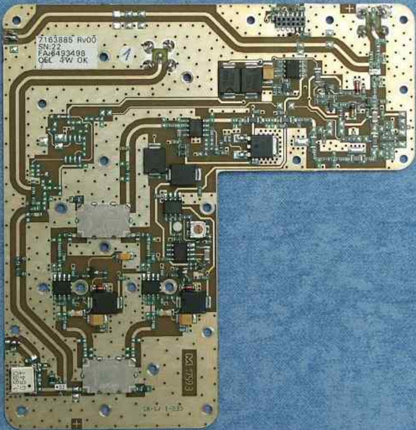
Final Amplifier - Uplink - Top
