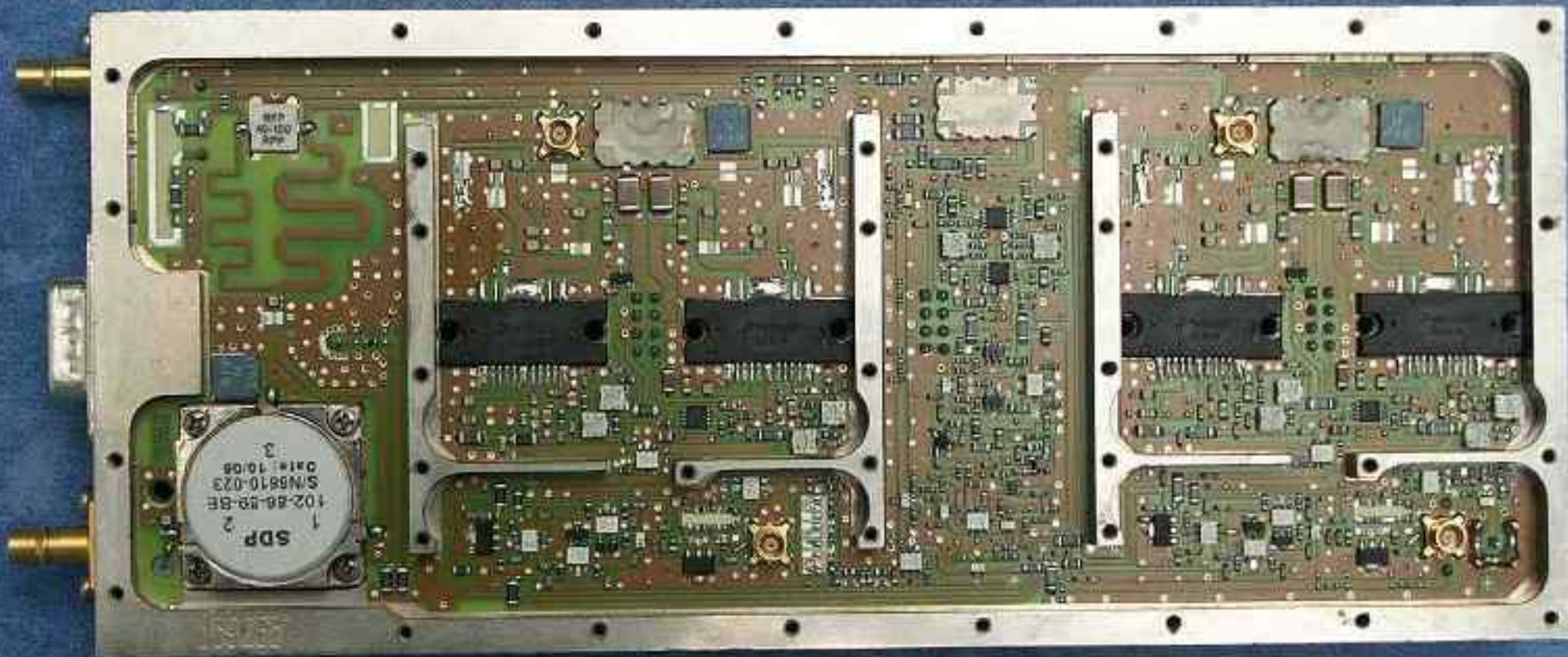
Final Amplifier board - Downlink - Top
