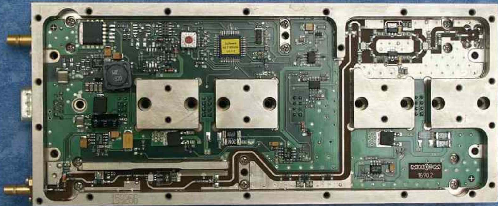
Final Amplifier board - Downlink - Bottom
