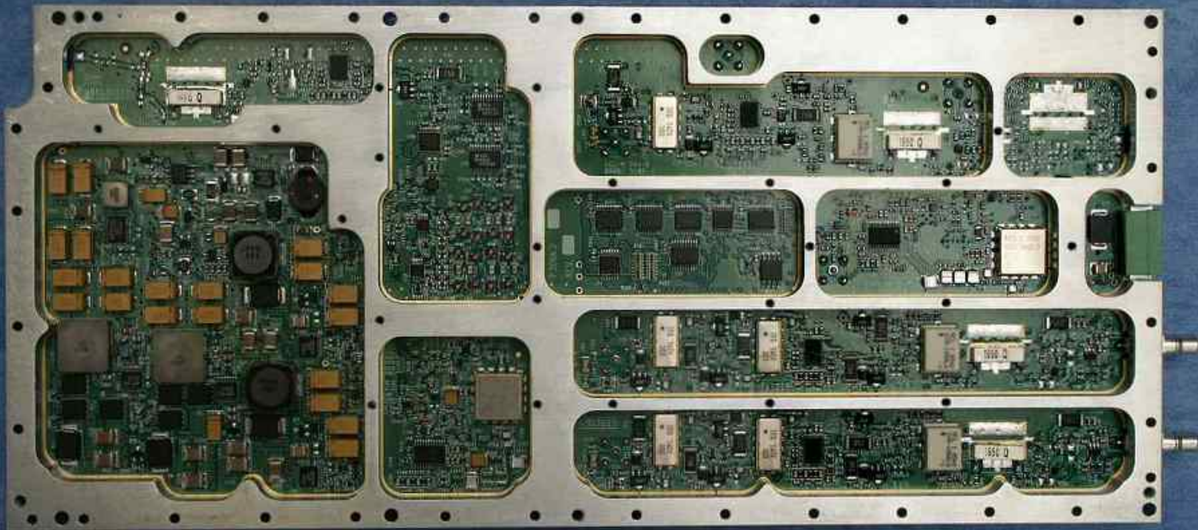
RF Channel Module - Uplink - Top
