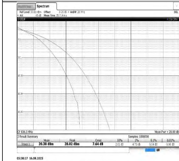
Band5-3MHz-QPSK-20525-15RB#0
