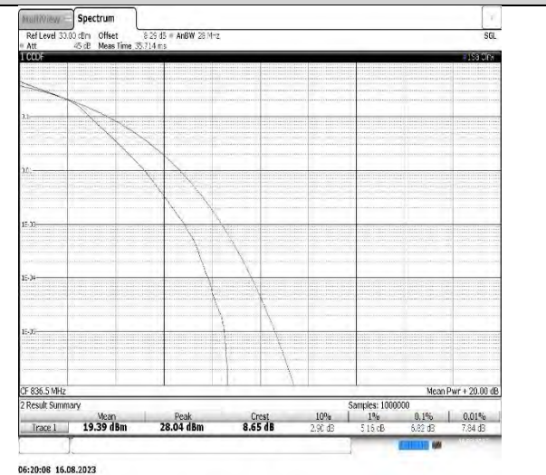
Band5-5MHz-16QAM-20525-25RB#0
