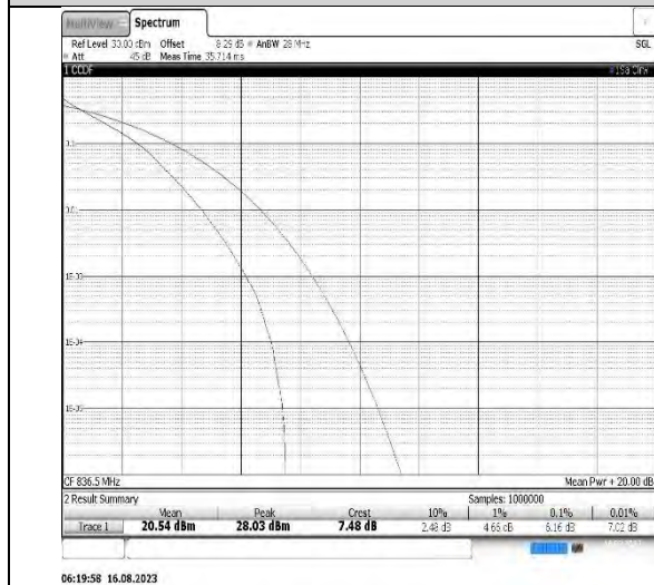
Band5-5MHz-QPSK-20525-25RB#0
