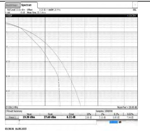
Band5-3MHz-16QAM-20525-15RB#0
